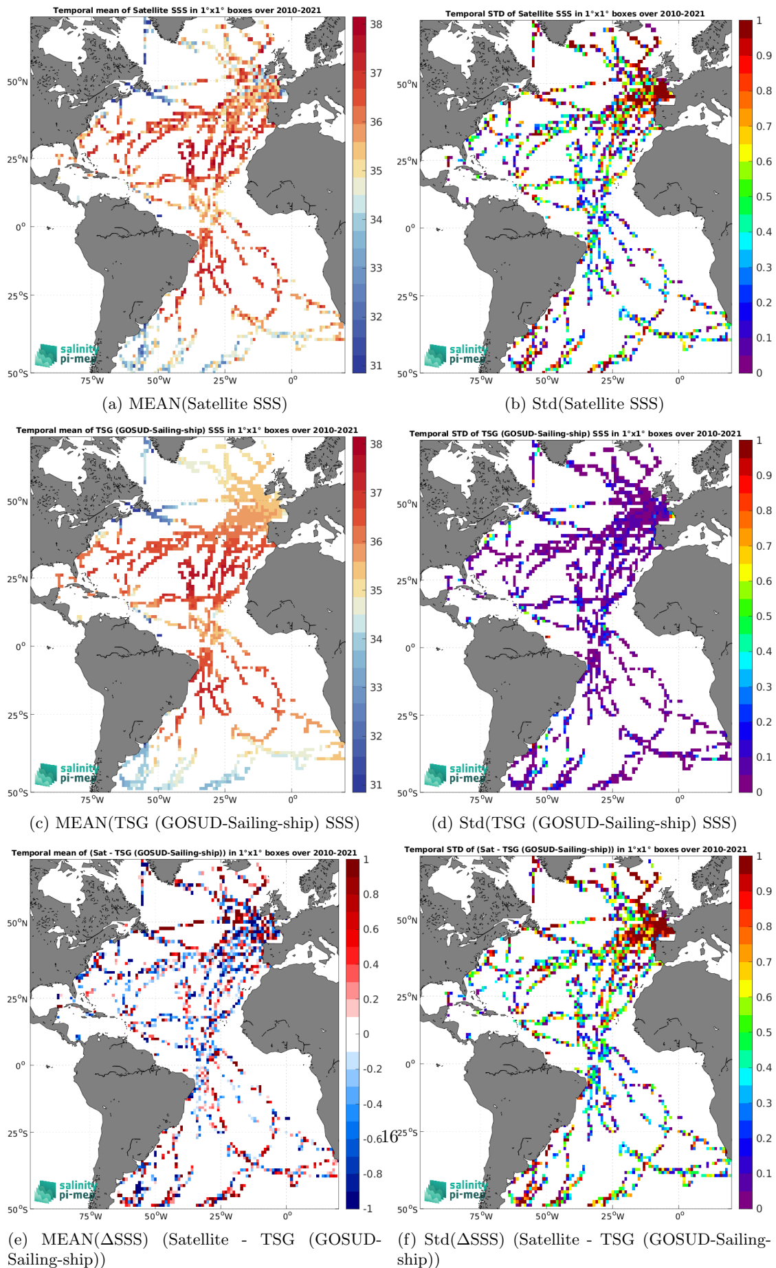
Figure 6: Temporal mean (left) and Std (right) of SSS from SMOS SSS L2Q v331 - With FLAG (CMEMS-CATDS-CPDC) (top), TSG (GOSUD-Sailing-ship) (middle), and of \Delta SSS (Satellite - TSG (GOSUD-Sailing-ship)). Only match-up pairs are used to generate these maps.
