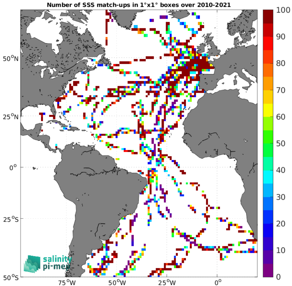
Figure 4: Number of SSS match-ups between TSG (GOSUD-Sailing-ship) SSS and the SMOS SSS L2Q v331 - With FLAG (CMEMS-CATDS-CPDC) SSS product for the Atlantic Ocean Pi-MEP region over 1^\circ \times 1^\circ boxes and for the full satellite product period.
