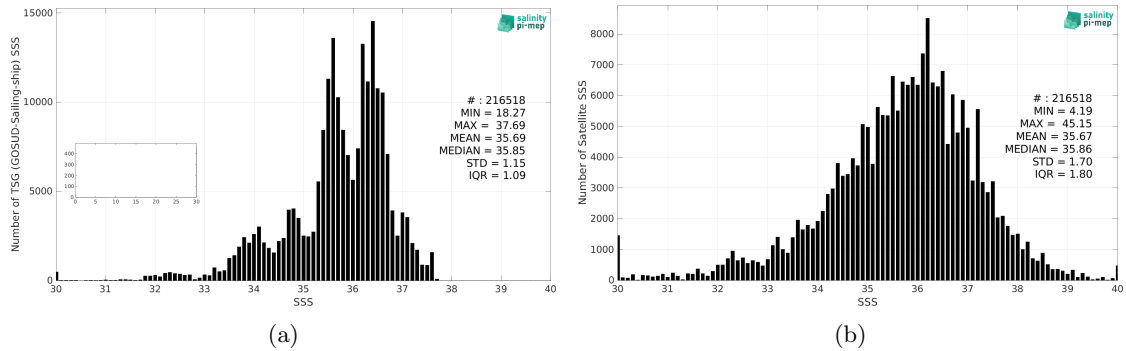
Figure 2: Histograms of SSS from TSG (GOSUD-Sailing-ship) (a) and SMOS SSS L2Q v331 - With FLAG (CMEMS-CATDS-CPDC) (b) considering all match-up pairs per bins of 0.1 over the Atlantic Ocean Pi-MEP region and for the full satellite product period.
