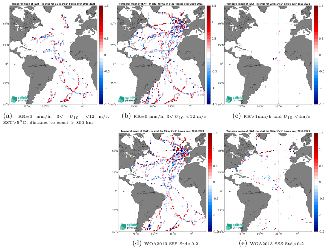
Figure 12: Temporal mean gridded over spatial boxes of size 1^\circ \times 1^\circ of \Delta\text{SSS} (SMOS SSS L2Q v331 - With FLAG (CMEMS-CATDS-CPDC) - TSG (GOSUD-Sailing-ship)) for 5 different subdatasets corresponding to:RR=0 mm/h, 3 < U_{10} < 12 m/s, SST>5°C, distance to coast > 800 km (a), RR=0 mm/h, 3 < U_{10} < 12 m/s (b), RR>1mm/h and U_{10} < 4 m/s (c), WOA2013 SSS Std<0.2 (d), WOA2013 SSS Std>0.2 (e).
