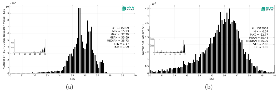
Figure 3: Histograms of SSS from TSG (GOSUD-Research-vessel) (a) and SMOS SSS L2Q v331 - With FLAG (CMEMS-CATDS-CPDC) (b) considering all match-up pairs per bins of 0.1 over the Atlantic Ocean Pi-MEP region and for the full satellite product period.
