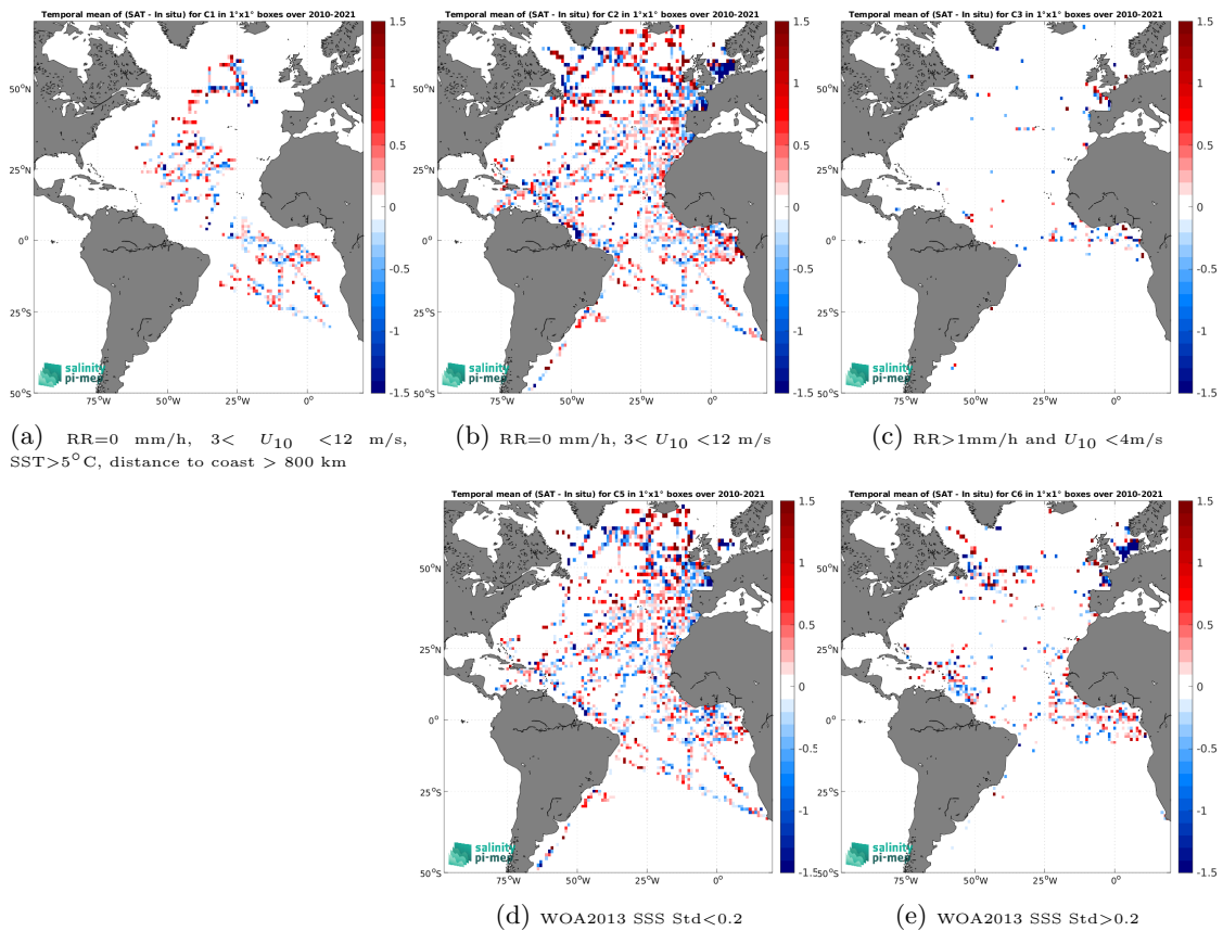
Figure 14: Temporal mean gridded over spatial boxes of size 1^\circ \times 1^\circ of \Delta\text{SSS} (SMOS SSS L2Q v331 - With FLAG (CMEMS-CATDS-CPDC) - TSG (GOSUD-Research-vessel)) for 5 different subdatasets corresponding to:RR=0 mm/h, 3 < U_{10} < 12 m/s, SST>5°C, distance to coast > 800 km (a), RR=0 mm/h, 3 < U_{10} < 12 m/s (b), RR>1mm/h and U_{10} < 4 m/s (c), WOA2013 SSS Std<0.2 (d), WOA2013 SSS Std>0.2 (e).
