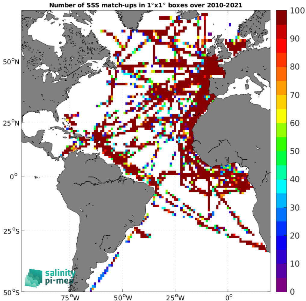
Figure 5: Number of SSS match-ups between TSG (GOSUD-Research-vessel) SSS and the SMOS SSS L2Q v331 - With FLAG (CMEMS-CATDS-CPDC) SSS product for the Atlantic Ocean Pi-MEP region over 1^\circ \times 1^\circ boxes and for the full satellite product period.
