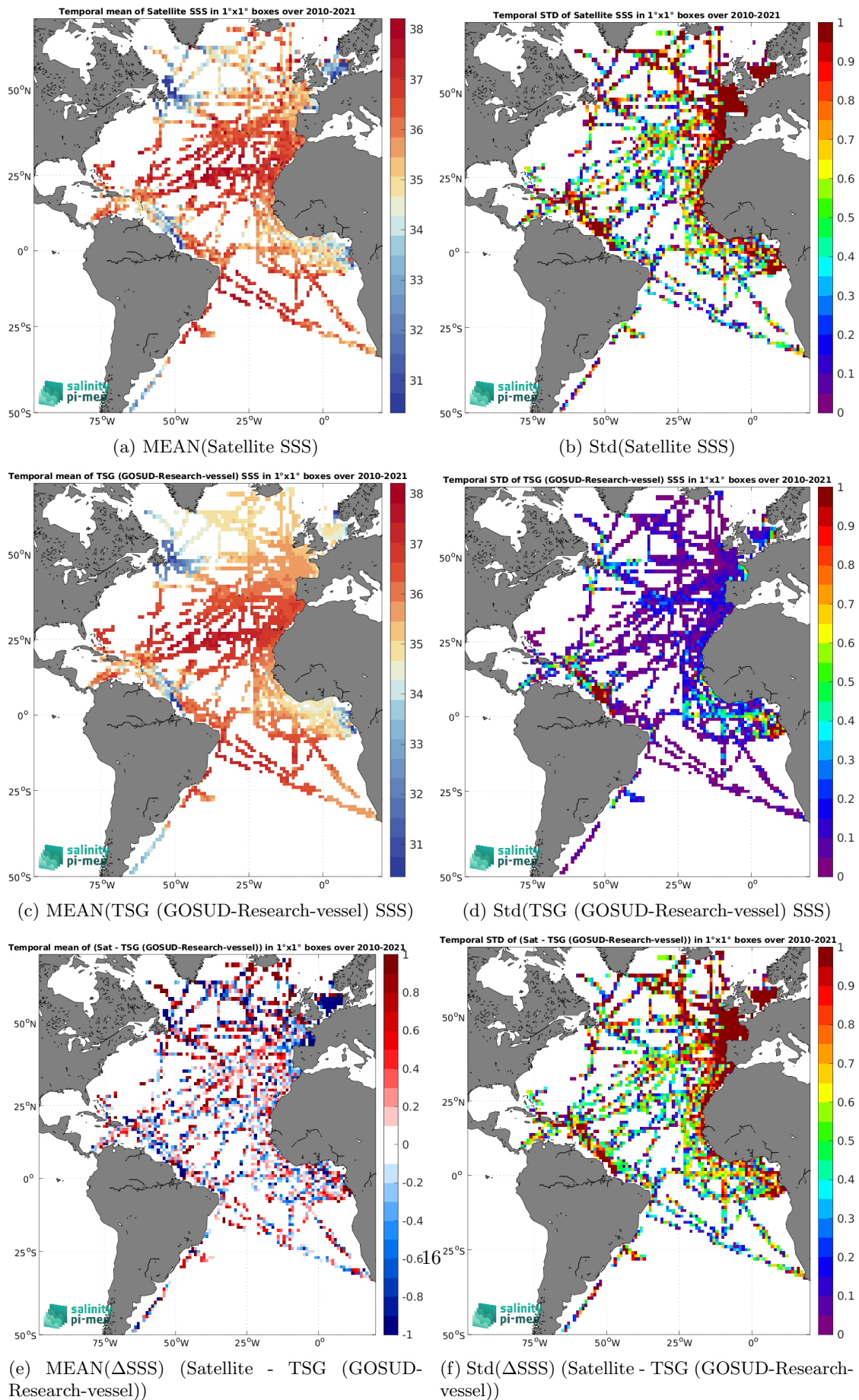
Figure 7: Temporal mean (left) and Std (right) of SSS from SMOS SSS L2Q v331 - With FLAG (CMEMS-CATDS-CPDC) (top), TSG (GOSUD-Research-vessel) (middle), and of \Delta SSS (Satellite - TSG (GOSUD-Research-vessel)). Only match-up pairs are used to generate these maps.
