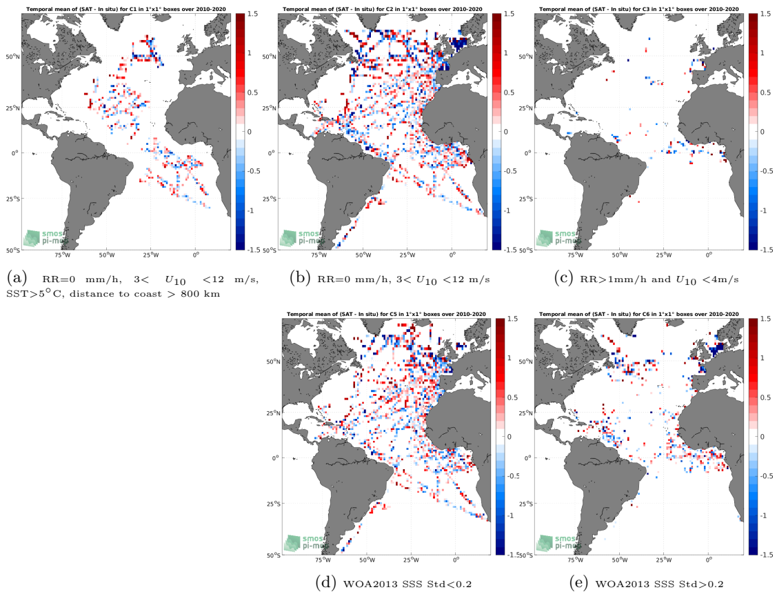
Figure 12: Temporal mean gridded over spatial boxes of size 1^\circ \times 1^\circ of \Delta SSS (SMOS SSS L2Q v331 - With FLAG (CMEMS-CATDS-CPDC) - TSG (GOSUD-Research-vessel)) for 5 different subdatasets corresponding to:RR=0 mm/h, 3 < U_{10} < 12 m/s, SST>5°C, distance to coast > 800 km (a), RR=0 mm/h, 3 < U_{10} < 12 m/s (b), RR>1mm/h and U_{10} < 4 m/s (c), WOA2013 SSS Std<0.2 (d), WOA2013 SSS Std>0.2 (e).
