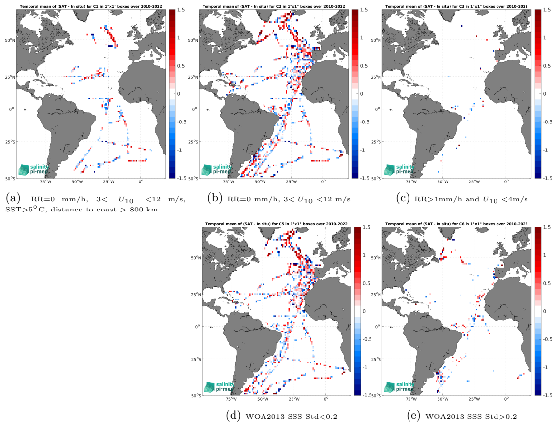
Figure 14: Temporal mean gridded over spatial boxes of size 1^\circ \times 1^\circ of \Delta SSS (SMOS SSS L2Q v331 - With FLAG (CMEMS-CATDS-CPDC) - TSG (CSIC-UTM)) for 5 different subdatasets corresponding to:RR=0 mm/h, 3 < U_{10} < 12 m/s, SST >5^\circ\text{C} , distance to coast > 800 km (a), RR=0 mm/h, 3 < U_{10} < 12 m/s (b), RR >1 mm/h and U_{10} < 4 m/s (c), WOA2013 SSS Std <0.2 (d), WOA2013 SSS Std >0.2 (e).
