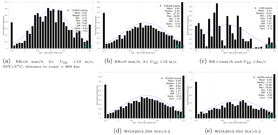
Figure 15: Normalized histogram of \Delta SSS (SMOS SSS L2Q v331 - With FLAG (CMEMS-CATDS-CPDC) - TSG (CSIC-UTM)) for 5 different subdatasets corresponding to: RR=0 mm/h, 3 < U_{10} < 12 m/s, SST>5°C, distance to coast > 800 km (a), RR=0 mm/h, 3 < U_{10} < 12 m/s (b), RR>1mm/h and U_{10} < 4 m/s (c), WOA2013 SSS Std<0.2 (d), WOA2013 SSS Std>0.2 (e).
