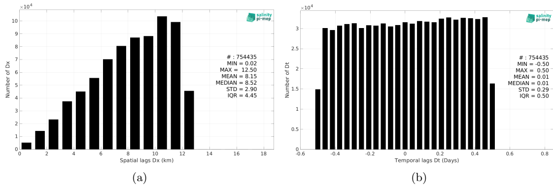
Figure 6: Histograms of the spatial (a) and temporal (b) lags between the location/time of the TSG (CSIC-UTM) measurement and the date of the corresponding SMOS SSS L2Q v331 - With FLAG (CMEMS-CATDS-CPDC) SSS pixel.
