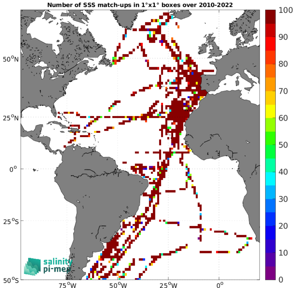
Figure 5: Number of SSS match-ups between TSG (CSIC-UTM) SSS and the SMOS SSS L2Q v331 - With FLAG (CMEMS-CATDS-CPDC) SSS product for the Atlantic Ocean Pi-MEP region over 1^\circ \times 1^\circ boxes and for the full satellite product period.
