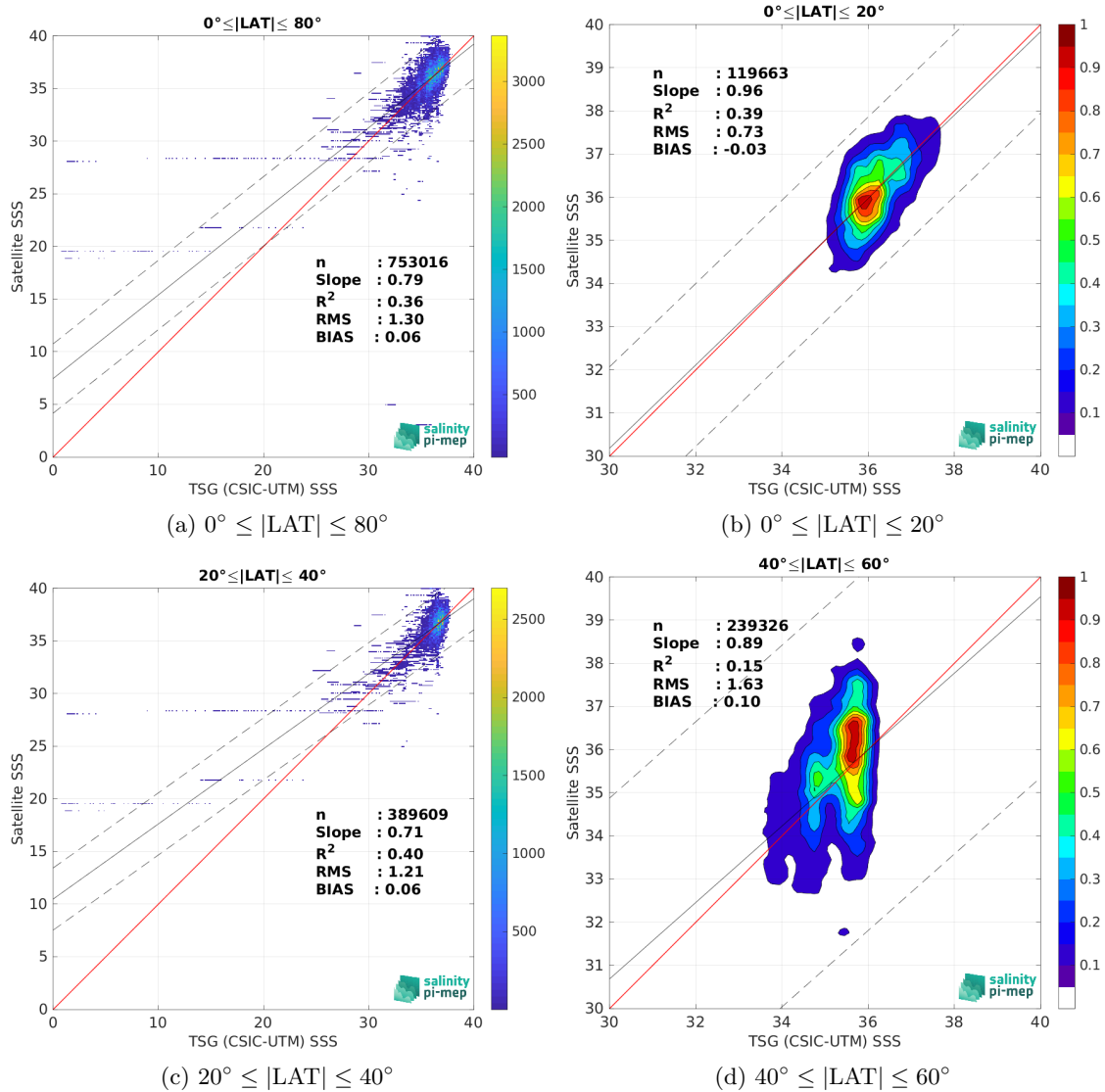
Figure 10: Contour maps of the concentration of SMOS SSS L2Q v331 - With FLAG (CMEMS-CATDS-CPDC) SSS (y-axis) versus TSG (CSIC-UTM) SSS (x-axis) at match-up pairs for different latitude bands. For each plot, the red line shows x=y . The black thin and dashed lines indicate a linear fit through the data cloud and the \pm 95\% confidence levels, respectively. The number match-up pairs n , the slope and R^2 coefficient of the linear fit, the root mean square (RMS) and the mean bias between satellite and in situ data are indicated for each latitude band in each plots.
