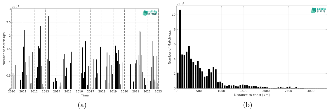
Figure 2: Number of match-ups between TSG (CSIC-UTM) and SMOS SSS L2Q v331 - With FLAG (CMEMS-CATDS-CPDC) SSS as a function of time (a) and as function of the distance to coast (b) over the Atlantic Ocean Pi-MEP region and for the full satellite product period.
