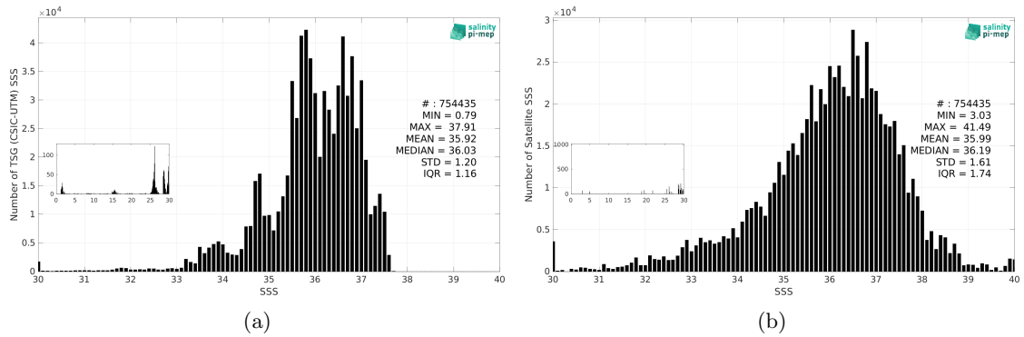
Figure 3: Histograms of SSS from TSG (CSIC-UTM) (a) and SMOS SSS L2Q v331 - With FLAG (CMEMS-CATDS-CPDC) (b) considering all match-up pairs per bins of 0.1 over the Atlantic Ocean Pi-MEP region and for the full satellite product period.
