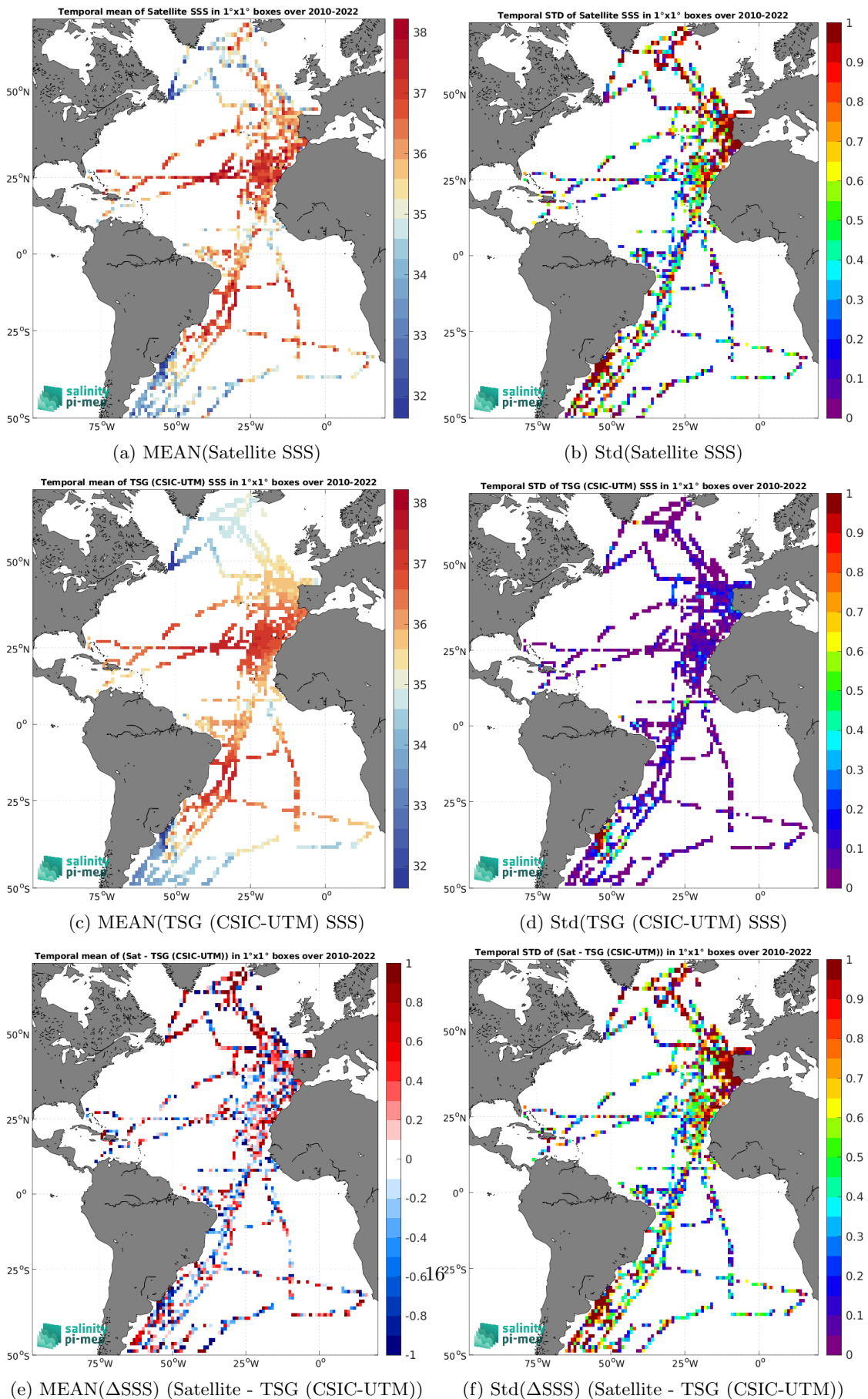
Figure 7: Temporal mean (left) and Std (right) of SSS from SMOS SSS L2Q v331 - With FLAG (CMEMS-CATDS-CPDC) (top), TSG (CSIC-UTM) (middle), and of \Delta SSS (Satellite - TSG (CSIC-UTM)). Only match-up pairs are used to generate these maps.
