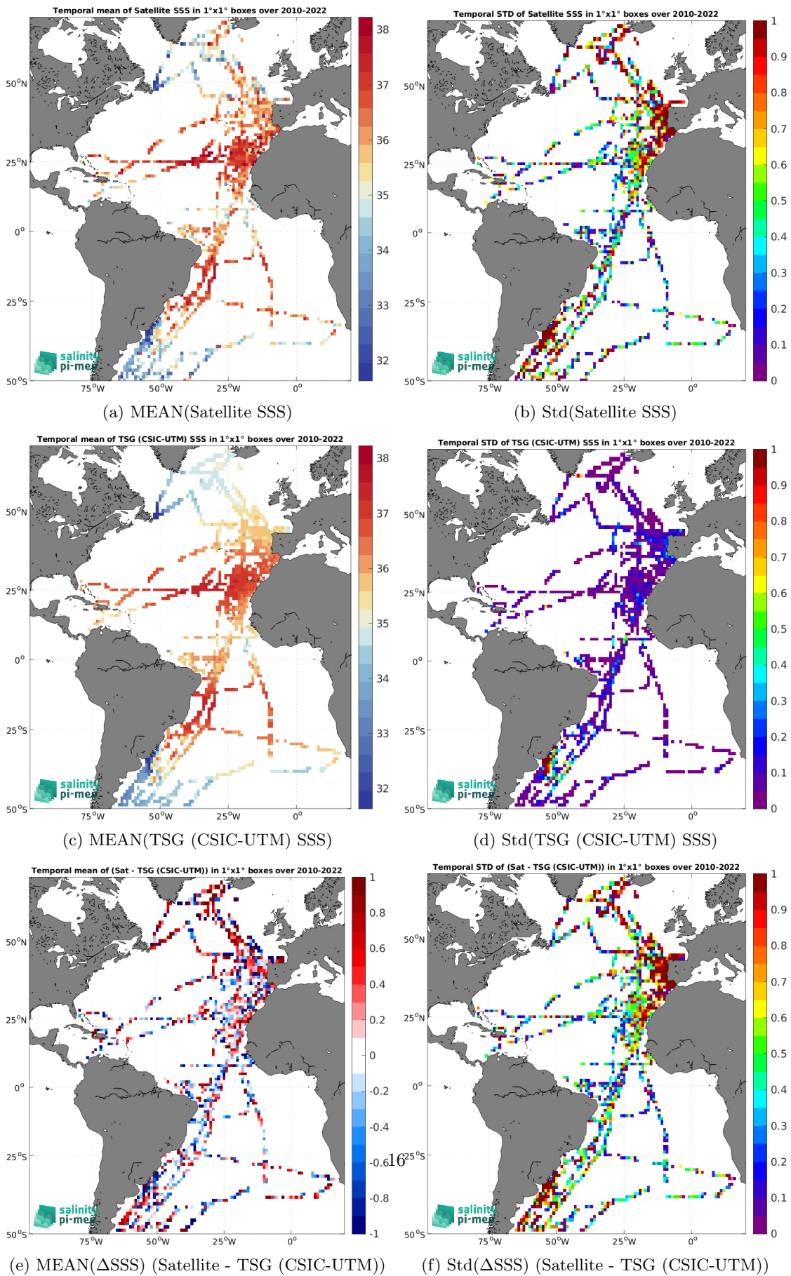
Figure 6: Temporal mean (left) and Std (right) of SSS from SMOS SSS L2Q v331 - With FLAG (CMEMS-CATDS-CPDC) (top), TSG (CSIC-UTM) (middle), and of \Delta SSS (Satellite - TSG (CSIC-UTM)). Only match-up pairs are used to generate these maps.
