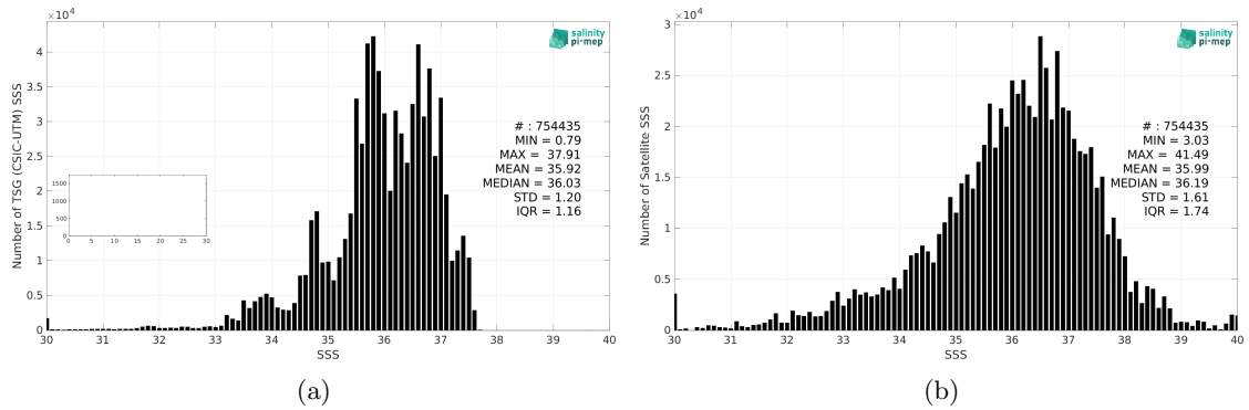
Figure 2: Histograms of SSS from TSG (CSIC-UTM) (a) and SMOS SSS L2Q v331 - With FLAG (CMEMS-CATDS-CPDC) (b) considering all match-up pairs per bins of 0.1 over the Atlantic Ocean Pi-MEP region and for the full satellite product period.
