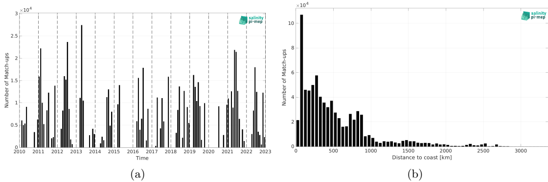
Figure 1: Number of match-ups between TSG (CSIC-UTM) and SMOS SSS L2Q v331 - With FLAG (CMEMS-CATDS-CPDC) SSS as a function of time (a) and as function of the distance to coast (b) over the Atlantic Ocean Pi-MEP region and for the full satellite product period.
