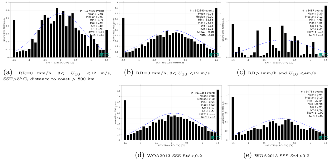
Figure 13: Normalized histogram of \Delta\text{SSS} (SMOS SSS L2Q v331 - With FLAG (CMEMS-CATDS-CPDC) - TSG (CSIC-UTM)) for 5 different subdatasets corresponding to: RR=0 mm/h, 3 < U_{10} < 12 m/s, SST > 5^\circ\text{C} , distance to coast > 800 km (a), RR=0 mm/h, 3 < U_{10} < 12 m/s (b), RR > 1 mm/h and U_{10} < 4 m/s (c), WOA2013 SSS Std < 0.2 (d), WOA2013 SSS Std > 0.2 (e).
