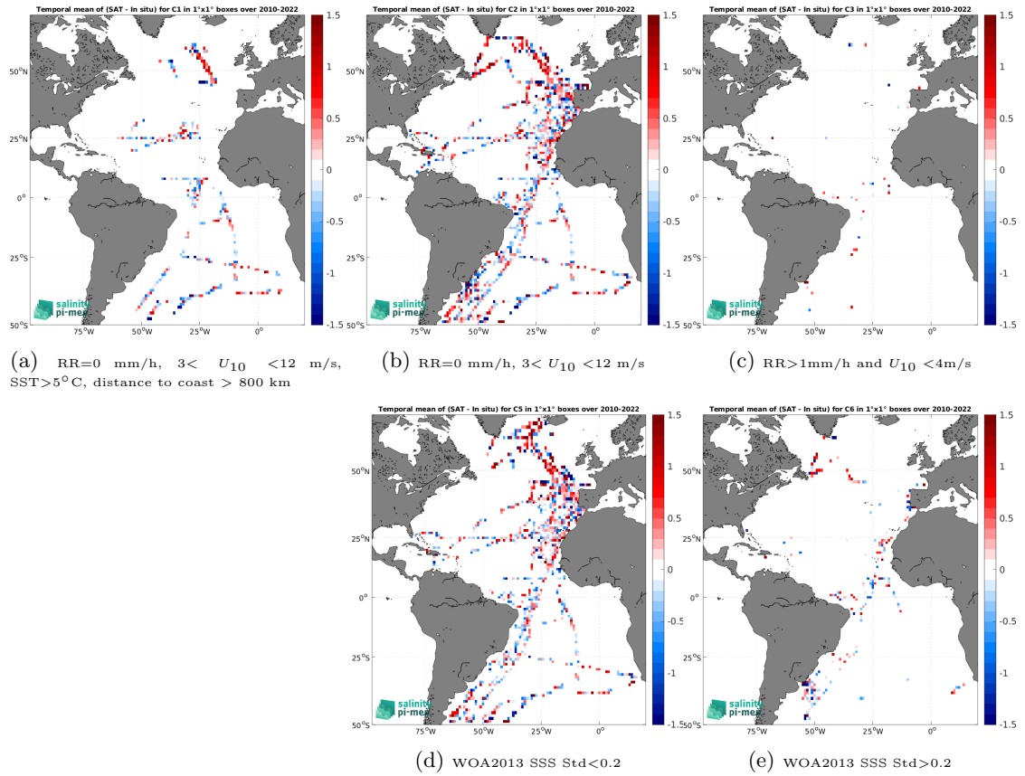
Figure 12: Temporal mean gridded over spatial boxes of size 1^\circ \times 1^\circ of \Delta SSS (SMOS SSS L2Q v331 - With FLAG (CMEMS-CATDS-CPDC) - TSG (CSIC-UTM)) for 5 different subdatasets corresponding to:RR=0 mm/h, 3 < U_{10} < 12 m/s, SST >5^\circ\text{C} , distance to coast > 800 km (a), RR=0 mm/h, 3 < U_{10} < 12 m/s (b), RR >1 mm/h and U_{10} < 4 m/s (c), WOA2013 SSS Std <0.2 (d), WOA2013 SSS Std >0.2 (e).
