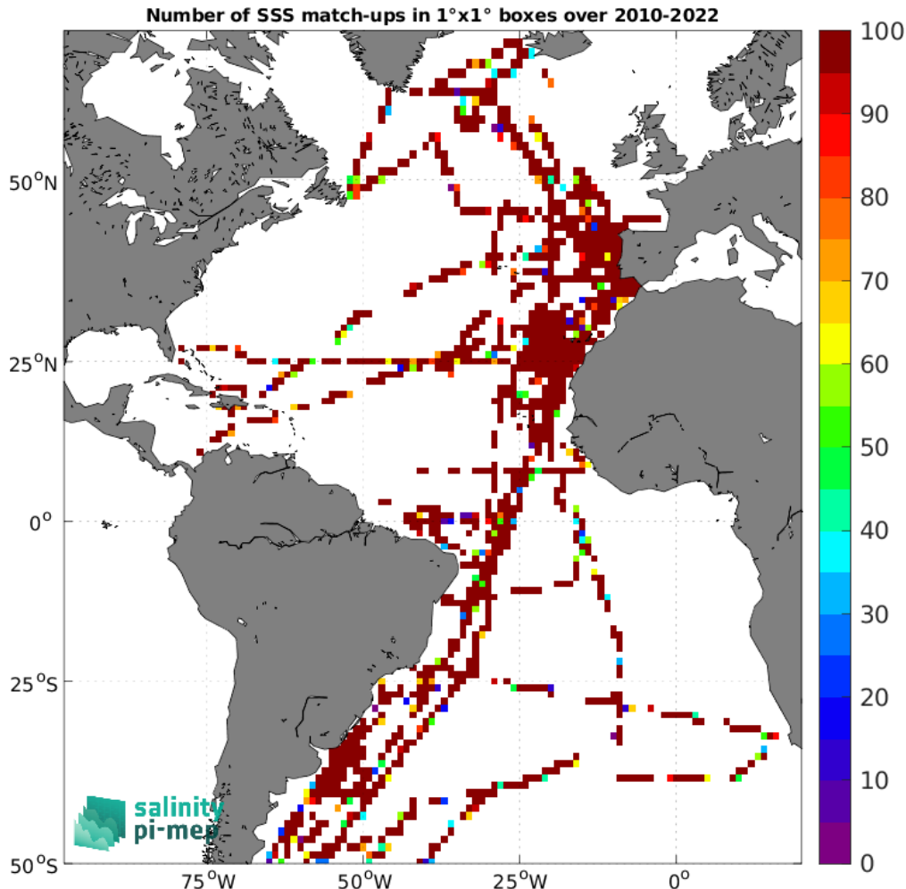
Figure 4: Number of SSS match-ups between TSG (CSIC-UTM) SSS and the SMOS SSS L2Q v331 - With FLAG (CMEMS-CATDS-CPDC) SSS product for the Atlantic Ocean Pi-MEP region over 1^\circ \times 1^\circ boxes and for the full satellite product period.
