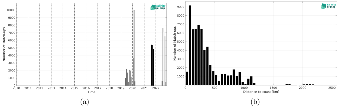
Figure 2: Number of match-ups between Saildrone and SMOS SSS L2Q v331 - With FLAG (CMEMS-CATDS-CPDC) SSS as a function of time (a) and as function of the distance to coast (b) over the Atlantic Ocean Pi-MEP region and for the full satellite product period.
