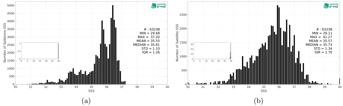
Figure 3: Histograms of SSS from Sairdrone (a) and SMOS SSS L2Q v331 - With FLAG (CMEMS-CATDS-CPDC) (b) considering all match-up pairs per bins of 0.1 over the Atlantic Ocean Pi-MEP region and for the full satellite product period.
