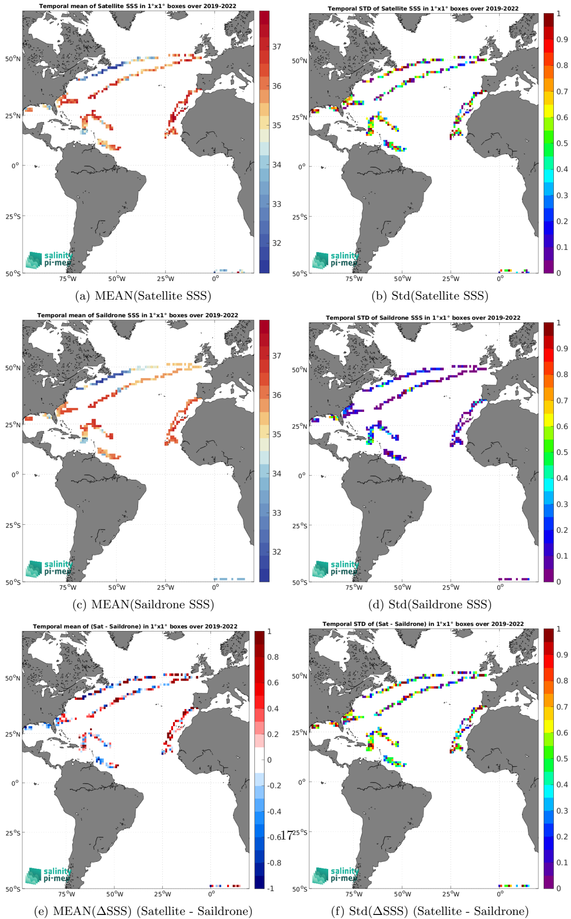
Figure 7: Temporal mean (left) and Std (right) of SSS from SMOS SSS L2Q v331 - With FLAG (CMEMS-CATDS-CPDC) (top), Saildrone (middle), and of \Delta\text{SSS} (Satellite - Saildrone). Only match-up pairs are used to generate these maps.
