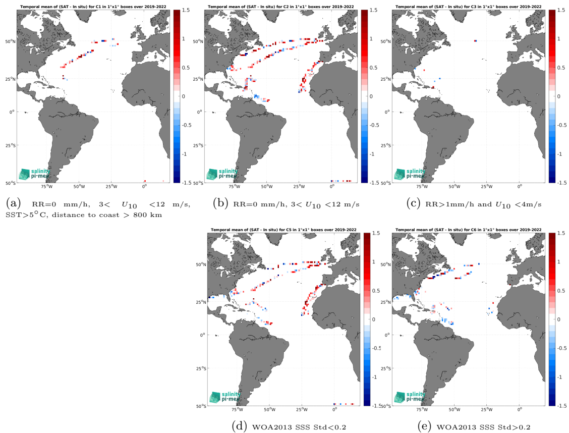
Figure 14: Temporal mean gridded over spatial boxes of size 1^\circ \times 1^\circ of \Delta SSS (SMOS SSS L2Q v331 - With FLAG (CMEMS-CATDS-CPDC) - Saildrone) for 5 different subdatasets corresponding to:RR=0 mm/h, 3 < U_{10} < 12 m/s, SST >5^\circ\text{C} , distance to coast > 800 km (a), RR=0 mm/h, 3 < U_{10} < 12 m/s (b), RR >1 mm/h and U_{10} < 4 m/s (c), WOA2013 SSS Std <0.2 (d), WOA2013 SSS Std >0.2 (e).
