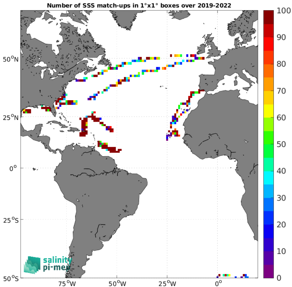
Figure 5: Number of SSS match-ups between Saildrone SSS and the SMOS SSS L2Q v331 - With FLAG (CMEMS-CATDS-CPDC) SSS product for the Atlantic Ocean Pi-MEP region over 1^\circ \times 1^\circ boxes and for the full satellite product period.
