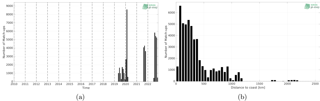
Figure 1: Number of match-ups between Sairdrone and SMOS SSS L2Q v331 - With FLAG (CMEMS-CATDS-CPDC) SSS as a function of time (a) and as function of the distance to coast (b) over the Atlantic Ocean Pi-MEP region and for the full satellite product period.
