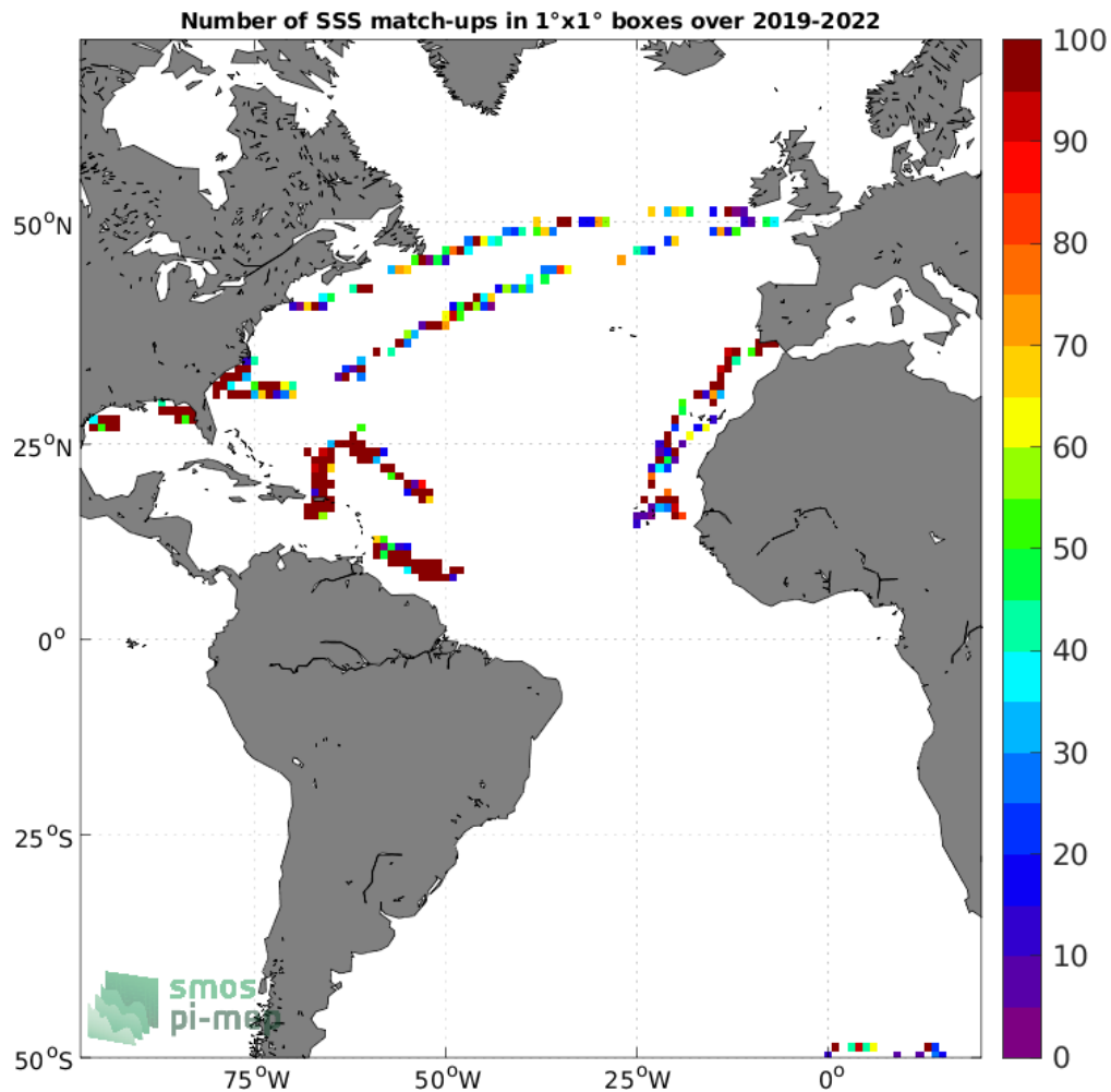
Figure 4: Number of SSS match-ups between Saildrone SSS and the SMOS SSS L2Q v331 - With FLAG (CMEMS-CATDS-CPDC) SSS product for the Atlantic Ocean Pi-MEP region over 1°x1° boxes and for the full satellite product period.
