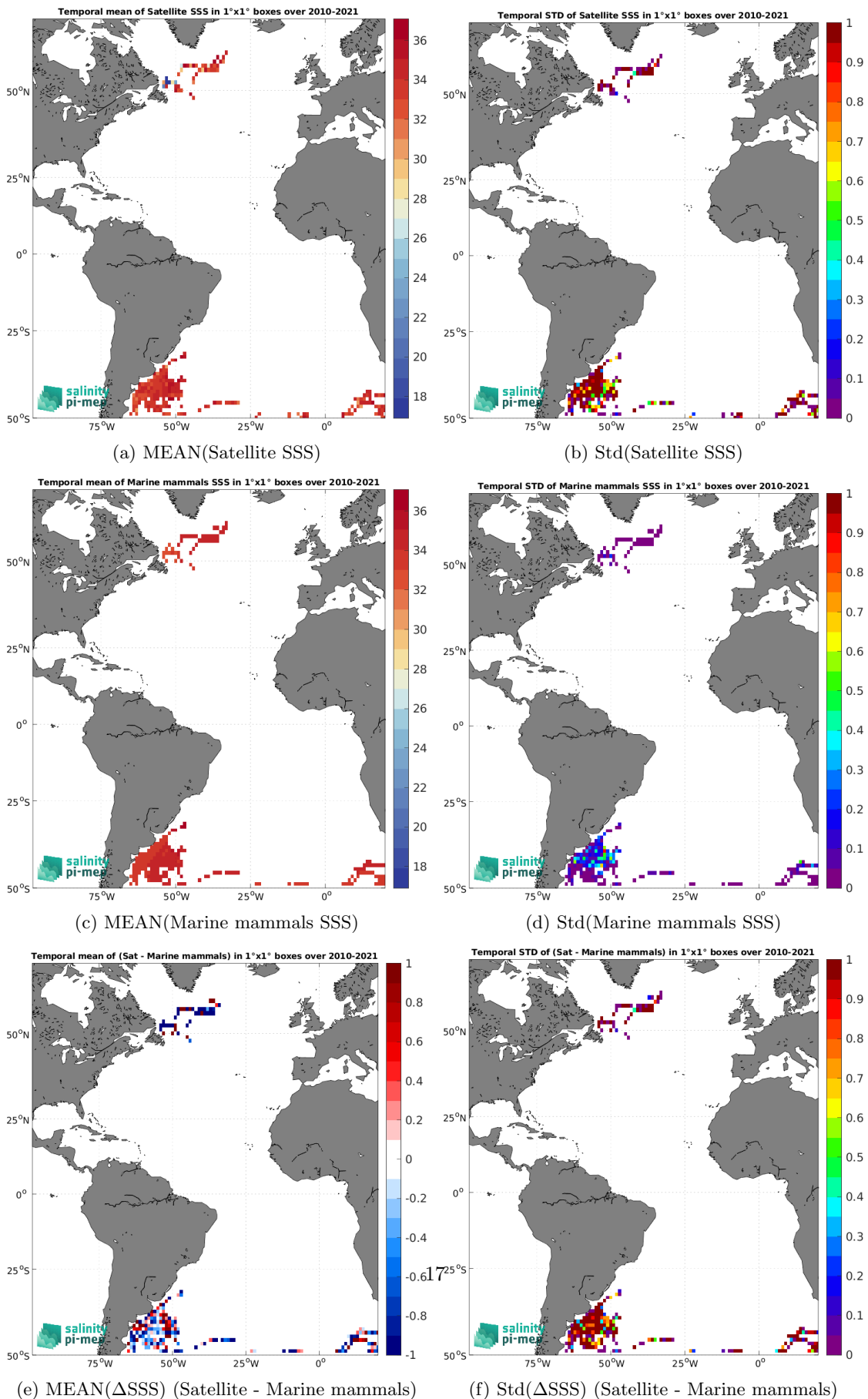
Figure 7: Temporal mean (left) and Std (right) of SSS from SMOS SSS L2Q v331 - With FLAG (CMEMS-CATDS-CPDC) (top), Marine mammals (middle), and of \Delta SSS (Satellite - Marine mammals). Only match-up pairs are used to generate these maps.
