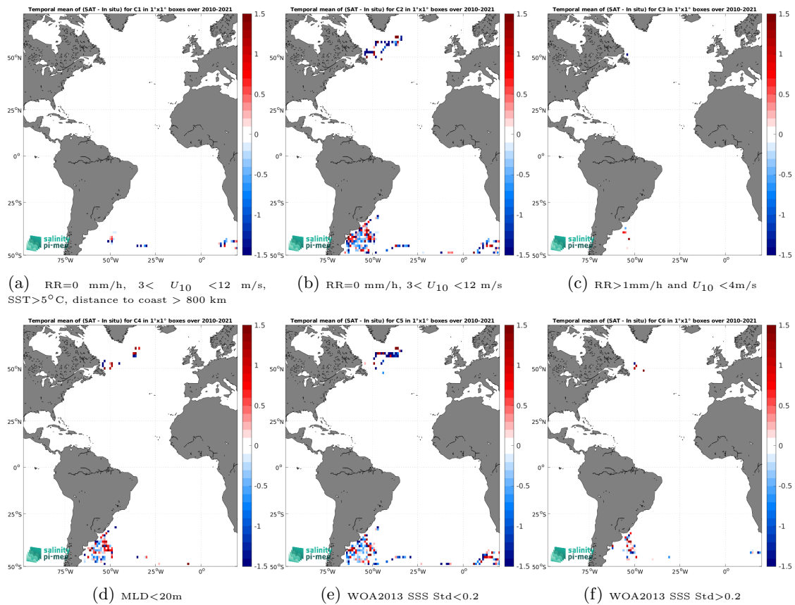
Figure 14: Temporal mean gridded over spatial boxes of size 1^\circ \times 1^\circ of \Delta SSS (SMOS SSS L2Q v331 - With FLAG (CMEMS-CATDS-CPDC) - Marine mammals) for 6 different subdatasets corresponding to:RR=0 mm/h, 3 < U_{10} < 12 m/s, SST>5°C, distance to coast > 800 km (a), RR=0 mm/h, 3 < U_{10} < 12 m/s (b), RR>1mm/h and U_{10} < 4 m/s (c),MLD<20m (d),WOA2013 SSS Std<0.2 (e),WOA2013 SSS Std>0.2 (f).
