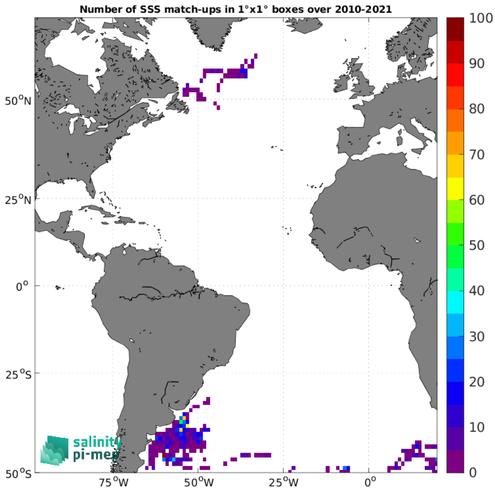
Figure 5: Number of SSS match-ups between Marine mammals SSS and the SMOS SSS L2Q v331 - With FLAG (CMEMS-CATDS-CPDC) SSS product for the Atlantic Ocean Pi-MEP region over 1° × 1° boxes and for the full satellite product period.
