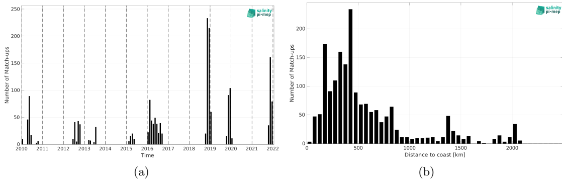
Figure 2: Number of match-ups between Marine mammals and SMOS SSS L2Q v331 - With FLAG (CMEMS-CATDS-CPDC) SSS as a function of time (a) and as function of the distance to coast (b) over the Atlantic Ocean Pi-MEP region and for the full satellite product period.
