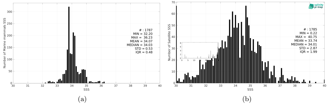
Figure 3: Histograms of SSS from Marine mammals (a) and SMOS SSS L2Q v331 - With FLAG (CMEMS-CATDS-CPDC) (b) considering all match-up pairs per bins of 0.1 over the Atlantic Ocean Pi-MEP region and for the full satellite product period.
