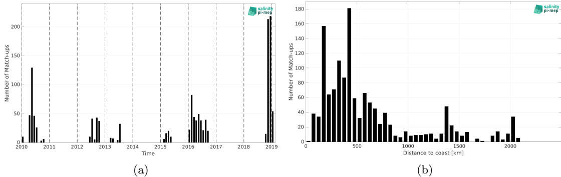
Figure 1: Number of match-ups between Marine mammals and SMOS SSS L2Q v331 - With FLAG (CMEMS-CATDS-CPDC) SSS as a function of time (a) and as function of the distance to coast (b) over the Atlantic Ocean Pi-MEP region and for the full satellite product period.
