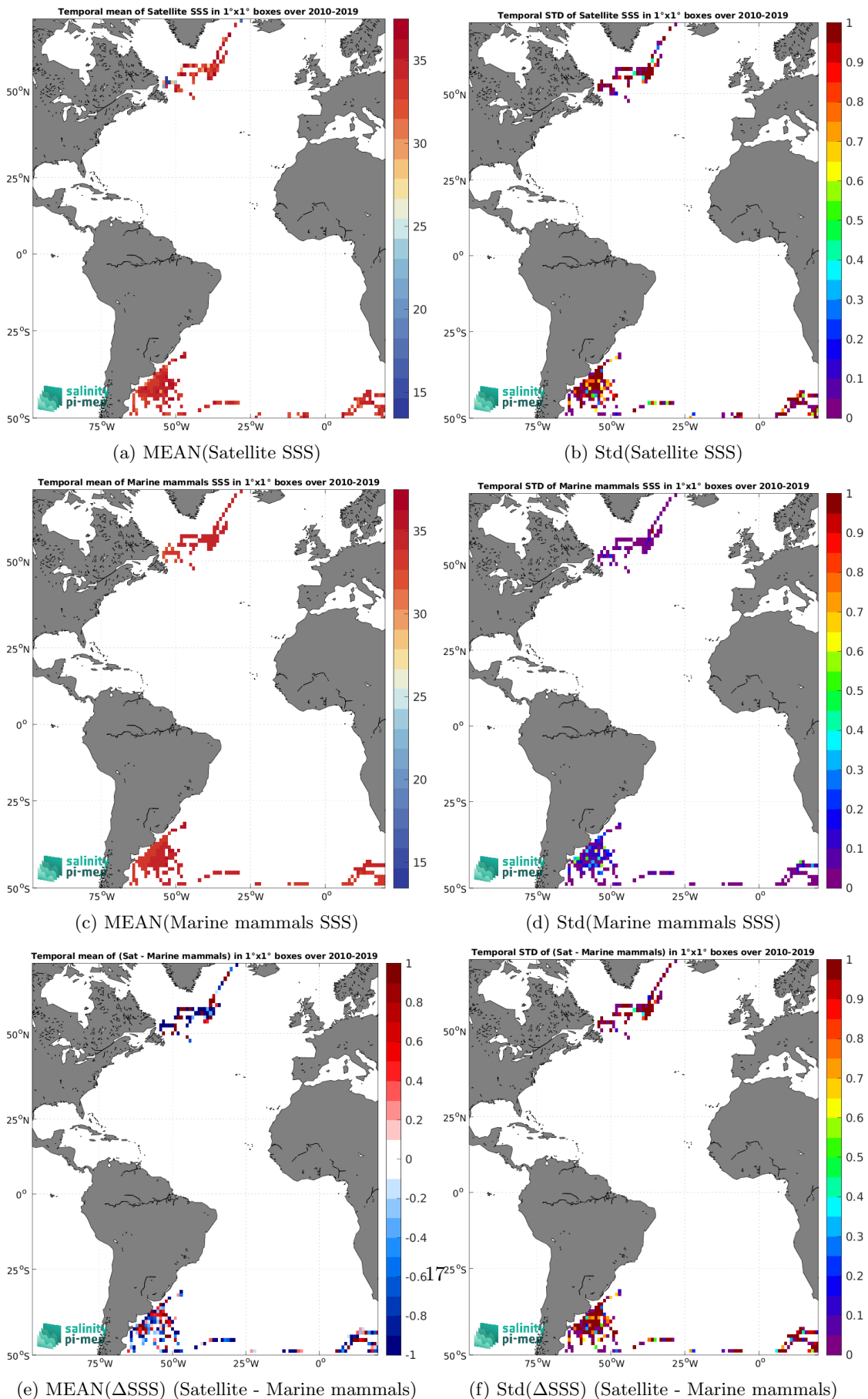
Figure 6: Temporal mean (left) and Std (right) of SSS from SMOS SSS L2Q v331 - With FLAG (CMEMS-CATDS-CPDC) (top), Marine mammals (middle), and of \Delta SSS (Satellite - Marine mammals). Only match-up pairs are used to generate these maps.
