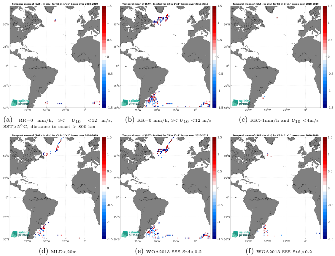
Figure 12: Temporal mean gridded over spatial boxes of size 1^{\circ} \times 1^{\circ} of \Delta SSS (SMOS SSS L2Q v331 - With FLAG (CMEMS-CATDS-CPDC) - Marine mammals) for 6 different subdatasets corresponding to: RR=0 mm/h, 3 < U_{10} < 12 m/s, SST > 5^{\circ}C , distance to coast > 800 km (a), RR=0 mm/h, 3 < U_{10} < 12 m/s (b), RR > 1 mm/h and U_{10} < 4 m/s (c), MLD < 20 m (d), WOA2013 SSS Std < 0.2 (e), WOA2013 SSS Std > 0.2 (f).
