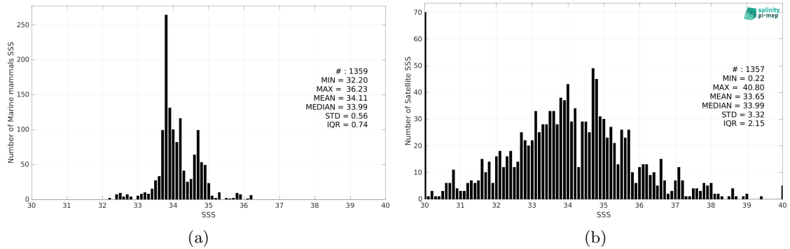
Figure 2: Histograms of SSS from Marine mammals (a) and SMOS SSS L2Q v331 - With FLAG (CMEMS-CATDS-CPDC) (b) considering all match-up pairs per bins of 0.1 over the Atlantic Ocean Pi-MEP region and for the full satellite period.
