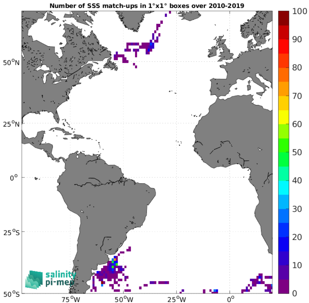
Figure 4: Number of SSS match-ups between Marine mammals SSS and the SMOS SSS L2Q v331 - With FLAG (CMEMS-CATDS-CPDC) SSS product for the Atlantic Ocean Pi-MEP region over 1^\circ \times 1^\circ boxes and for the full satellite product period.
