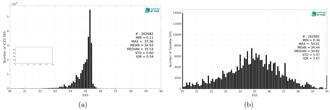
Figure 2: Histograms of SSS from ICES (a) and SMOS SSS L2Q v331 - With FLAG (CMEMS-CATDS-CPDC) (b) considering all match-up pairs per bins of 0.1 over the Atlantic Ocean Pi-MEP region and for the full satellite product period.
