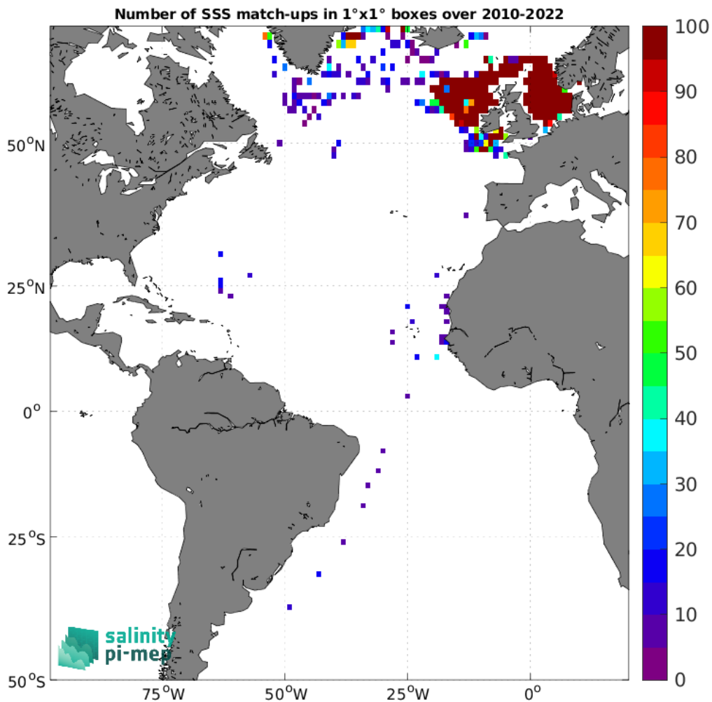
Figure 4: Number of SSS match-ups between ICES SSS and the SMOS SSS L2Q v331 - With FLAG (CMEMS-CATDS-CPDC) SSS product for the Atlantic Ocean Pi-MEP region over 1^\circ \times 1^\circ boxes and for the full satellite product period.
