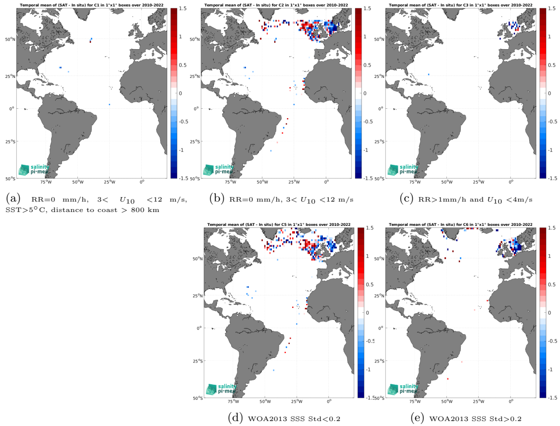
Figure 12: Temporal mean gridded over spatial boxes of size 1^\circ \times 1^\circ of \Delta SSS (SMOS SSS L2Q v331 - With FLAG (CMEMS-CATDS-CPDC) - ICES) for 5 different subdatasets corresponding to:RR=0 mm/h, 3 < U_{10} < 12 m/s, SST >5^\circ\text{C} , distance to coast > 800 km (a), RR=0 mm/h, 3 < U_{10} < 12 m/s (b), RR >1 mm/h and U_{10} < 4 m/s (c), WOA2013 SSS Std <0.2 (d), WOA2013 SSS Std >0.2 (e).
