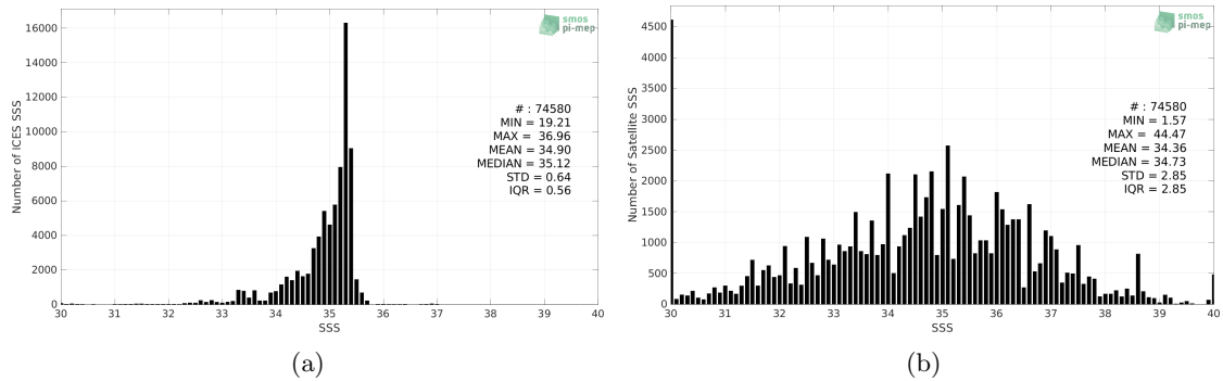
Figure 2: Histograms of SSS from ICES (a) and SMOS SSS L2Q v331 - With FLAG (CMEMS-CATDS-CPDC) (b) considering all match-up pairs per bins of 0.1 over the Atlantic Ocean Pi-MEP region and for the full satellite product period.
