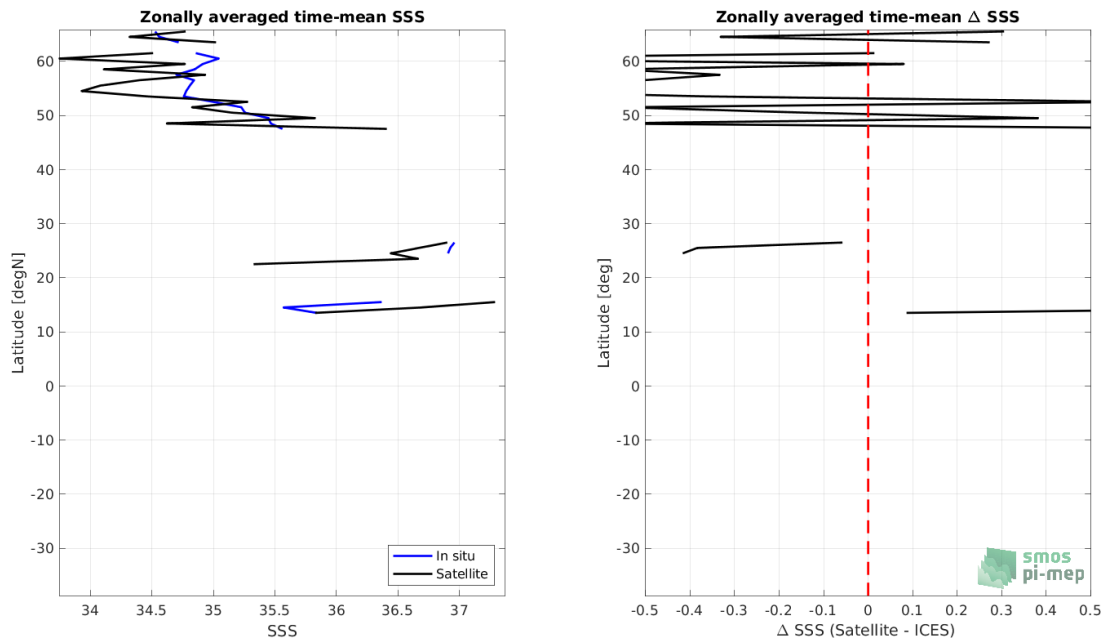
Figure 8: Left panel: Zonal mean SSS from SMOS SSS L2Q v331 - With FLAG (CMEMS-CATDS-CPDC) satellite product (black) and from ICES (blue). Right panel: Zonal mean of \Delta SSS (Satellite - ICES) for all the collected Pi-MEP match-up pairs estimated over the full satellite product period.
