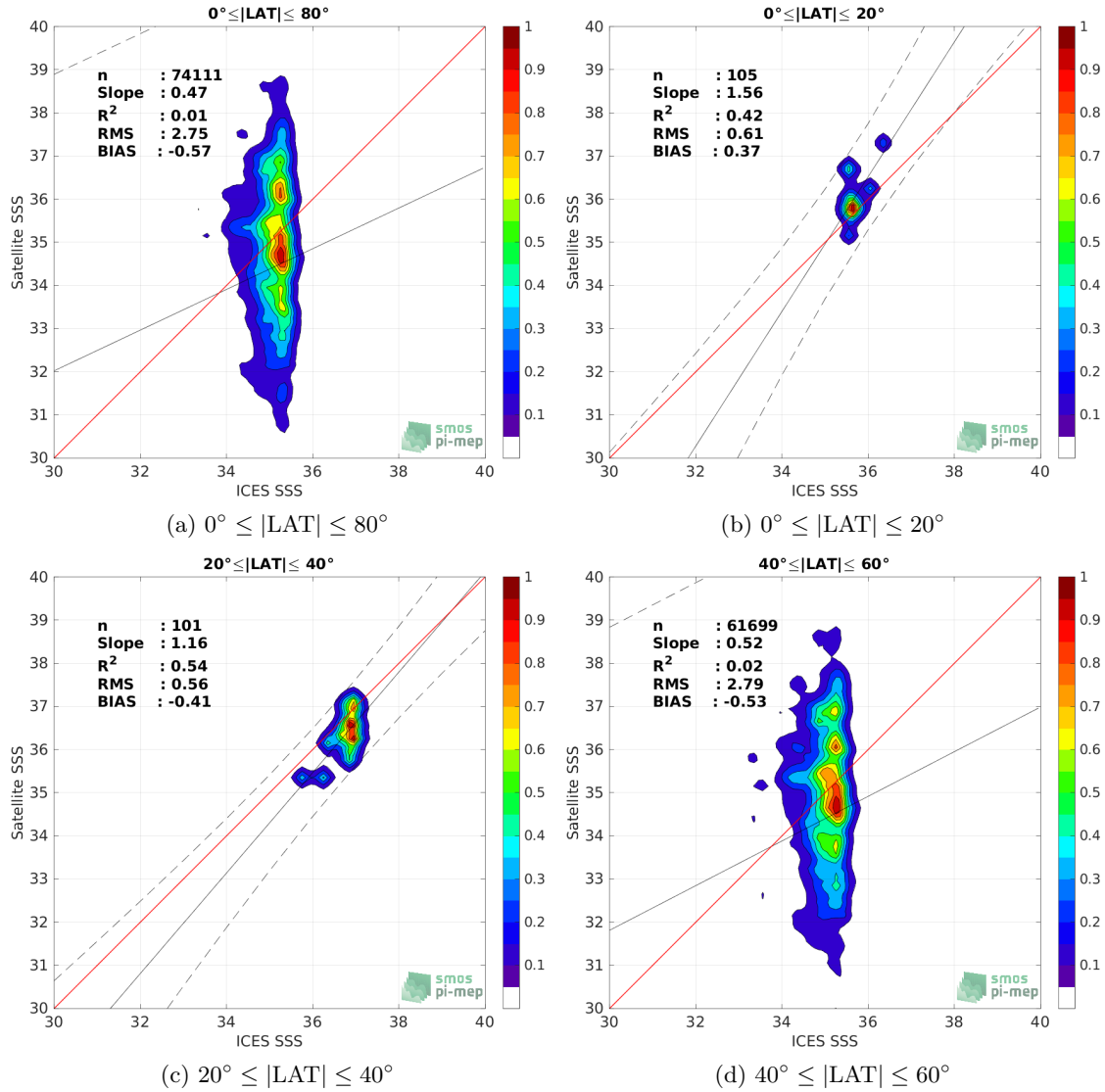
Figure 9: Contour maps of the concentration of SMOS SSS L2Q v331 - With FLAG (CMEMS-CATDS-CPDC) SSS (y-axis) versus ICES SSS (x-axis) at match-up pairs for different latitude bands. For each plot, the red line shows x=y . The black thin and dashed lines indicate a linear fit through the data cloud and the \pm 95\% confidence levels, respectively. The number match-up pairs n , the slope and R^2 coefficient of the linear fit, the root mean square (RMS) and the mean bias between satellite and in situ data are indicated for each latitude band in each plots.
