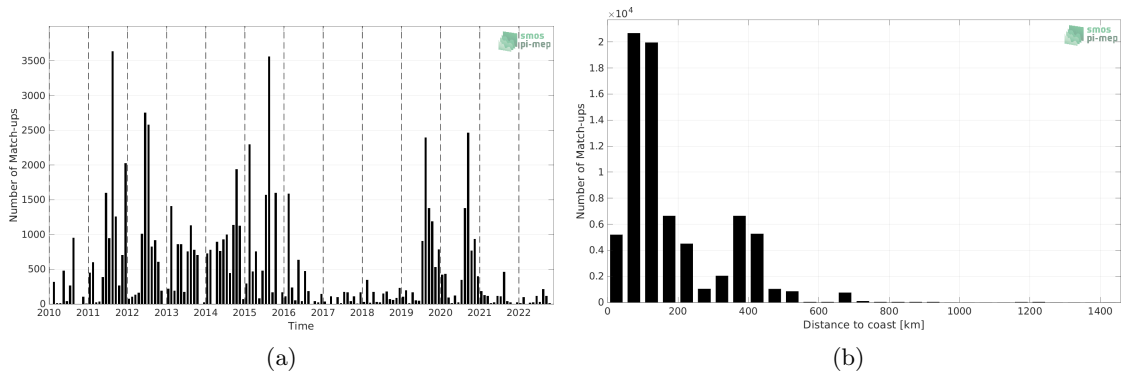
Figure 1: Number of match-ups between ICES and SMOS SSS L2Q v331 - With FLAG (CMEMS-CATDS-CPDC) SSS as a function of time (a) and as function of the distance to coast (b) over the Atlantic Ocean Pi-MEP region and for the full satellite product period.
