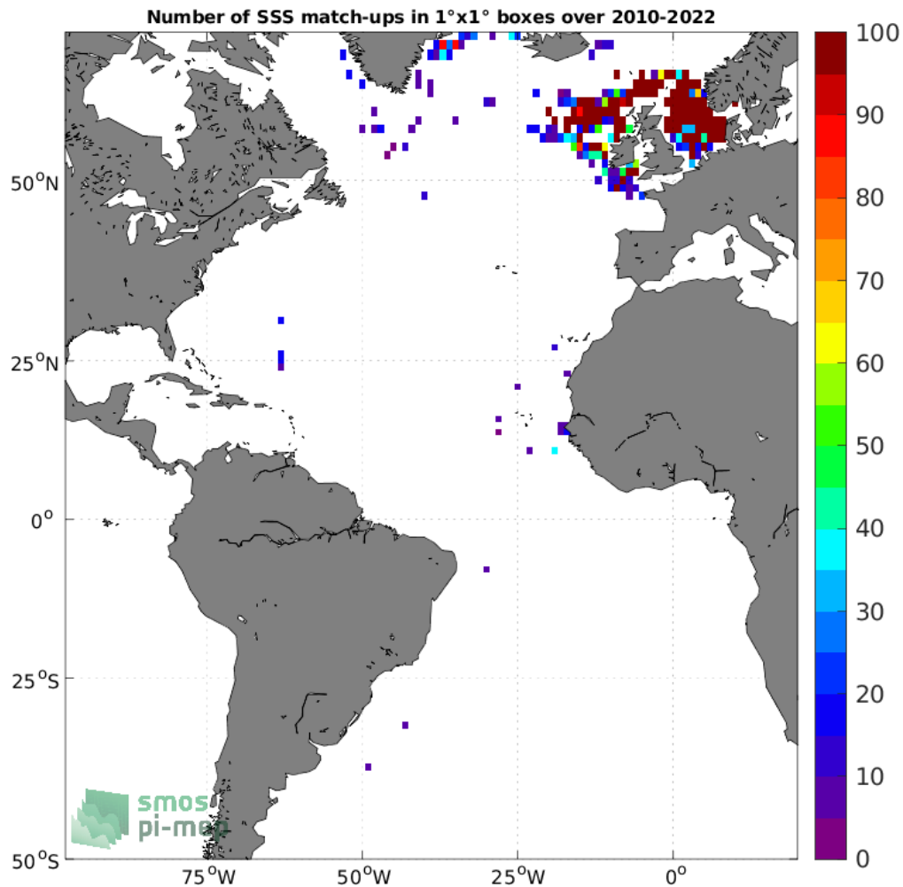
Figure 4: Number of SSS match-ups between ICES SSS and the SMOS SSS L2Q v331 - With FLAG (CMEMS-CATDS-CPDC) SSS product for the Atlantic Ocean Pi-MEP region over 1°x1° boxes and for the full satellite product period.
