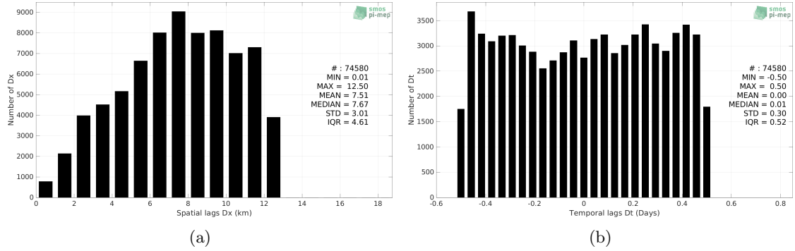
Figure 5: Histograms of the spatial (a) and temporal (b) lags between the location/time of the ICES measurement and the date of the corresponding SMOS SSS L2Q v331 - With FLAG (CMEMS-CATDS-CPDC) SSS pixel.
