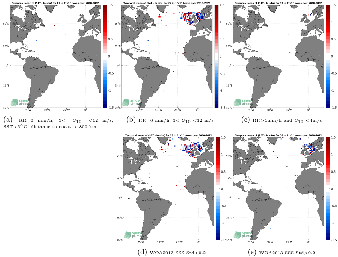
Figure 12: Temporal mean gridded over spatial boxes of size 1^\circ \times 1^\circ of \Delta\text{SSS} (SMOS SSS L2Q v331 - With FLAG (CMEMS-CATDS-CPDC) - ICES) for 5 different subdatasets corresponding to:RR=0 mm/h, 3 < U_{10} < 12 m/s, SST >5^\circ\text{C} , distance to coast > 800 km (a), RR=0 mm/h, 3 < U_{10} < 12 m/s (b), RR >1 mm/h and U_{10} < 4 m/s (c), WOA2013 SSS Std <0.2 (d), WOA2013 SSS Std >0.2 (e).
