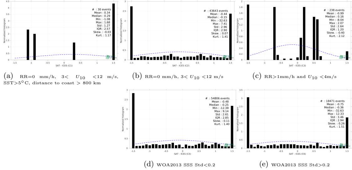
Figure 13: Normalized histogram of \Delta SSS (SMOS SSS L2Q v331 - With FLAG (CMEMS-CATDS-CPDC) - ICES) for 5 different subdatasets corresponding to: RR=0 mm/h, 3 < U_{10} < 12 m/s, SST > 5°C, distance to coast > 800 km (a), RR=0 mm/h, 3 < U_{10} < 12 m/s (b), RR > 1mm/h and U_{10} < 4 m/s (c), WOA2013 SSS Std < 0.2 (d), WOA2013 SSS Std > 0.2 (e).
