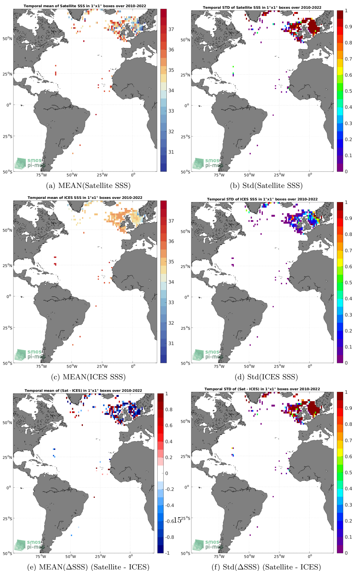
Figure 6: Temporal mean (left) and Std (right) of SSS from SMOS SSS L2Q v331 - With FLAG (CMEMS-CATDS-CPDC) (top), ICES (middle), and of \Delta SSS (Satellite - ICES). Only match-up pairs are used to generate these maps.
