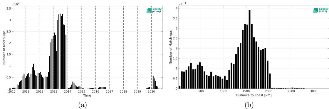
Figure 2: Number of match-ups between Surface drifters and SMOS SSS L2Q v331 - With FLAG (CMEMS-CATDS-CPDC) SSS as a function of time (a) and as function of the distance to coast (b) over the Atlantic Ocean Pi-MEP region and for the full satellite product period.
