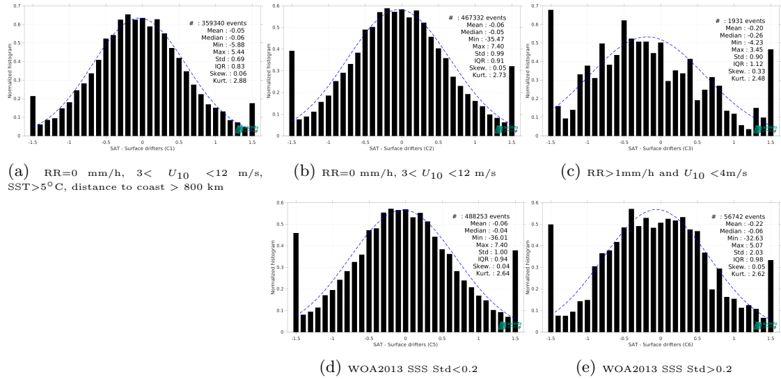
Figure 14: Normalized histogram of \Delta\text{SSS} (SMOS SSS L2Q v331 - With FLAG (CMEMS-CATDS-CPDC) - Surface drifters) for 5 different subdatasets corresponding to: RR=0 mm/h, 3 < U_{10} < 12 m/s, SST > 5^\circ\text{C} , distance to coast > 800 km (a), RR=0 mm/h, 3 < U_{10} < 12 m/s (b), RR > 1 mm/h and U_{10} < 4 m/s (c), WOA2013 SSS Std < 0.2 (d), WOA2013 SSS Std > 0.2 (e).
