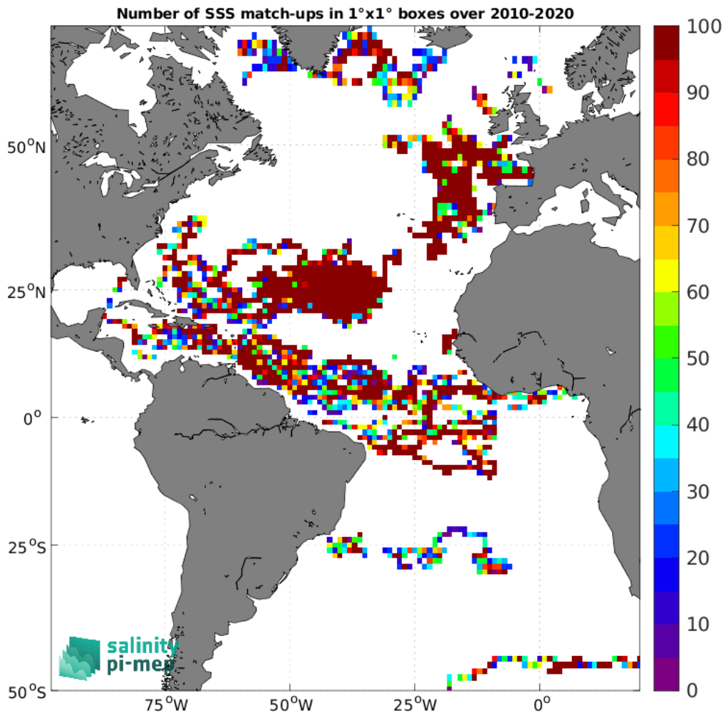
Figure 4: Number of SSS match-ups between Surface drifters SSS and the SMOS SSS L2Q v331 - With FLAG (CMEMS-CATDS-CPDC) SSS product for the Atlantic Ocean Pi-MEP region over 1°x1° boxes and for the full satellite product period.
