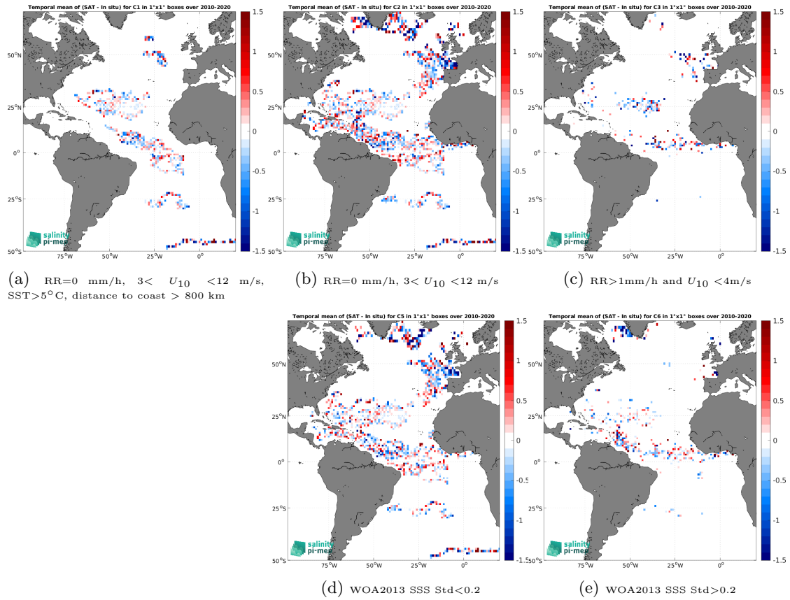
Figure 13: Temporal mean gridded over spatial boxes of size 1^\circ \times 1^\circ of \Delta SSS (SMOS SSS L2Q v331 - With FLAG (CMEMS-CATDS-CPDC) - Surface drifters) for 5 different subdatasets corresponding to:RR=0 mm/h, 3 < U_{10} < 12 m/s, SST >5^\circ\text{C} , distance to coast > 800 km (a), RR=0 mm/h, 3 < U_{10} < 12 m/s (b), RR >1 mm/h and U_{10} < 4 m/s (c), WOA2013 SSS Std <0.2 (d), WOA2013 SSS Std >0.2 (e).
