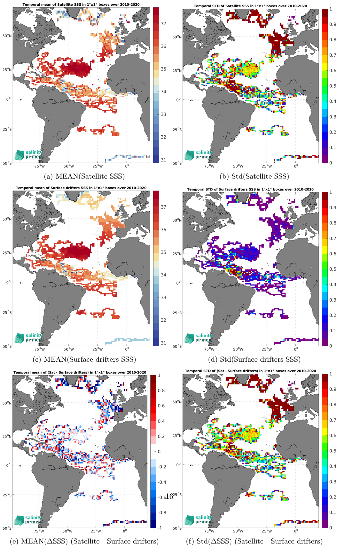
Figure 6: Temporal mean (left) and Std (right) of SSS from SMOS SSS L2Q v331 - With FLAG (CMEMS-CATDS-CPDC) (top), Surface drifters (middle), and of \Delta SSS (Satellite - Surface drifters). Only match-up pairs are used to generate these maps.
