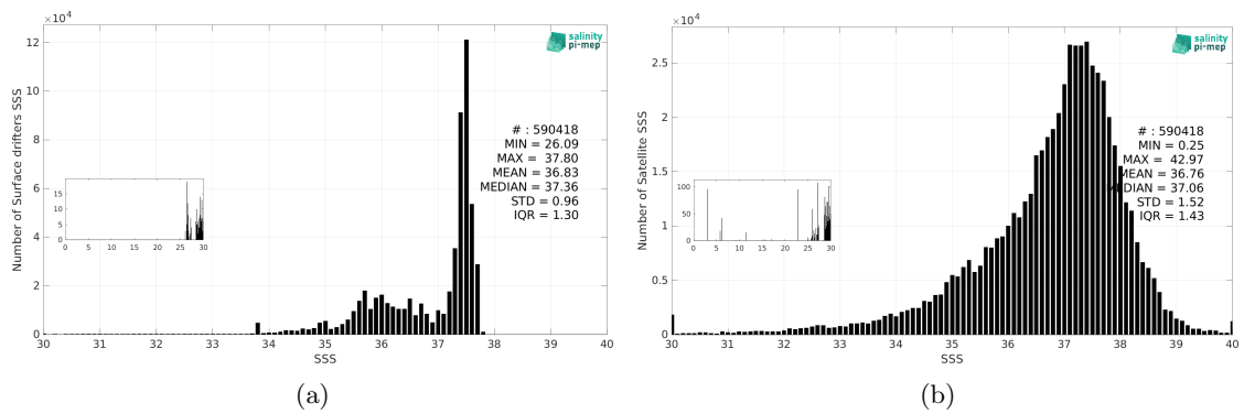
Figure 3: Histograms of SSS from Surface drifters (a) and SMOS SSS L2Q v331 - With FLAG (CMEMS-CATDS-CPDC) (b) considering all match-up pairs per bins of 0.1 over the Atlantic Ocean Pi-MEP region and for the full satellite product period.
