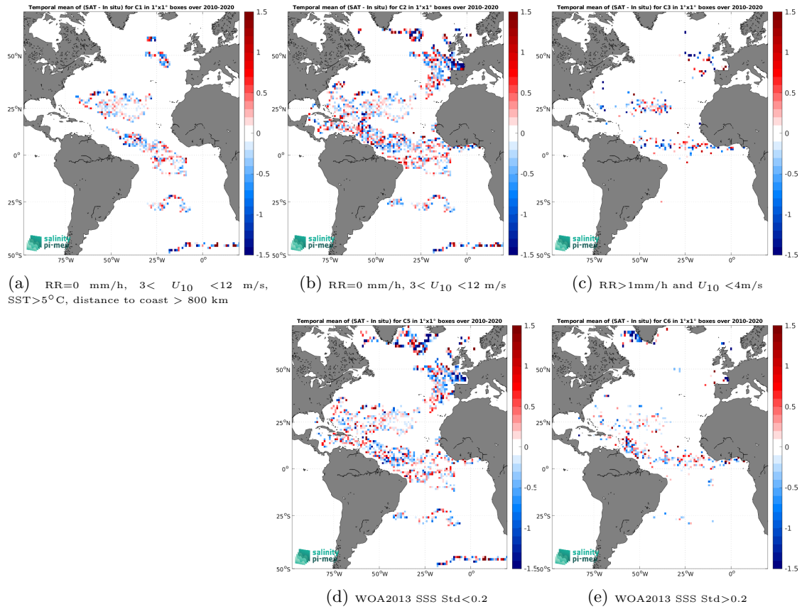
Figure 11: Temporal mean gridded over spatial boxes of size 1^\circ \times 1^\circ of \Delta SSS (SMOS SSS L2Q v331 - With FLAG (CMEMS-CATDS-CPDC) - Surface drifters) for 5 different subdatasets corresponding to:RR=0 mm/h, 3 < U_{10} < 12 m/s, SST >5^\circ\text{C} , distance to coast > 800 km (a), RR=0 mm/h, 3 < U_{10} < 12 m/s (b), RR >1 mm/h and U_{10} < 4 m/s (c), WOA2013 SSS Std <0.2 (d), WOA2013 SSS Std >0.2 (e).
