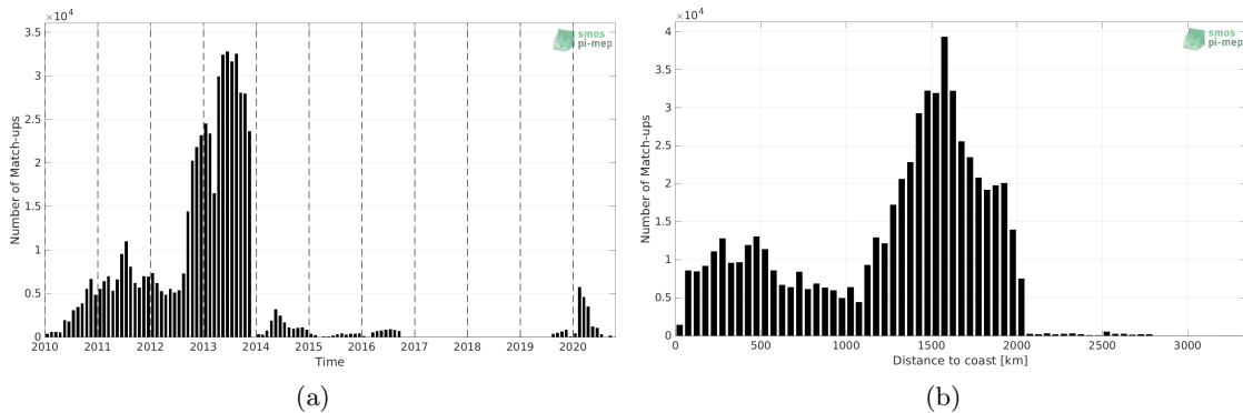
Figure 1: Number of match-ups between Surface drifters and SMOS SSS L2Q v331 - With FLAG (CMEMS-CATDS-CPDC) SSS as a function of time (a) and as function of the distance to coast (b) over the Atlantic Ocean Pi-MEP region and for the full satellite product period.
