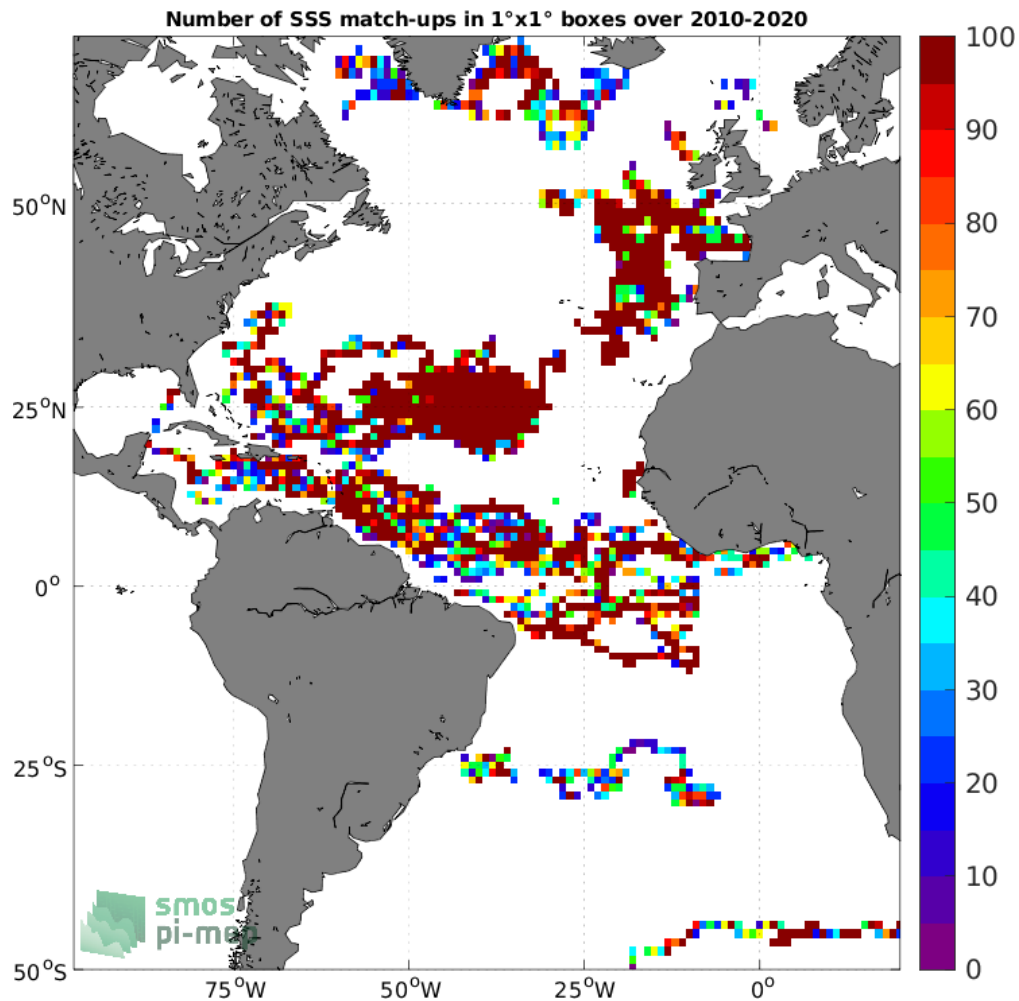
Figure 3: Number of SSS match-ups between Surface drifters SSS and the SMOS SSS L2Q v331 - With FLAG (CMEMS-CATDS-CPDC) SSS product for the Atlantic Ocean Pi-MEP region over 1°x1° boxes and for the full satellite product period.
