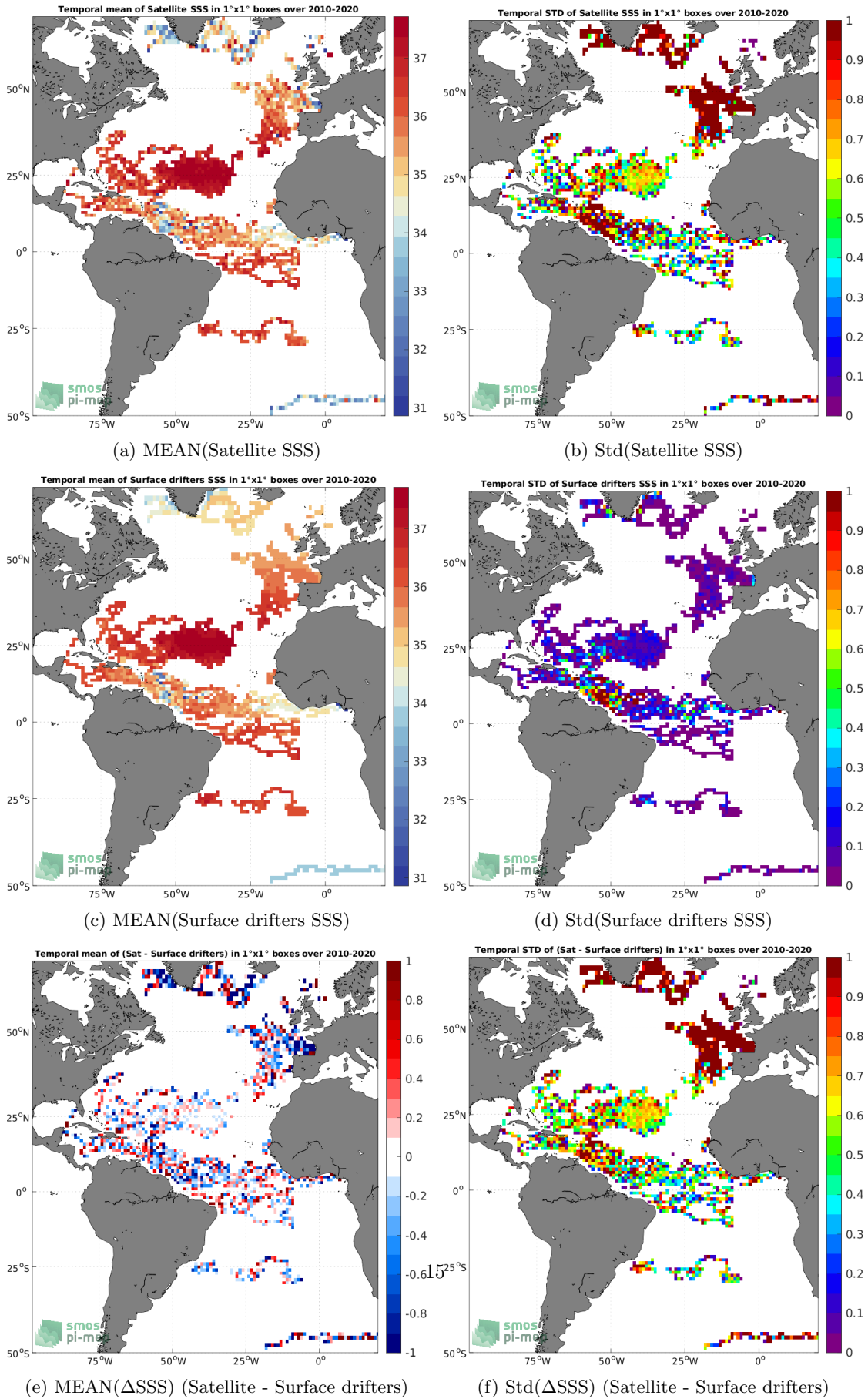
Figure 5: Temporal mean (left) and Std (right) of SSS from SMOS SSS L2Q v331 - With FLAG (CMEMS-CATDS-CPDC) (top), Surface drifters (middle), and of \Delta SSS (Satellite - Surface drifters). Only match-up pairs are used to generate these maps.
