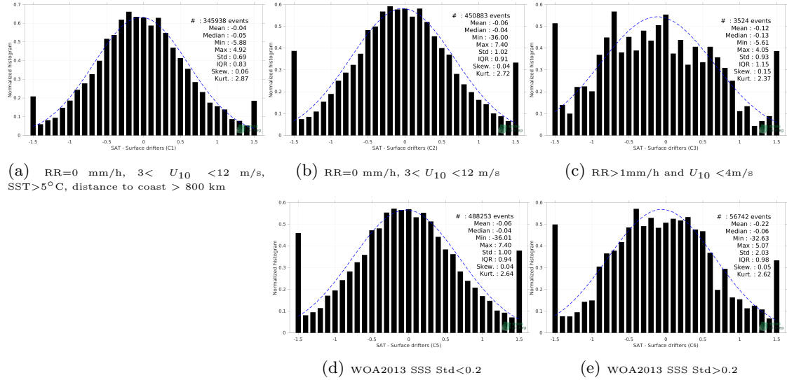
Figure 12: Normalized histogram of \Delta SSS (SMOS SSS L2Q v331 - With FLAG (CMEMS-CATDS-CPDC) - Surface drifters) for 5 different subdatasets corresponding to: RR=0 mm/h, 3 < U_{10} < 12 m/s, SST > 5°C, distance to coast > 800 km (a), RR=0 mm/h, 3 < U_{10} < 12 m/s (b), RR > 1mm/h and U_{10} < 4 m/s (c), WOA2013 SSS Std < 0.2 (d), WOA2013 SSS Std > 0.2 (e).
