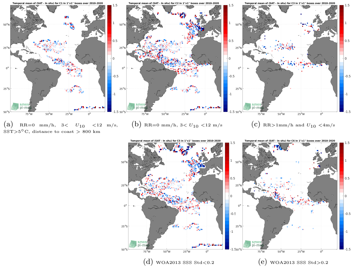
Figure 11: Temporal mean gridded over spatial boxes of size 1^\circ \times 1^\circ of \Delta\text{SSS} (SMOS SSS L2Q v331 - With FLAG (CMEMS-CATDS-CPDC) - Surface drifters) for 5 different subdatasets corresponding to:RR=0 mm/h, 3 < U_{10} < 12 m/s, SST >5^\circ\text{C} , distance to coast > 800 km (a), RR=0 mm/h, 3 < U_{10} < 12 m/s (b), RR >1 mm/h and U_{10} < 4 m/s (c), WOA2013 SSS Std <0.2 (d), WOA2013 SSS Std >0.2 (e).
