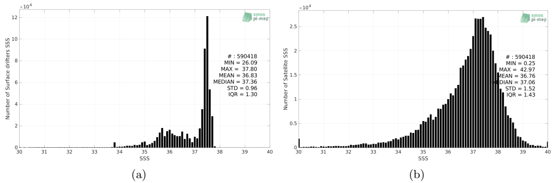
Figure 2: Histograms of SSS from Surface drifters (a) and SMOS SSS L2Q v331 - With FLAG (CMEMS-CATDS-CPDC) (b) considering all match-up pairs per bins of 0.1 over the Atlantic Ocean Pi-MEP region and for the full satellite product period.
