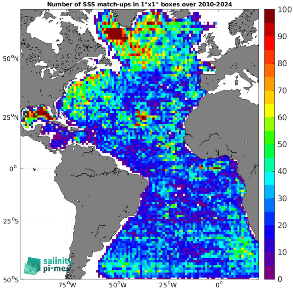
Figure 5: Number of SSS match-ups between Argo SSS and the SMOS SSS L2Q v331 - With FLAG (CMEMS-CATDS-CPDC) SSS product for the Atlantic Ocean Pi-MEP region over 1^\circ \times 1^\circ boxes and for the full satellite product period.
