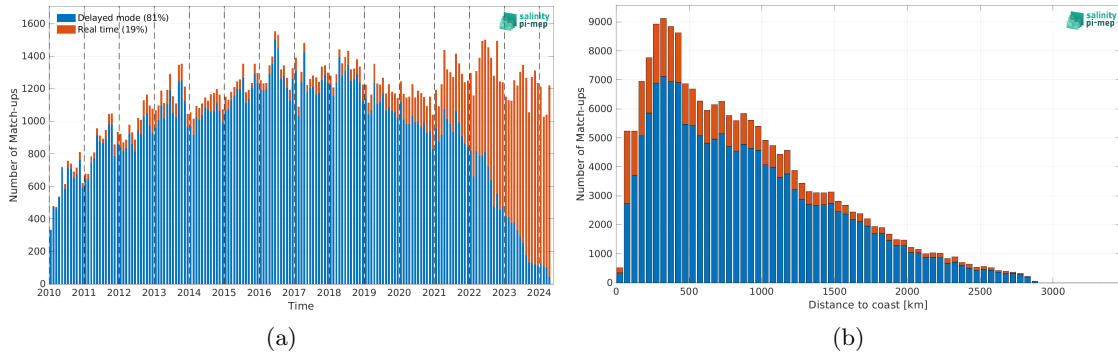
Figure 2: Number of match-ups between Argo and SMOS SSS L2Q v331 - With FLAG (CMEMS-CATDS-CPDC) SSS as a function of time (a) and as function of the distance to coast (b) over the Atlantic Ocean Pi-MEP region and for the full satellite product period.
