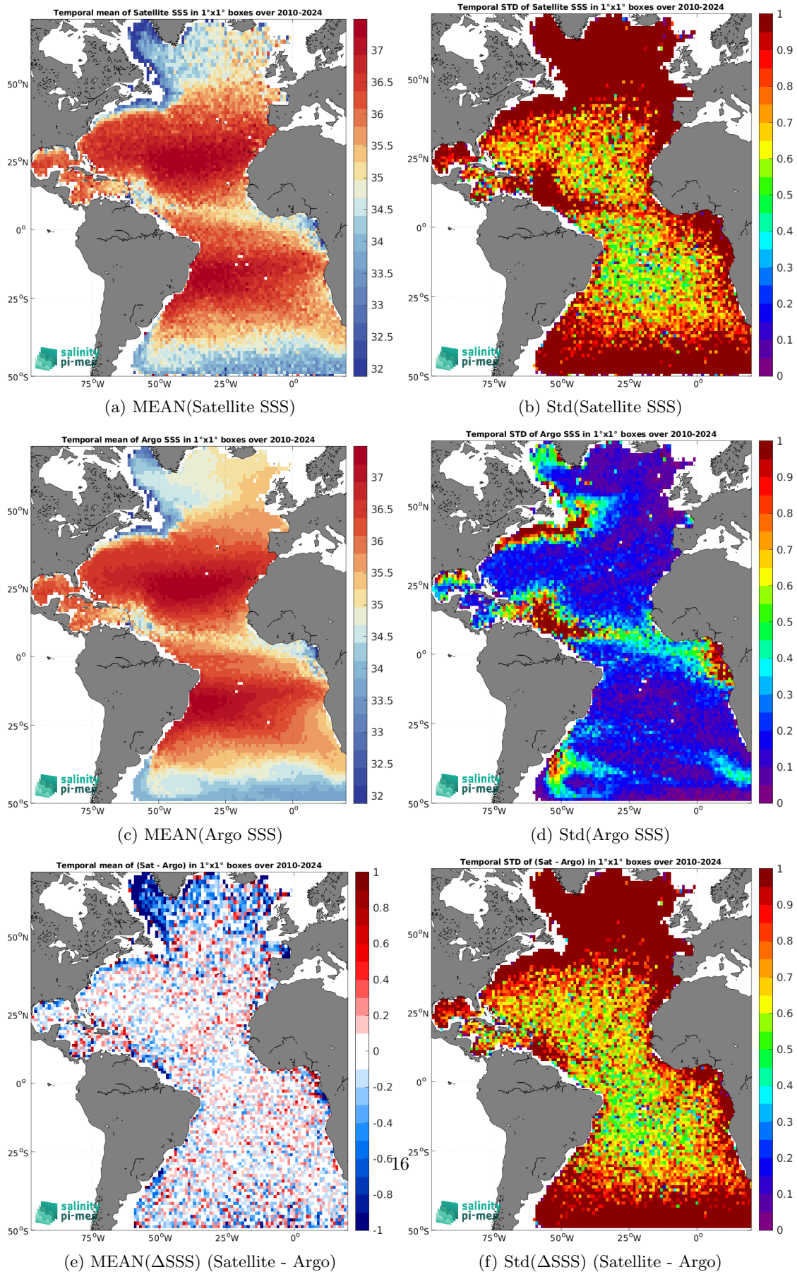
Figure 7: Temporal mean (left) and Std (right) of SSS from SMOS SSS L2Q v331 - With FLAG (CMEMS-CATDS-CPDC) (top), Argo (middle), and of \Delta SSS (Satellite - Argo). Only match-up pairs are used to generate these maps.
