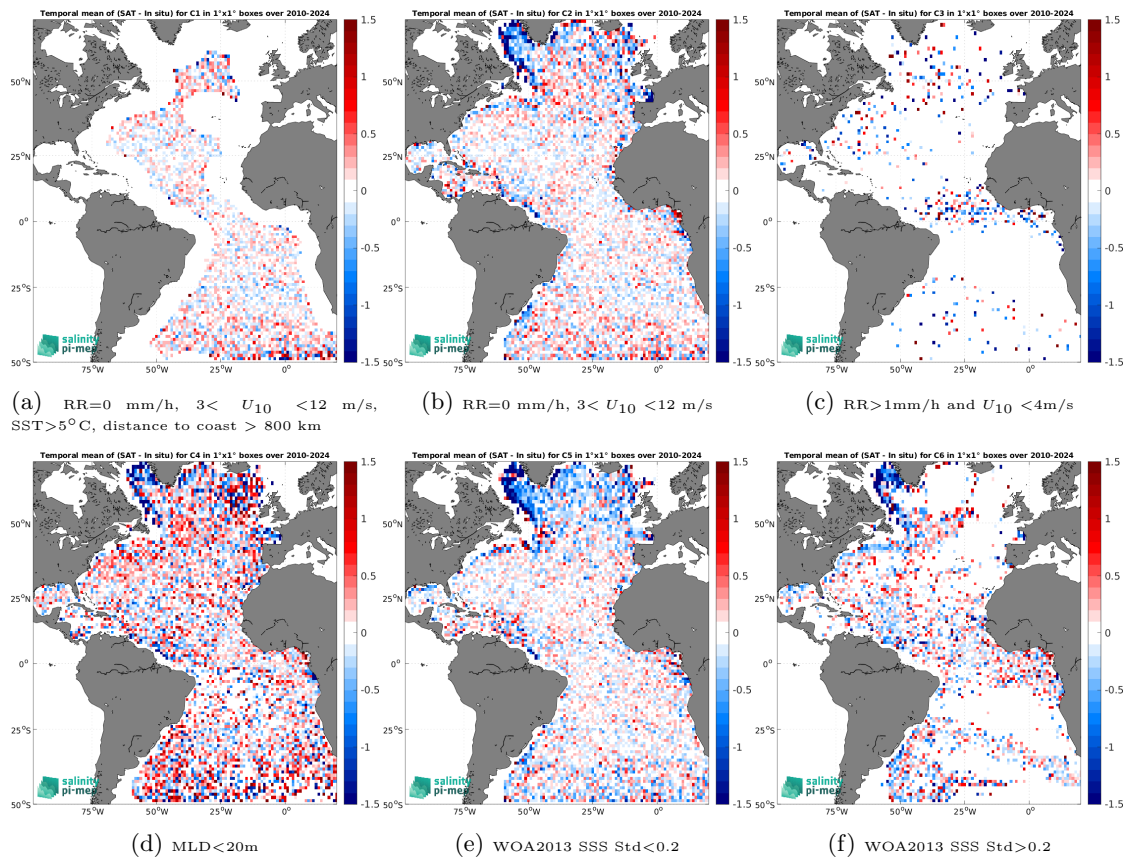
Figure 14: Temporal mean gridded over spatial boxes of size 1^\circ \times 1^\circ of \Delta SSS (SMOS SSS L2Q v331 - With FLAG (CMEMS-CATDS-CPDC) - Argo) for 6 different subdatasets corresponding to:RR=0 mm/h, 3 < U_{10} < 12 m/s, SST>5°C, distance to coast > 800 km (a), RR=0 mm/h, 3 < U_{10} < 12 m/s (b), RR>1mm/h and U_{10} < 4 m/s (c),MLD<20m (d),WOA2013 SSS Std<0.2 (e),WOA2013 SSS Std>0.2 (f).
