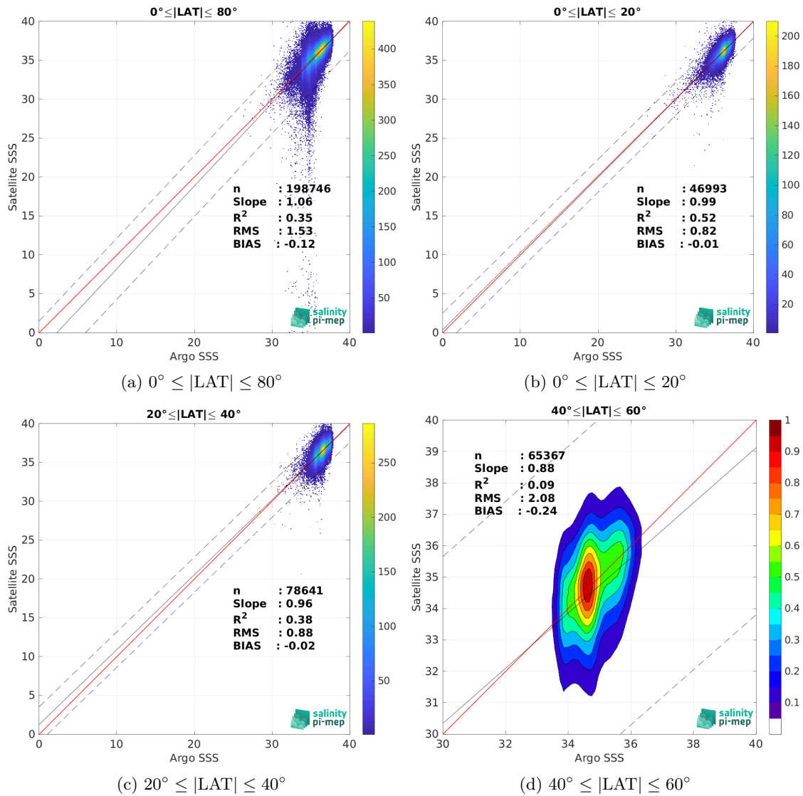
Figure 10: Contour maps of the concentration of SMOS SSS L2Q v331 - With FLAG (CMEMS-CATDS-CPDC) SSS ( y -axis) versus Argo SSS ( x -axis) at match-up pairs for different latitude bands. For each plot, the red line shows x=y . The black thin and dashed lines indicate a linear fit through the data cloud and the \pm 95\% confidence levels, respectively. The number match-up pairs n , the slope and R^2 coefficient of the linear fit, the root mean square (RMS) and the mean bias between satellite and in situ data are indicated for each latitude band in each plots.
