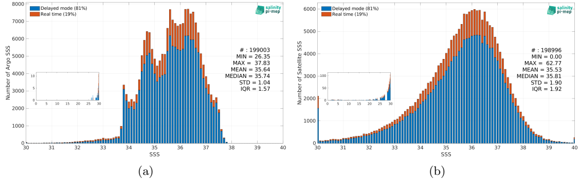
Figure 3: Histograms of SSS from Argo (a) and SMOS SSS L2Q v331 - With FLAG (CMEMS-CATDS-CPDC) (b) considering all match-up pairs per bins of 0.1 over the Atlantic Ocean Pi-MEP region and for the full satellite product period.
