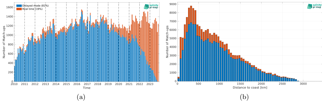
Figure 1: Number of match-ups between Argo and SMOS SSS L2Q v331 - With FLAG (CMEMS-CATDS-CPDC) SSS as a function of time (a) and as function of the distance to coast (b) over the Atlantic Ocean Pi-MEP region and for the full satellite product period.
