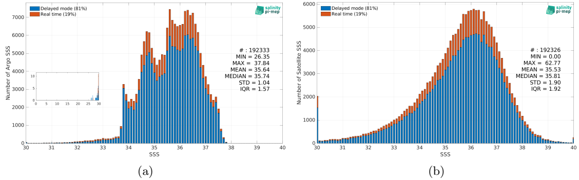
Figure 2: Histograms of SSS from Argo (a) and SMOS SSS L2Q v331 - With FLAG (CMEMS-CATDS-CPDC) (b) considering all match-up pairs per bins of 0.1 over the Atlantic Ocean Pi-MEP region and for the full satellite product period.
