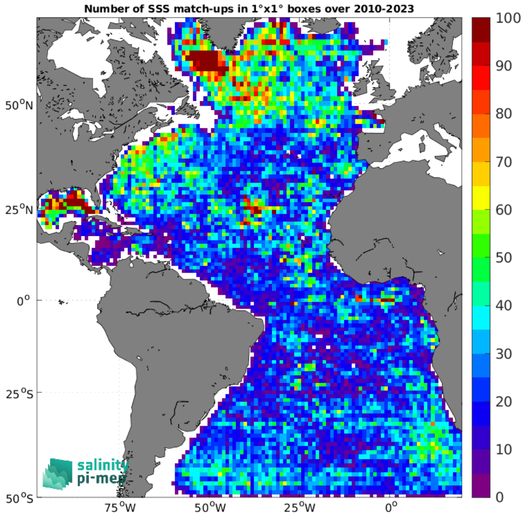
Figure 4: Number of SSS match-ups between Argo SSS and the SMOS SSS L2Q v331 - With FLAG (CMEMS-CATDS-CPDC) SSS product for the Atlantic Ocean Pi-MEP region over 1^\circ \times 1^\circ boxes and for the full satellite product period.
