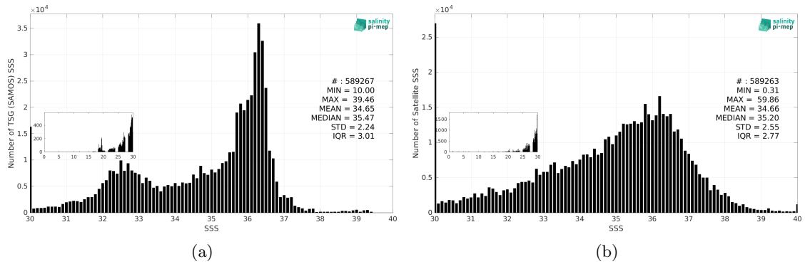
Figure 3: Histograms of SSS from TSG (SAMOS) (a) and SMOS SSS L2Q v331 - No FLAG (CMEMS-CATDS-CPDC) (b) considering all match-up pairs per bins of 0.1 over the Atlantic Ocean Pi-MEP region and for the full satellite product period.
