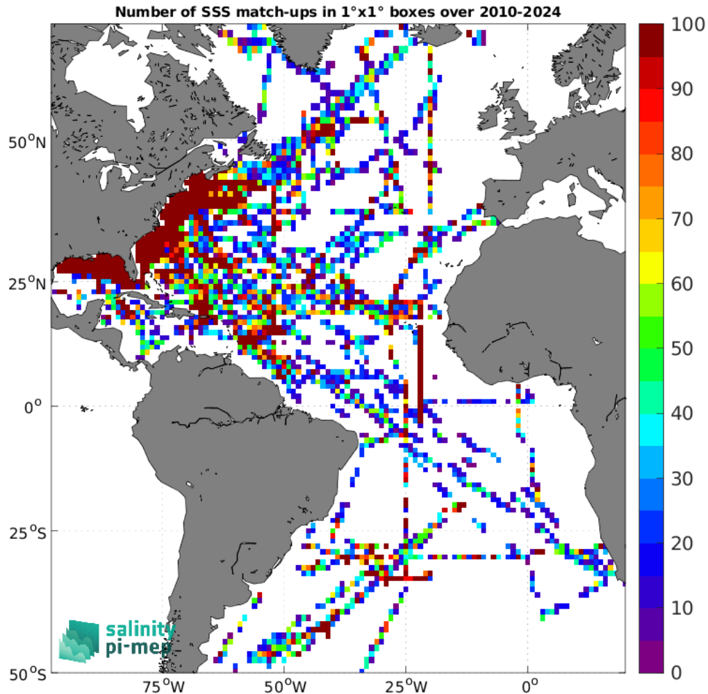
Figure 5: Number of SSS match-ups between TSG (SAMOS) SSS and the SMOS SSS L2Q v331 - No FLAG (CMEMS-CATDS-CPDC) SSS product for the Atlantic Ocean Pi-MEP region over 1^\circ \times 1^\circ boxes and for the full satellite product period.
