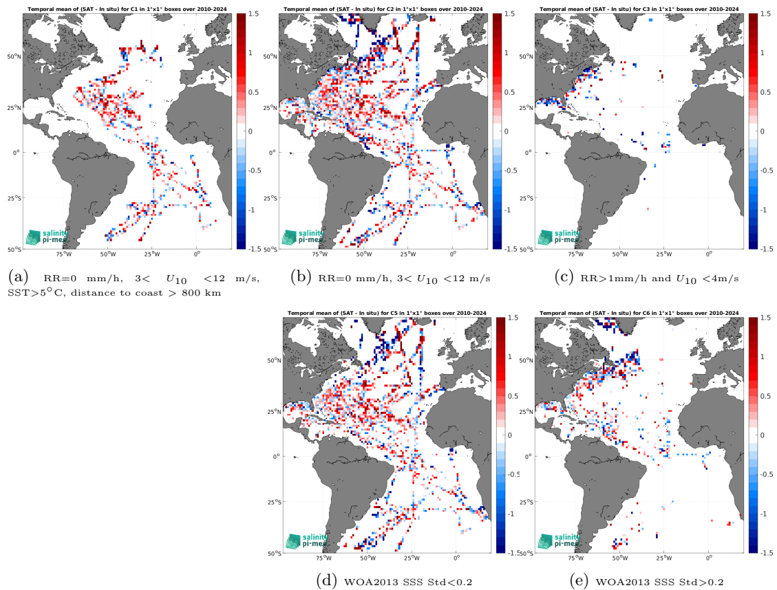
Figure 14: Temporal mean gridded over spatial boxes of size 1^\circ \times 1^\circ of \Delta\text{SSS} (SMOS SSS L2Q v331 - No FLAG (CMEMS-CATDS-CPDC) - TSG (SAMOS)) for 5 different subdatasets corresponding to:RR=0 mm/h, 3 < U_{10} < 12 m/s, SST>5°C, distance to coast > 800 km (a), RR=0 mm/h, 3 < U_{10} < 12 m/s (b), RR>1mm/h and U_{10} < 4 m/s (c), WOA2013 SSS Std<0.2 (d), WOA2013 SSS Std>0.2 (e).
