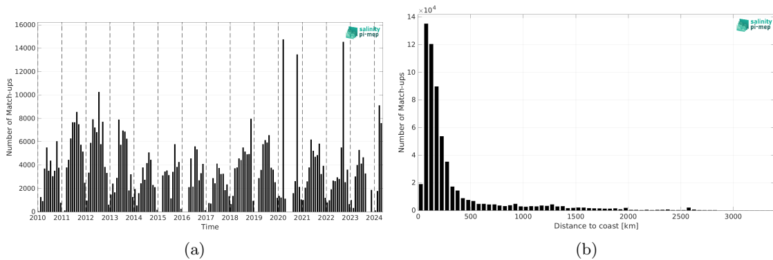
Figure 2: Number of match-ups between TSG (SAMOS) and SMOS SSS L2Q v331 - No FLAG (CMEMS-CATDS-CPDC) SSS as a function of time (a) and as function of the distance to coast (b) over the Atlantic Ocean Pi-MEP region and for the full satellite product period.
