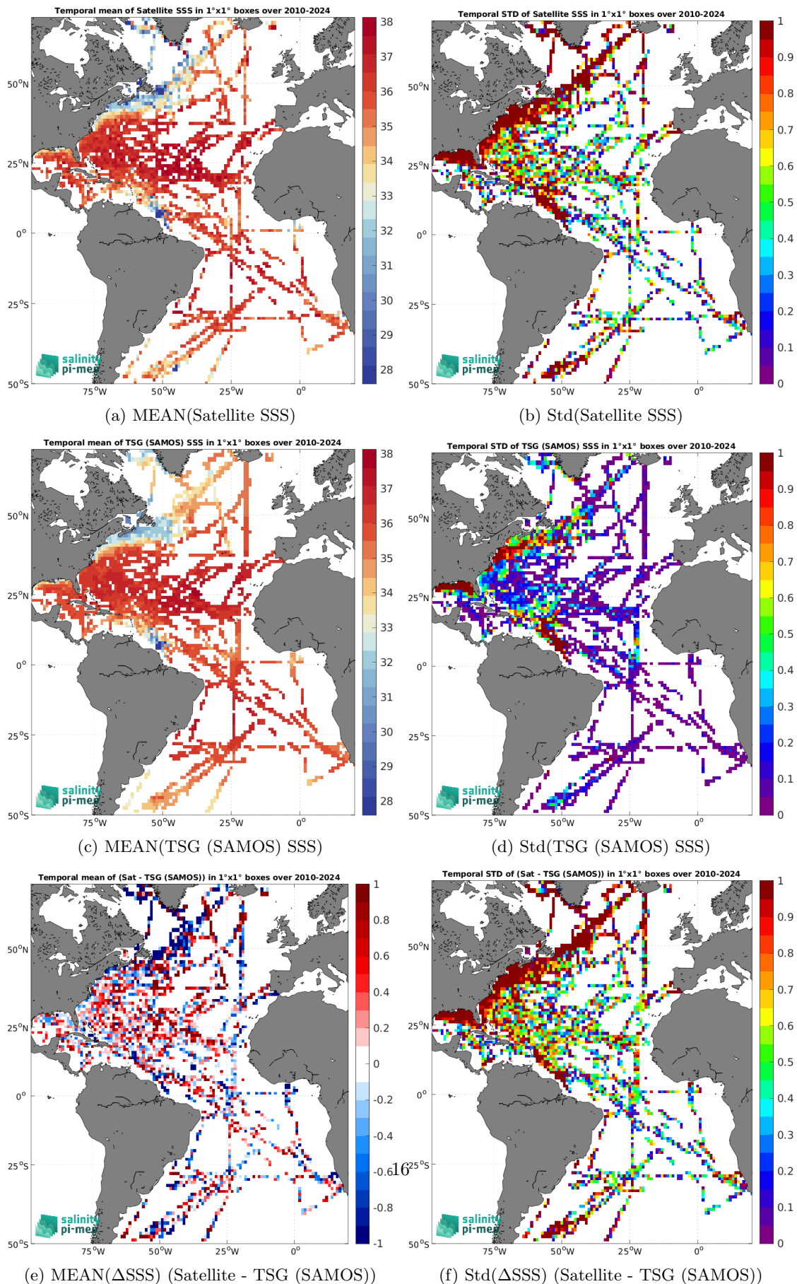
Figure 7: Temporal mean (left) and Std (right) of SSS from SMOS SSS L2Q v331 - No FLAG (CMEMS-CATDS-CPDC) (top), TSG (SAMOS) (middle), and of \Delta SSS (Satellite - TSG (SAMOS)). Only match-up pairs are used to generate these maps.
