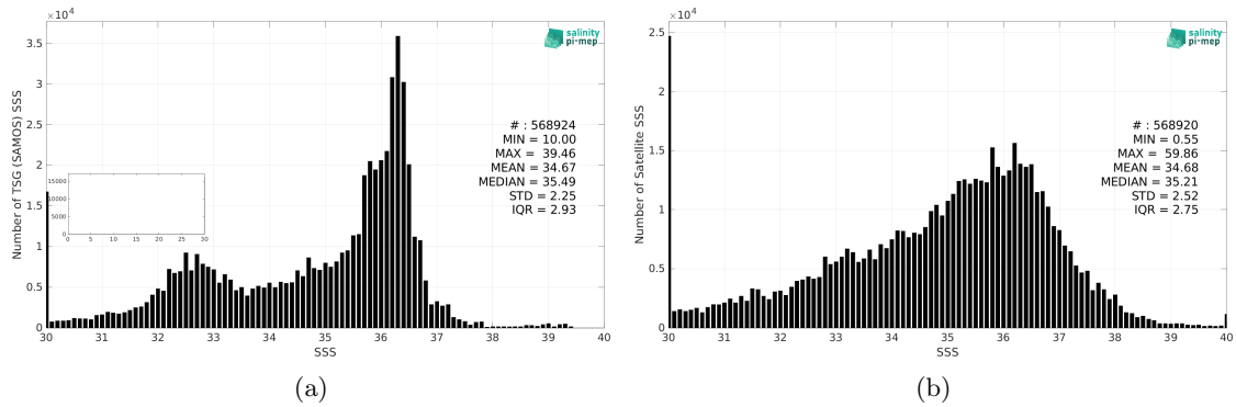
Figure 2: Histograms of SSS from TSG (SAMOS) (a) and SMOS SSS L2Q v331 - No FLAG (CMEMS-CATDS-CPDC) (b) considering all match-up pairs per bins of 0.1 over the Atlantic Ocean Pi-MEP region and for the full satellite product period.
