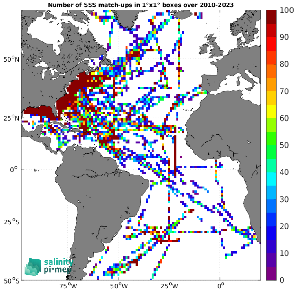
Figure 4: Number of SSS match-ups between TSG (SAMOS) SSS and the SMOS SSS L2Q v331 - No FLAG (CMEMS-CATDS-CPDC) SSS product for the Atlantic Ocean Pi-MEP region over 1^\circ \times 1^\circ boxes and for the full satellite product period.
