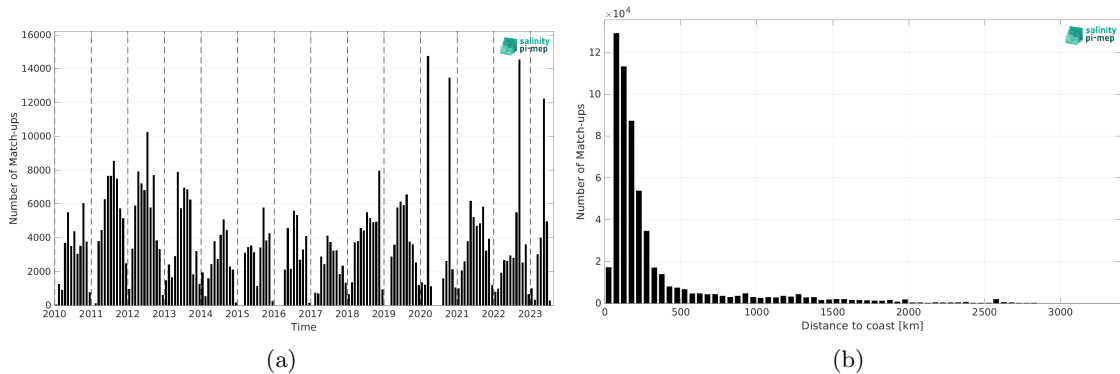
Figure 1: Number of match-ups between TSG (SAMOS) and SMOS SSS L2Q v331 - No FLAG (CMEMS-CATDS-CPDC) SSS as a function of time (a) and as function of the distance to coast (b) over the Atlantic Ocean Pi-MEP region and for the full satellite product period.
