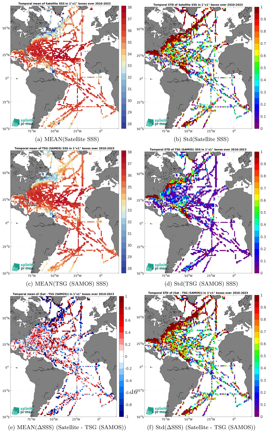
Figure 6: Temporal mean (left) and Std (right) of SSS from SMOS SSS L2Q v331 - No FLAG (CMEMS-CATDS-CPDC) (top), TSG (SAMOS) (middle), and of \Delta SSS (Satellite - TSG (SAMOS)). Only match-up pairs are used to generate these maps.
