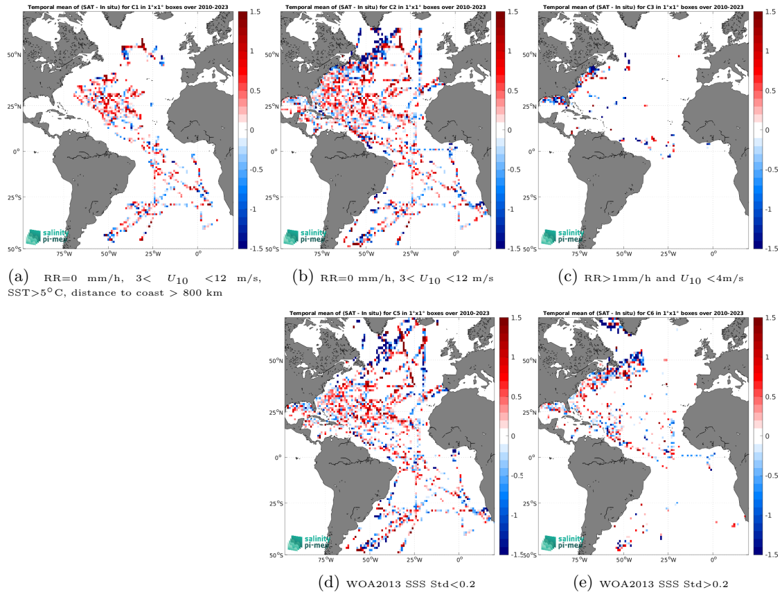
Figure 12: Temporal mean gridded over spatial boxes of size 1^\circ \times 1^\circ of \Delta\text{SSS} (SMOS SSS L2Q v331 - No FLAG (CMEMS-CATDS-CPDC) - TSG (SAMOS)) for 5 different subdatasets corresponding to:RR=0 mm/h, 3 < U_{10} < 12 m/s, SST >5^\circ\text{C} , distance to coast > 800 km (a), RR=0 mm/h, 3 < U_{10} < 12 m/s (b), RR >1 mm/h and U_{10} < 4 m/s (c), WOA2013 SSS Std <0.2 (d), WOA2013 SSS Std >0.2 (e).
