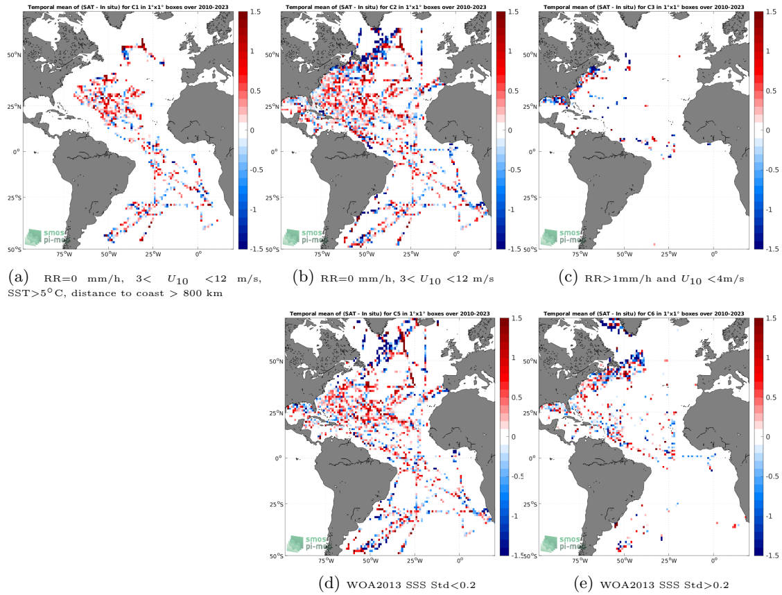
Figure 12: Temporal mean gridded over spatial boxes of size 1^\circ \times 1^\circ of \Delta\text{SSS} (SMOS SSS L2Q v331 - No FLAG (CMEMS-CATDS-CPDC) - TSG (SAMOS)) for 5 different subdatasets corresponding to:RR=0 mm/h, 3 < U_{10} < 12 m/s, SST >5^\circ\text{C} , distance to coast > 800 km (a), RR=0 mm/h, 3 < U_{10} < 12 m/s (b), RR >1 mm/h and U_{10} < 4 m/s (c), WOA2013 SSS Std <0.2 (d), WOA2013 SSS Std >0.2 (e).
