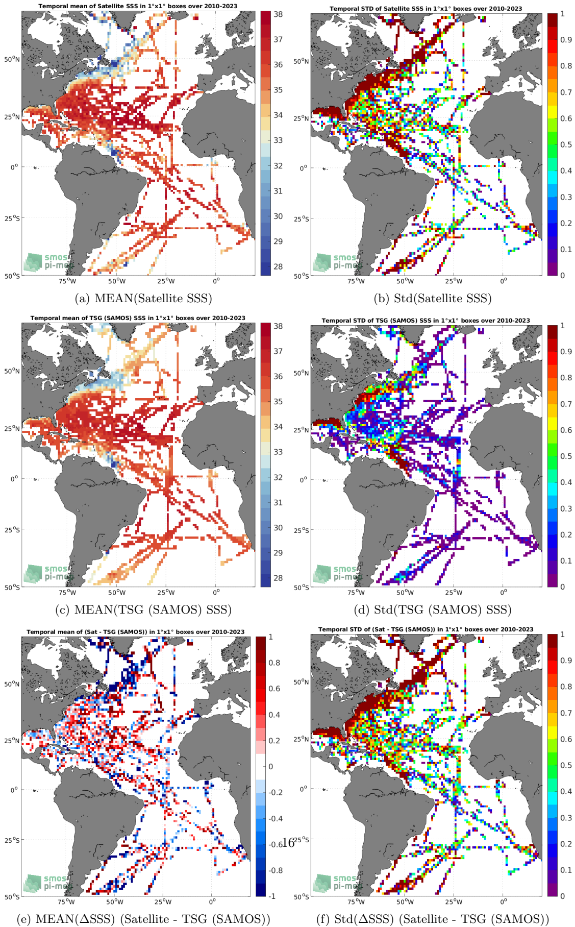
(e) MEAN( \Delta SSS) (Satellite - TSG (SAMOS)) (f) Std( \Delta SSS) (Satellite - TSG (SAMOS)) Figure 6: Temporal mean (left) and Std (right) of SSS from SMOS SSS L2Q v331 - No FLAG (CMEMS-CATDS-CPDC) (top), TSG (SAMOS) (middle), and of \Delta SSS (Satellite - TSG (SAMOS)). Only match-up pairs are used to generate these maps.
