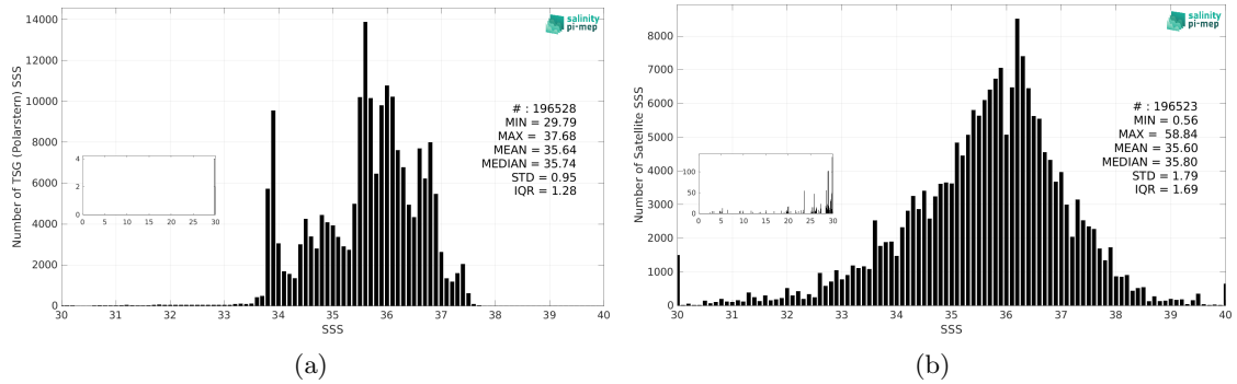
Figure 3: Histograms of SSS from TSG (Polarstern) (a) and SMOS SSS L2Q v331 - No FLAG (CMEMS-CATDS-CPDC) (b) considering all match-up pairs per bins of 0.1 over the Atlantic Ocean Pi-MEP region and for the full satellite product period.
