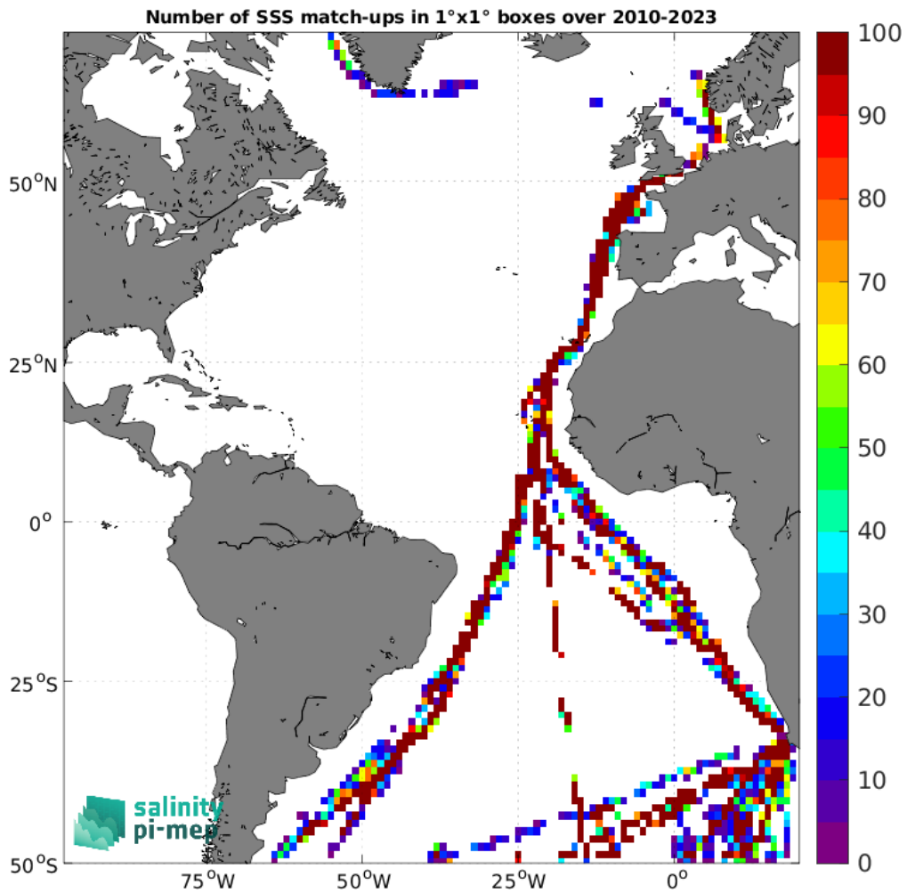
Figure 5: Number of SSS match-ups between TSG (Polarstern) SSS and the SMOS SSS L2Q v331 - No FLAG (CMEMS-CATDS-CPDC) SSS product for the Atlantic Ocean Pi-MEP region over 1°x1° boxes and for the full satellite product period.
