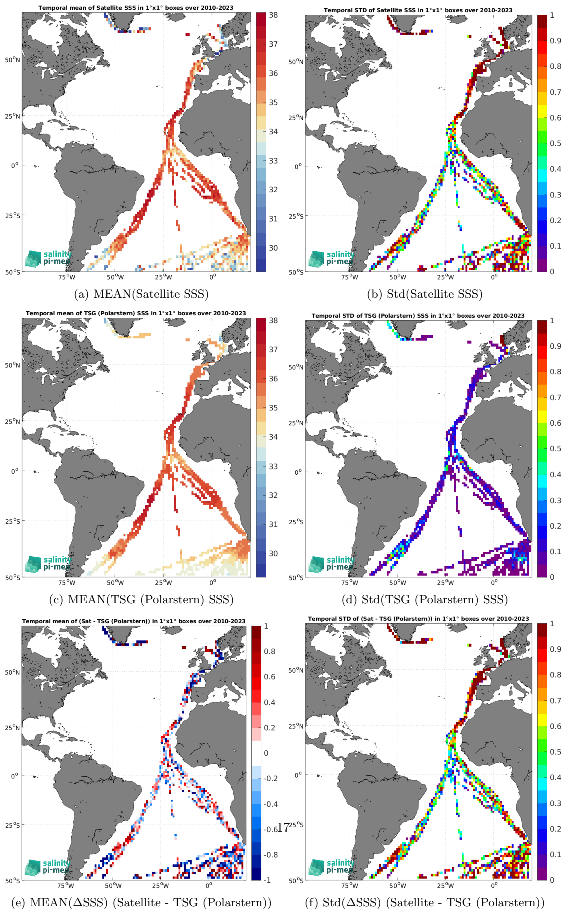
Figure 7: Temporal mean (left) and Std (right) of SSS from SMOS SSS L2Q v331 - No FLAG (CMEMS-CATDS-CPDC) (top), TSG (Polarstern) (middle), and of \Delta SSS (Satellite - TSG (Polarstern)). Only match-up pairs are used to generate these maps.
