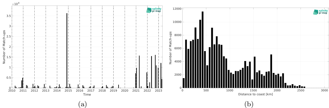
Figure 2: Number of match-ups between TSG (Polarstern) and SMOS SSS L2Q v331 - No FLAG (CMEMS-CATDS-CPDC) SSS as a function of time (a) and as function of the distance to coast (b) over the Atlantic Ocean Pi-MEP region and for the full satellite product period.
