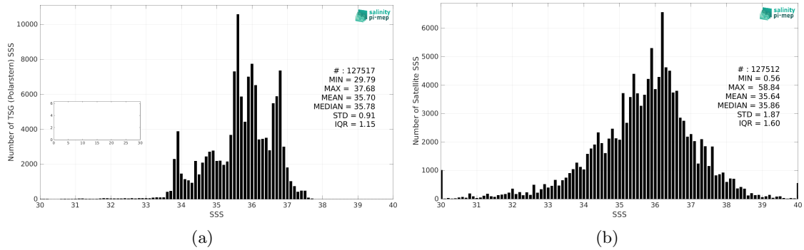
Figure 2: Histograms of SSS from TSG (Polarstern) (a) and SMOS SSS L2Q v331 - No FLAG (CMEMS-CATDS-CPDC) (b) considering all match-up pairs per bins of 0.1 over the Atlantic Ocean Pi-MEP region and for the full satellite product period.
