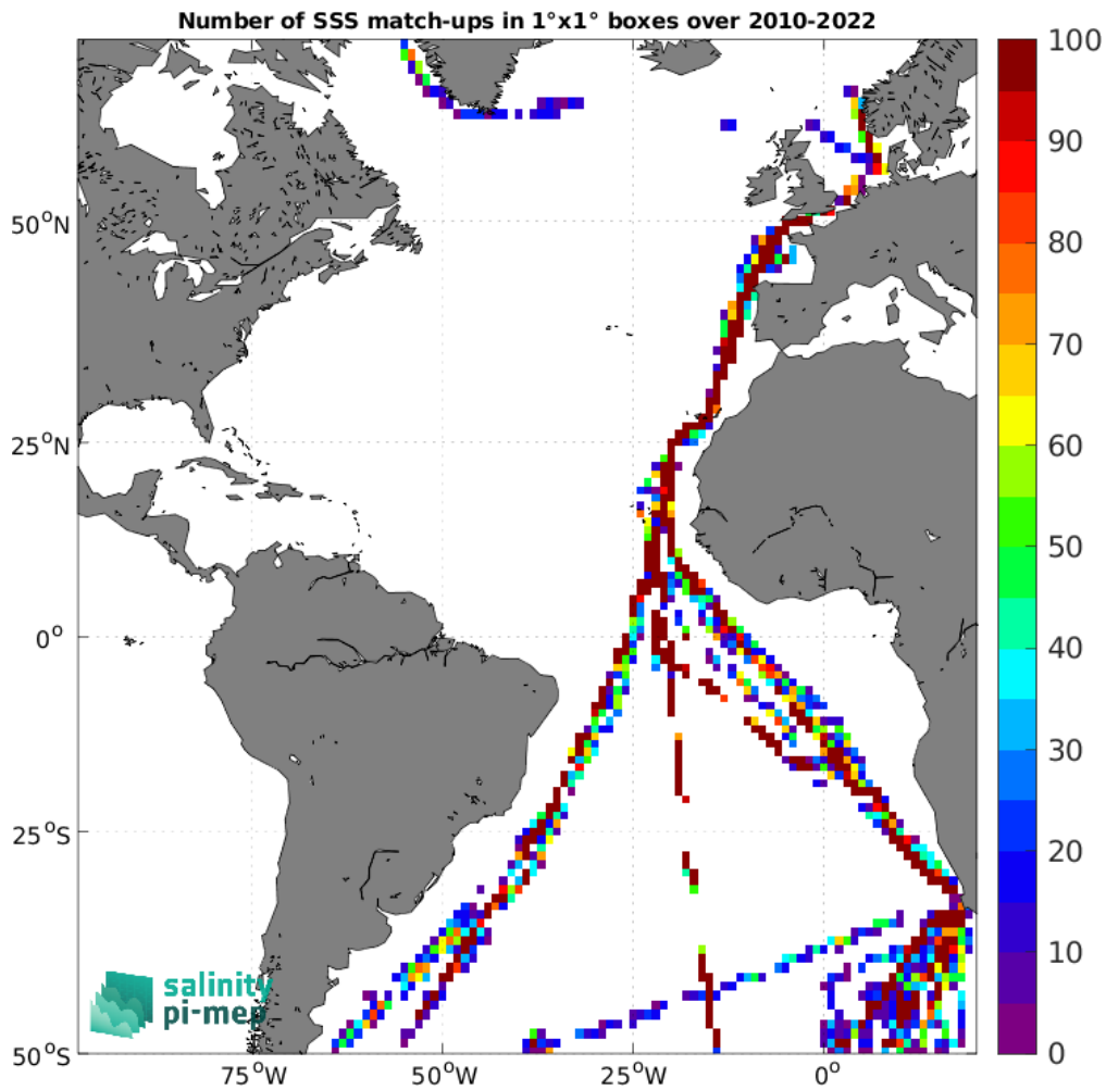
Figure 4: Number of SSS match-ups between TSG (Polarstern) SSS and the SMOS SSS L2Q v331 - No FLAG (CMEMS-CATDS-CPDC) SSS product for the Atlantic Ocean Pi-MEP region over 1°x1° boxes and for the full satellite product period.
