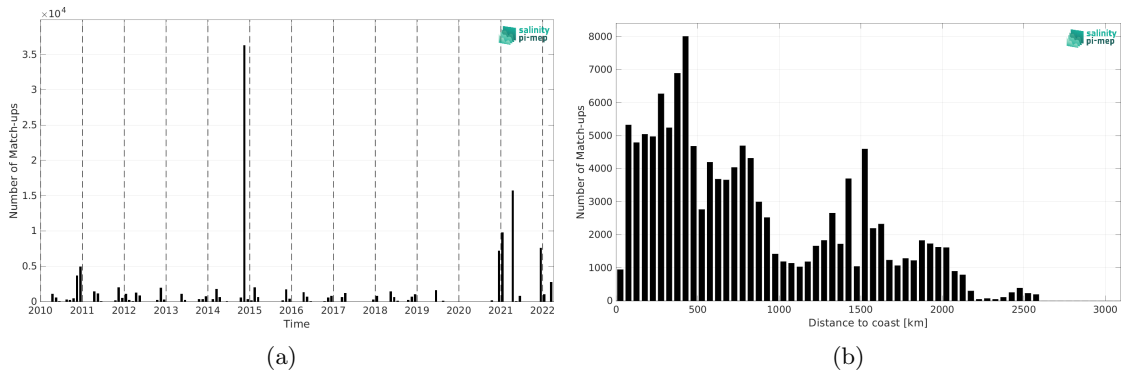
Figure 1: Number of match-ups between TSG (Polarstern) and SMOS SSS L2Q v331 - No FLAG (CMEMS-CATDS-CPDC) SSS as a function of time (a) and as function of the distance to coast (b) over the Atlantic Ocean Pi-MEP region and for the full satellite product period.
