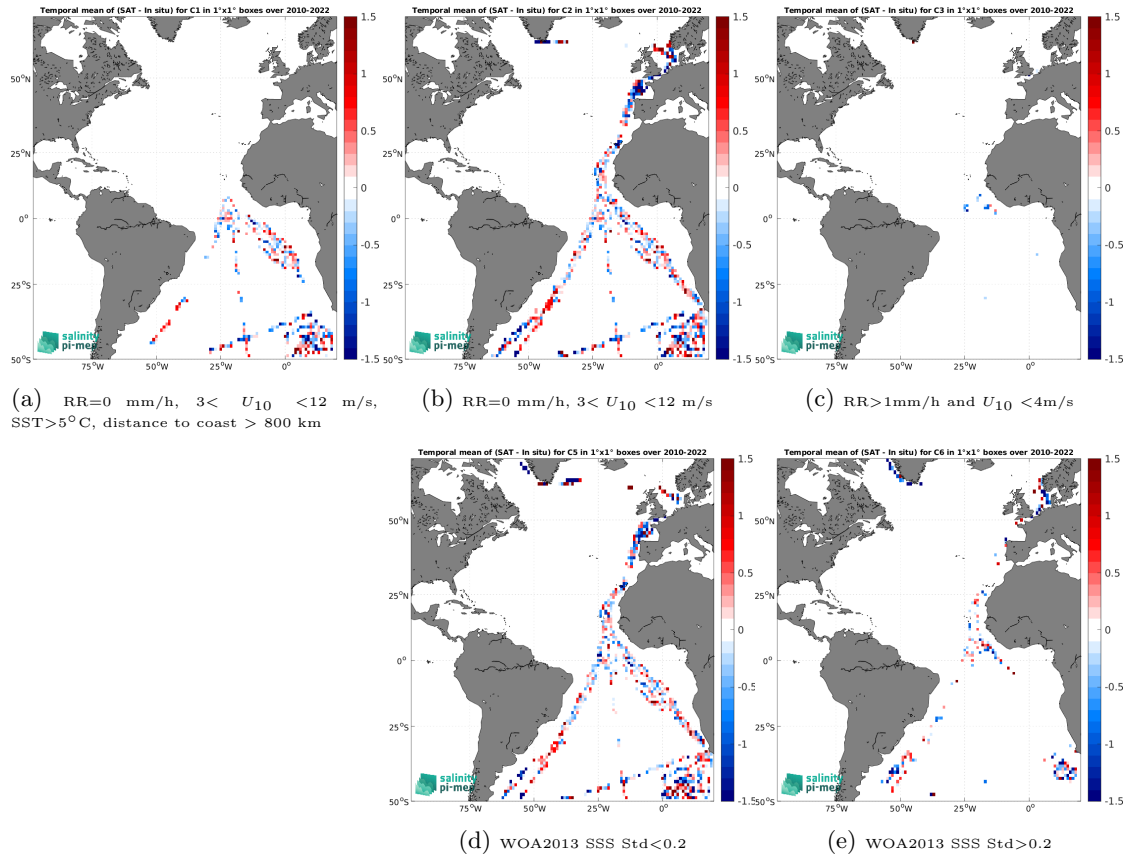
Figure 12: Temporal mean gridded over spatial boxes of size 1^\circ \times 1^\circ of \Delta SSS (SMOS SSS L2Q v331 - No FLAG (CMEMS-CATDS-CPDC) - TSG (Polarstern)) for 5 different subdatasets corresponding to:RR=0 mm/h, 3 < U_{10} < 12 m/s, SST >5^\circ\text{C} , distance to coast > 800 km (a), RR=0 mm/h, 3 < U_{10} < 12 m/s (b), RR >1 mm/h and U_{10} < 4 m/s (c), WOA2013 SSS Std <0.2 (d), WOA2013 SSS Std >0.2 (e).
