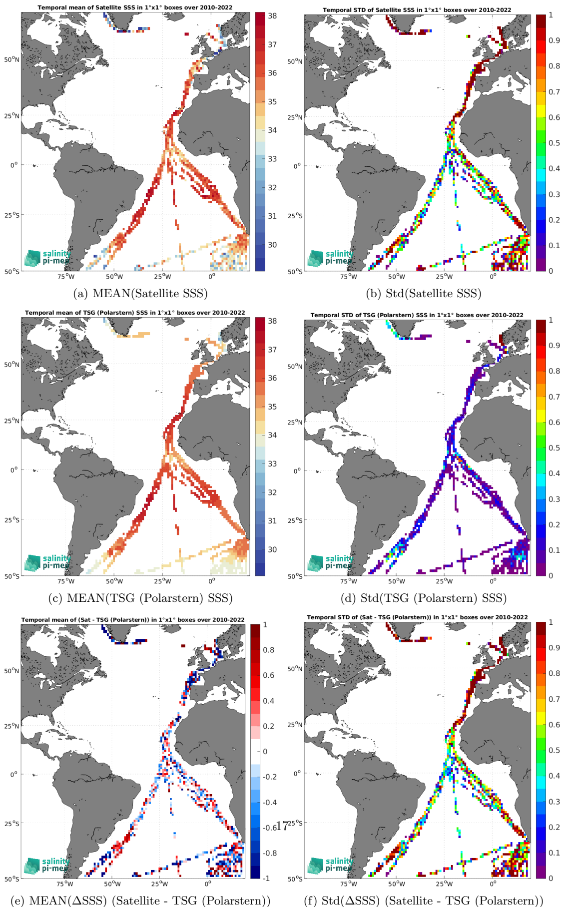
Figure 6: Temporal mean (left) and Std (right) of SSS from SMOS SSS L2Q v331 - No FLAG (CMEMS-CATDS-CPDC) (top), TSG (Polarstern) (middle), and of \Delta SSS (Satellite - TSG (Polarstern)). Only match-up pairs are used to generate these maps.
