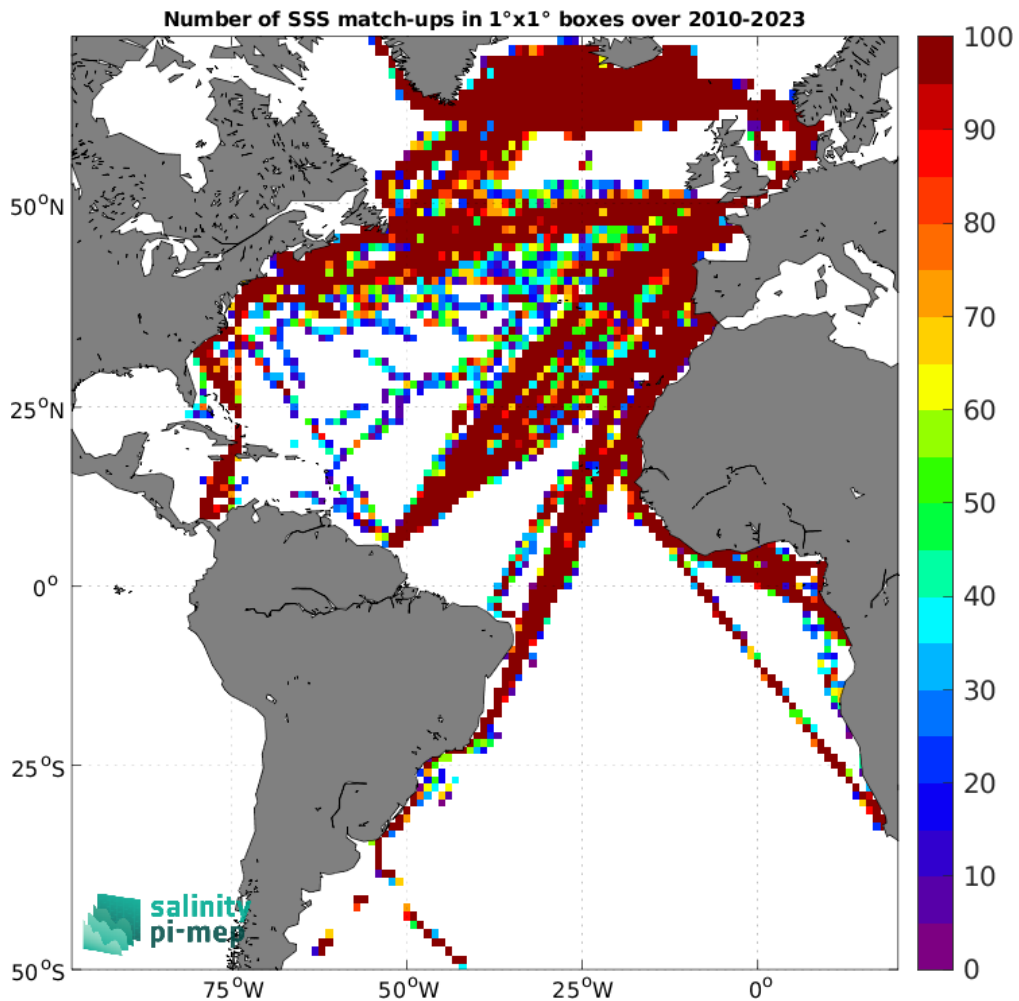
Figure 5: Number of SSS match-ups between TSG (LEGOS-DM) SSS and the SMOS SSS L2Q v331 - No FLAG (CMEMS-CATDS-CPDC) SSS product for the Atlantic Ocean Pi-MEP region over 1^\circ \times 1^\circ boxes and for the full satellite product period.
