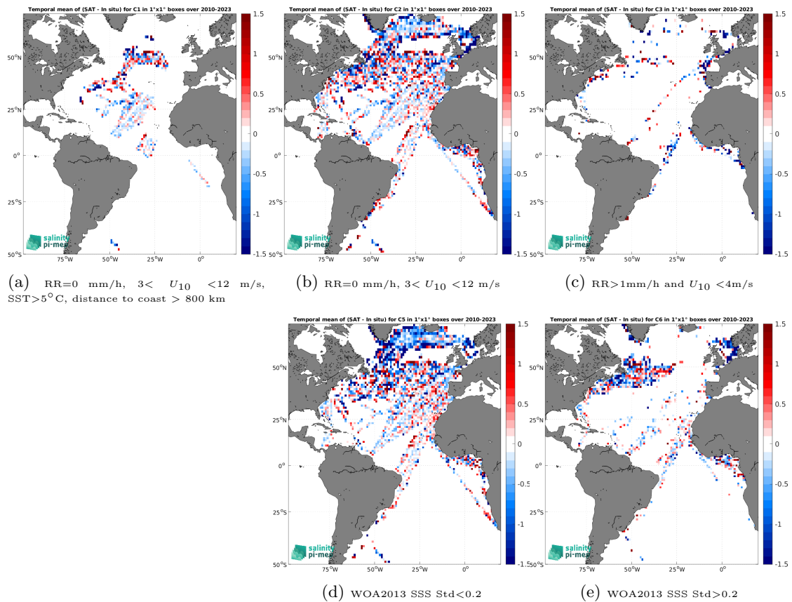
Figure 14: Temporal mean gridded over spatial boxes of size 1^\circ \times 1^\circ of \Delta\text{SSS} (SMOS SSS L2Q v331 - No FLAG (CMEMS-CATDS-CPDC) - TSG (LEGOS-DM)) for 5 different subdatasets corresponding to:RR=0 mm/h, 3 < U_{10} < 12 m/s, SST>5°C, distance to coast > 800 km (a), RR=0 mm/h, 3 < U_{10} < 12 m/s (b), RR>1mm/h and U_{10} < 4 m/s (c), WOA2013 SSS Std<0.2 (d), WOA2013 SSS Std>0.2 (e).
