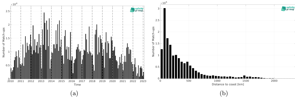
Figure 2: Number of match-ups between TSG (LEGOS-DM) and SMOS SSS L2Q v331 - No FLAG (CMEMS-CATDS-CPDC) SSS as a function of time (a) and as function of the distance to coast (b) over the Atlantic Ocean Pi-MEP region and for the full satellite product period.
