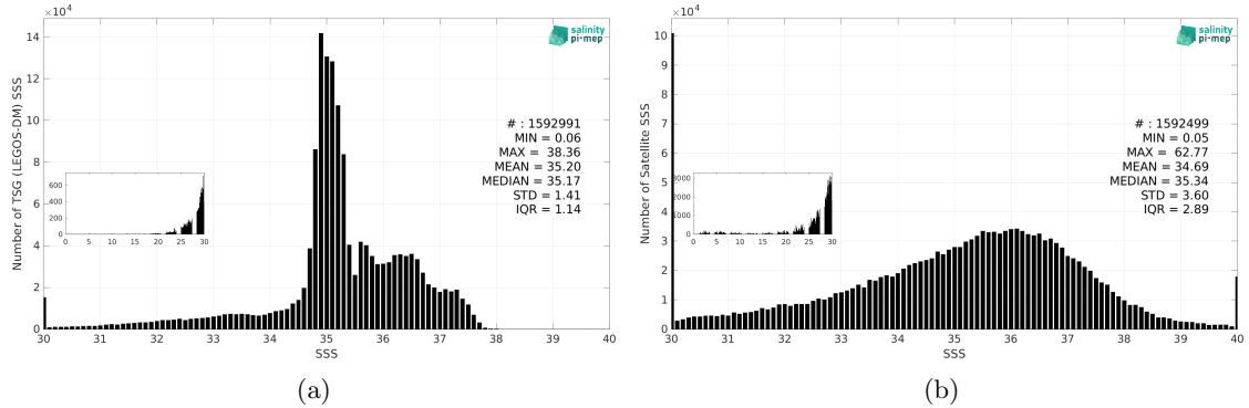
Figure 3: Histograms of SSS from TSG (LEGOS-DM) (a) and SMOS SSS L2Q v331 - No FLAG (CMEMS-CATDS-CPDC) (b) considering all match-up pairs per bins of 0.1 over the Atlantic Ocean Pi-MEP region and for the full satellite product period.
