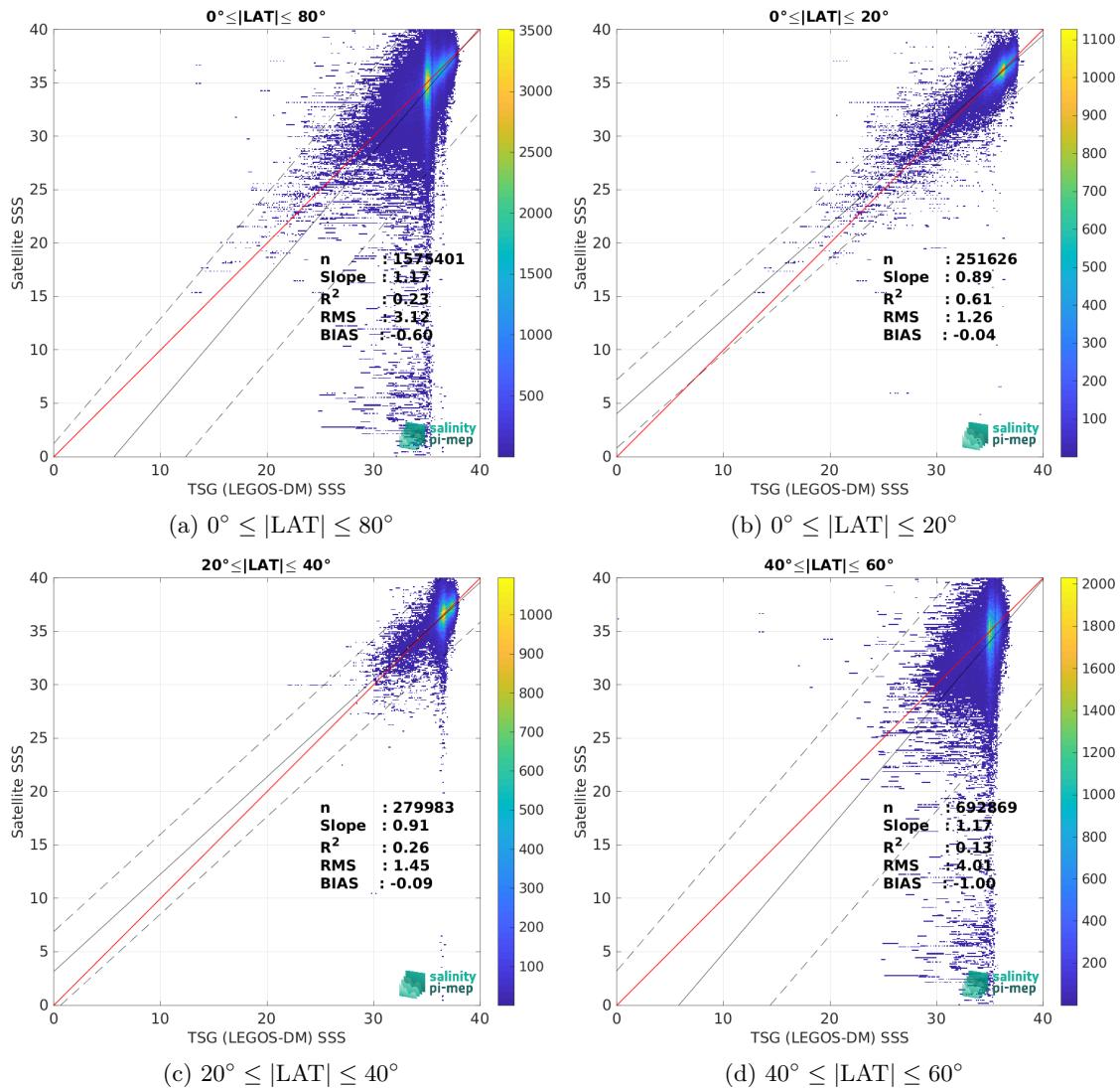
Figure 10: Contour maps of the concentration of SMOS SSS L2Q v331 - No FLAG (CMEMS-CATDS-CPDC) SSS (y-axis) versus TSG (LEGOS-DM) SSS (x-axis) at match-up pairs for different latitude bands. For each plot, the red line shows x=y . The black thin and dashed lines indicate a linear fit through the data cloud and the \pm 95\% confidence levels, respectively. The number match-up pairs n , the slope and R^2 coefficient of the linear fit, the root mean square (RMS) and the mean bias between satellite and in situ data are indicated for each latitude band in each plots.
