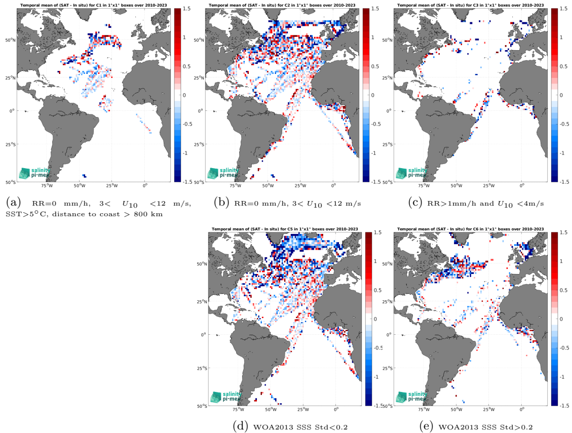
Figure 12: Temporal mean gridded over spatial boxes of size 1^\circ \times 1^\circ of \Delta\text{SSS} (SMOS SSS L2Q v331 - No FLAG (CMEMS-CATDS-CPDC) - TSG (LEGOS-DM)) for 5 different subdatasets corresponding to:RR=0 mm/h, 3 < U_{10} < 12 m/s, SST >5^\circ\text{C} , distance to coast > 800 km (a), RR=0 mm/h, 3 < U_{10} < 12 m/s (b), RR >1 mm/h and U_{10} < 4 m/s (c), WOA2013 SSS Std <0.2 (d), WOA2013 SSS Std >0.2 (e).
