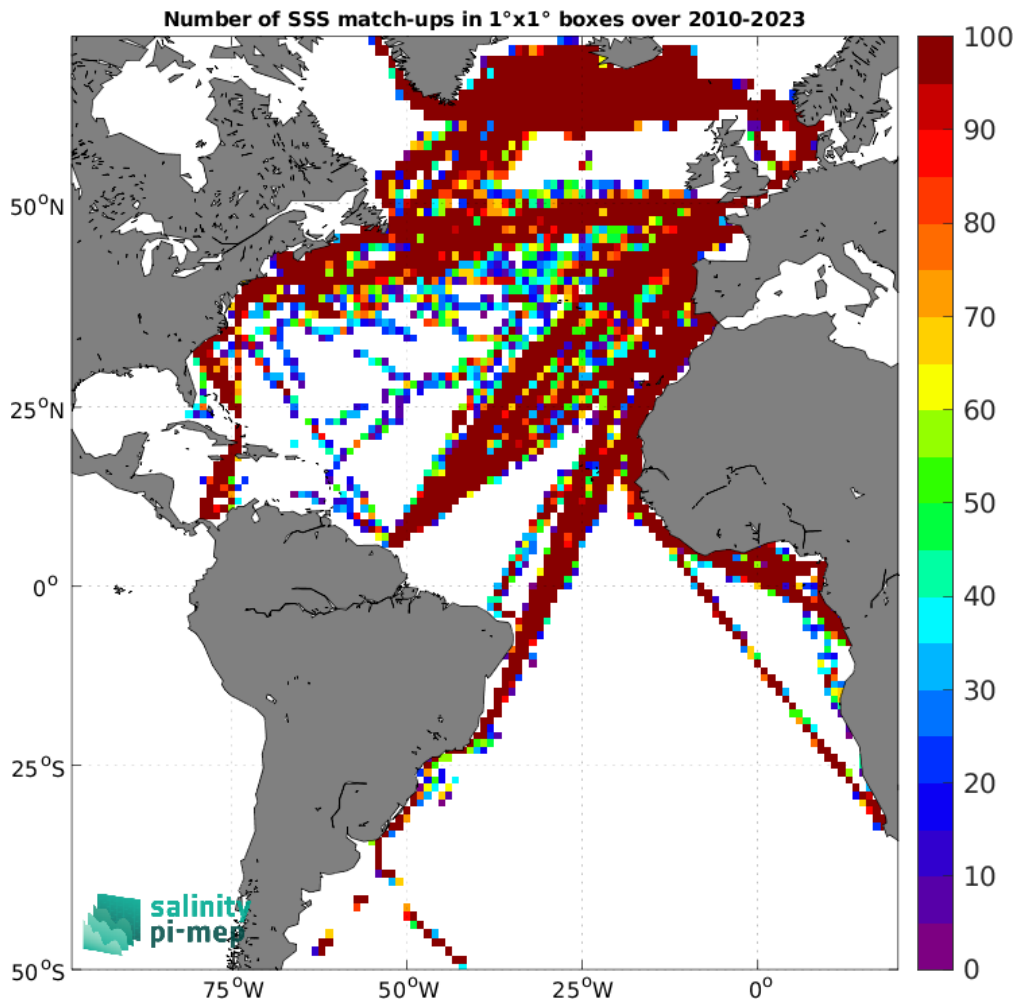
Figure 4: Number of SSS match-ups between TSG (LEGOS-DM) SSS and the SMOS SSS L2Q v331 - No FLAG (CMEMS-CATDS-CPDC) SSS product for the Atlantic Ocean Pi-MEP region over 1^\circ \times 1^\circ boxes and for the full satellite product period.
