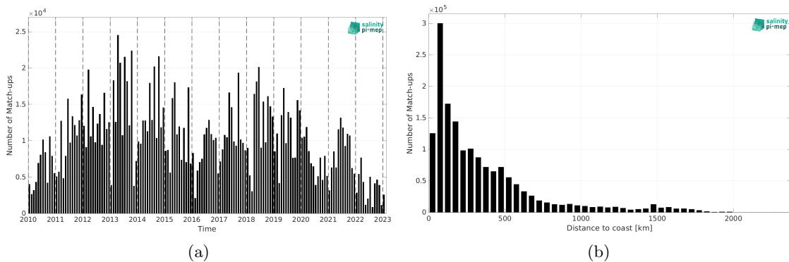
Figure 1: Number of match-ups between TSG (LEGOS-DM) and SMOS SSS L2Q v331 - No FLAG (CMEMS-CATDS-CPDC) SSS as a function of time (a) and as function of the distance to coast (b) over the Atlantic Ocean Pi-MEP region and for the full satellite product period.
