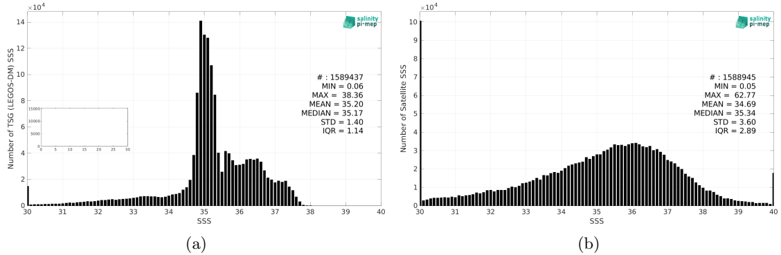
Figure 2: Histograms of SSS from TSG (LEGOS-DM) (a) and SMOS SSS L2Q v331 - No FLAG (CMEMS-CATDS-CPDC) (b) considering all match-up pairs per bins of 0.1 over the Atlantic Ocean Pi-MEP region and for the full satellite product period.
