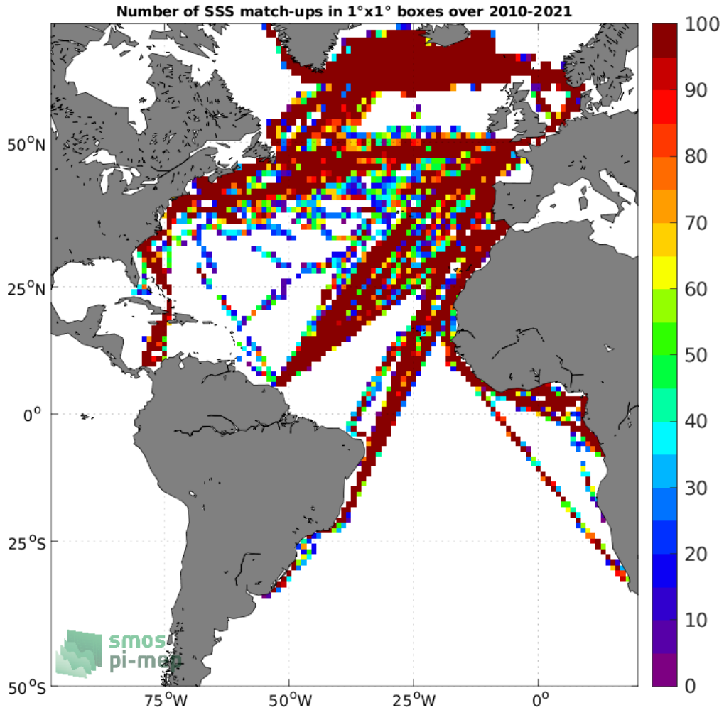
Figure 4: Number of SSS match-ups between TSG (LEGOS-DM) SSS and the SMOS SSS L2Q v331 - No FLAG (CMEMS-CATDS-CPDC) SSS product for the Atlantic Ocean Pi-MEP region over 1°x1° boxes and for the full satellite product period.
