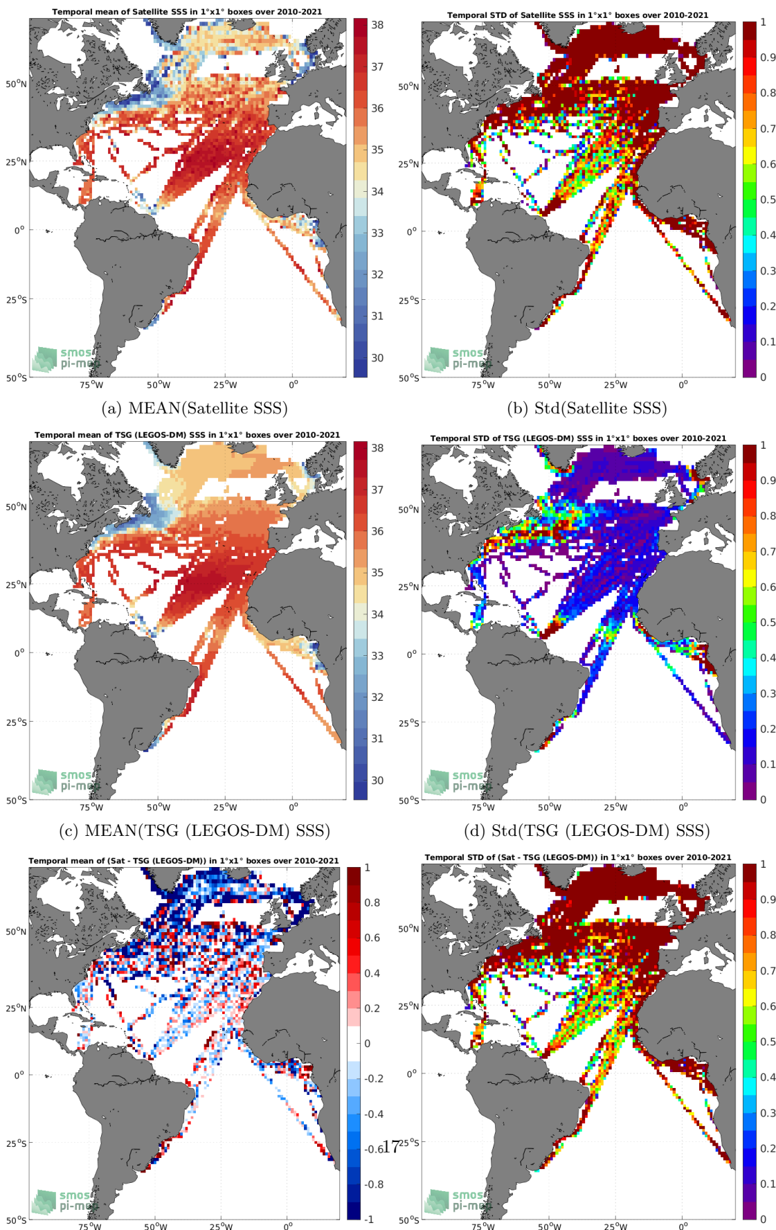
(e) MEAN( \Delta SSS) (Satellite - TSG (LEGOS-DM)) (f) Std( \Delta SSS) (Satellite - TSG (LEGOS-DM)) Figure 6: Temporal mean (left) and Std (right) of SSS from SMOS SSS L2Q v331 - No FLAG (CMEMS-CATDS-CPDC) (top), TSG (LEGOS-DM) (middle), and of \Delta SSS (Satellite - TSG (LEGOS-DM)). Only match-up pairs are used to generate these maps.
