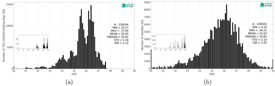
Figure 3: Histograms of SSS from TSG (GOSUD-Sailing-ship) (a) and SMOS SSS L2Q v331 - No FLAG (CMEMS-CATDS-CPDC) (b) considering all match-up pairs per bins of 0.1 over the Atlantic Ocean Pi-MEP region and for the full satellite product period.
