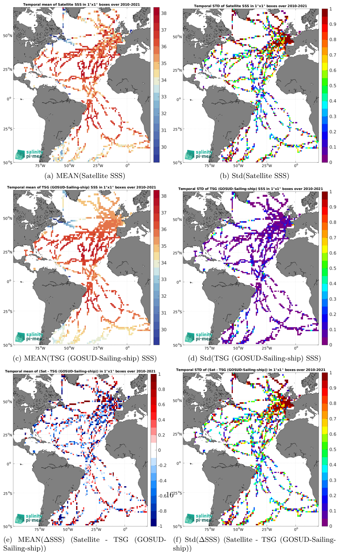
Figure 7: Temporal mean (left) and Std (right) of SSS from SMOS SSS L2Q v331 - No FLAG (CMEMS-CATDS-CPDC) (top), TSG (GOSUD-Sailing-ship) (middle), and of \Delta SSS (Satellite - TSG (GOSUD-Sailing-ship)). Only match-up pairs are used to generate these maps.
