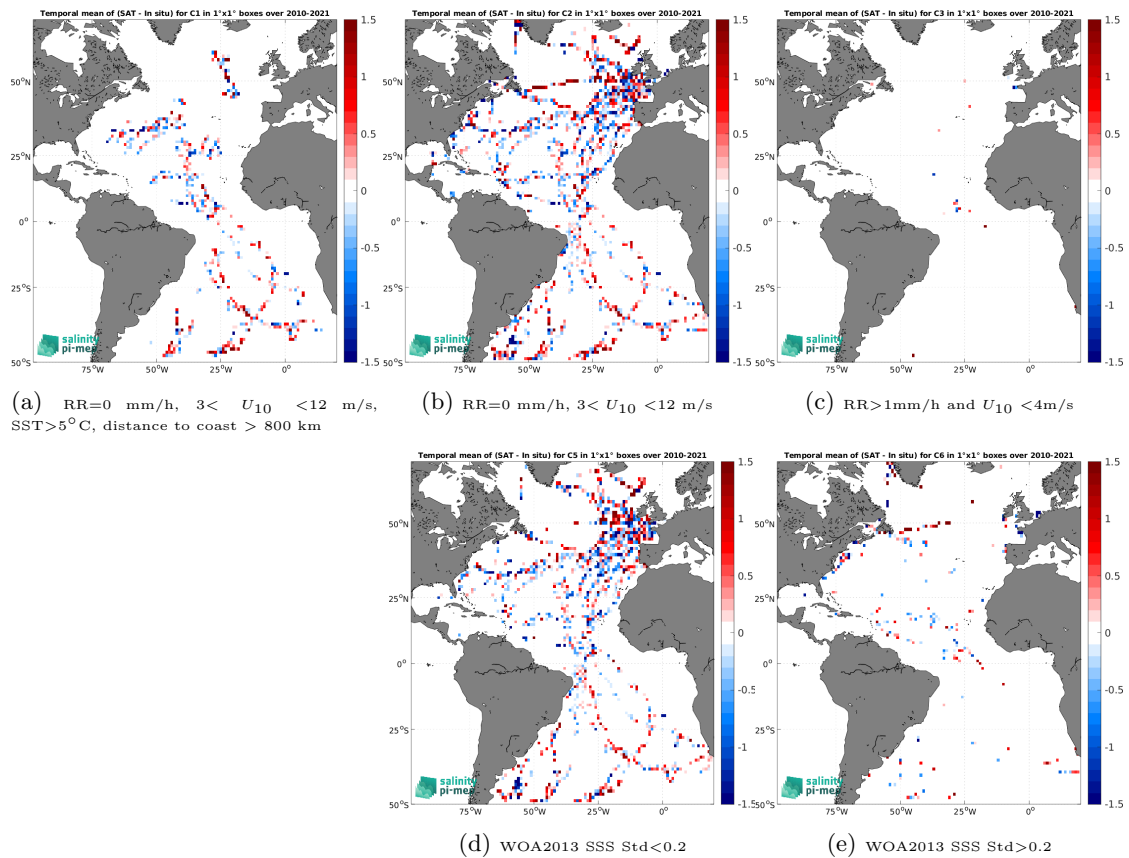
Figure 14: Temporal mean gridded over spatial boxes of size 1^\circ \times 1^\circ of \Delta\text{SSS} (SMOS SSS L2Q v331 - No FLAG (CMEMS-CATDS-CPDC) - TSG (GOSUD-Sailing-ship)) for 5 different sub-datasets corresponding to:RR=0 mm/h, 3 < U_{10} < 12 m/s, SST>5°C, distance to coast > 800 km (a), RR=0 mm/h, 3 < U_{10} < 12 m/s (b), RR>1mm/h and U_{10} < 4 m/s (c), WOA2013 SSS Std<0.2 (d), WOA2013 SSS Std>0.2 (e).
