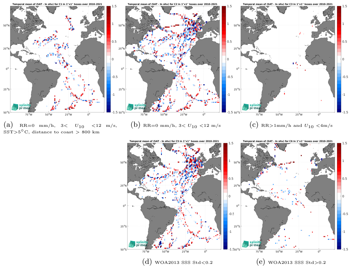
Figure 12: Temporal mean gridded over spatial boxes of size 1^\circ \times 1^\circ of \Delta\text{SSS} (SMOS SSS L2Q v331 - No FLAG (CMEMS-CATDS-CPDC) - TSG (GOSUD-Sailing-ship)) for 5 different sub-datasets corresponding to:RR=0 mm/h, 3 < U_{10} < 12 m/s, SST >5^\circ\text{C} , distance to coast > 800 km (a), RR=0 mm/h, 3 < U_{10} < 12 m/s (b), RR >1 mm/h and U_{10} < 4 m/s (c), WOA2013 SSS Std <0.2 (d), WOA2013 SSS Std >0.2 (e).
