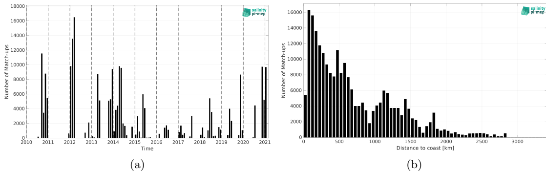
Figure 1: Number of match-ups between TSG (GOSUD-Sailing-ship) and SMOS SSS L2Q v331 - No FLAG (CMEMS-CATDS-CPDC) SSS as a function of time (a) and as function of the distance to coast (b) over the Atlantic Ocean Pi-MEP region and for the full satellite product period.
