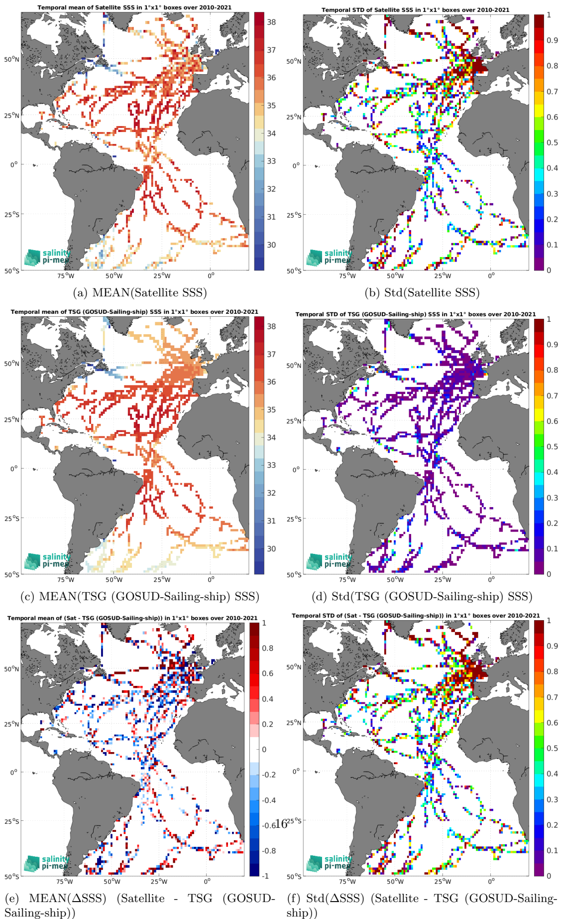
Figure 6: Temporal mean (left) and Std (right) of SSS from SMOS SSS L2Q v331 - No FLAG (CMEMS-CATDS-CPDC) (top), TSG (GOSUD-Sailing-ship) (middle), and of \Delta SSS (Satellite - TSG (GOSUD-Sailing-ship)). Only match-up pairs are used to generate these maps.
