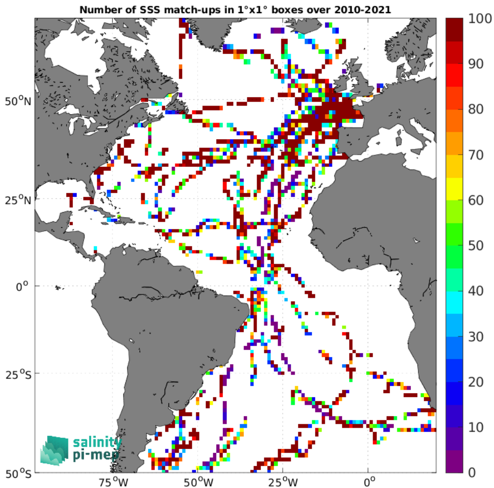
Figure 4: Number of SSS match-ups between TSG (GOSUD-Sailing-ship) SSS and the SMOS SSS L2Q v331 - No FLAG (CMEMS-CATDS-CPDC) SSS product for the Atlantic Ocean Pi-MEP region over 1^\circ \times 1^\circ boxes and for the full satellite product period.
