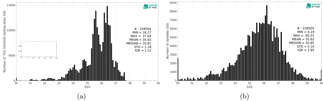
Figure 2: Histograms of SSS from TSG (GOSUD-Sailing-ship) (a) and SMOS SSS L2Q v331 - No FLAG (CMEMS-CATDS-CPDC) (b) considering all match-up pairs per bins of 0.1 over the Atlantic Ocean Pi-MEP region and for the full satellite product period.
