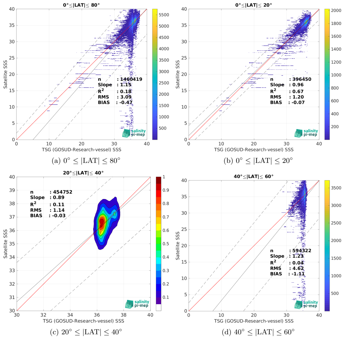
Figure 10: Contour maps of the concentration of SMOS SSS L2Q v331 - No FLAG (CMEMS-CATDS-CPDC) SSS (y-axis) versus TSG (GOSUD-Research-vessel) SSS (x-axis) at match-up pairs for different latitude bands. For each plot, the red line shows x=y . The black thin and dashed lines indicate a linear fit through the data cloud and the \pm 95\% confidence levels, respectively. The number match-up pairs n , the slope and R^2 coefficient of the linear fit, the root mean square (RMS) and the mean bias between satellite and in situ data are indicated for each latitude band in each plots.
