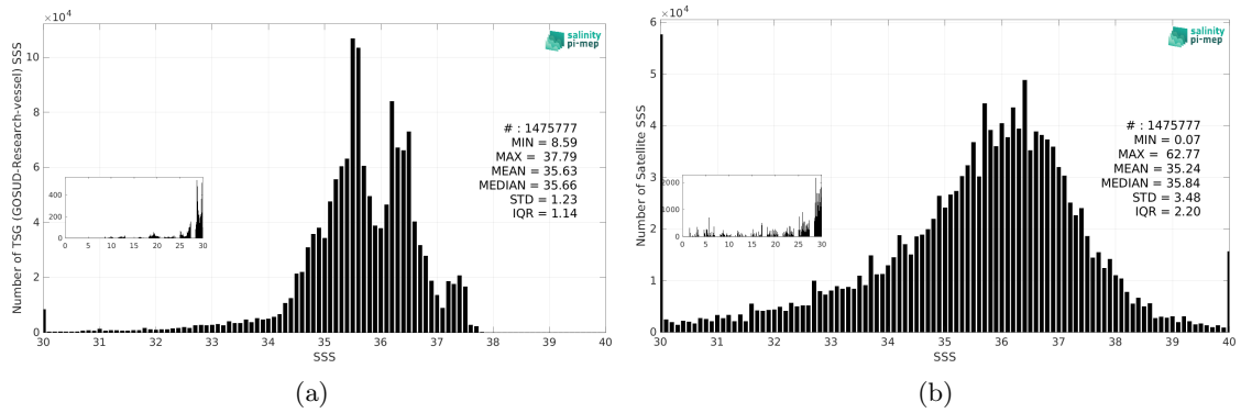
Figure 3: Histograms of SSS from TSG (GOSUD-Research-vessel) (a) and SMOS SSS L2Q v331 - No FLAG (CMEMS-CATDS-CPDC) (b) considering all match-up pairs per bins of 0.1 over the Atlantic Ocean Pi-MEP region and for the full satellite product period.
