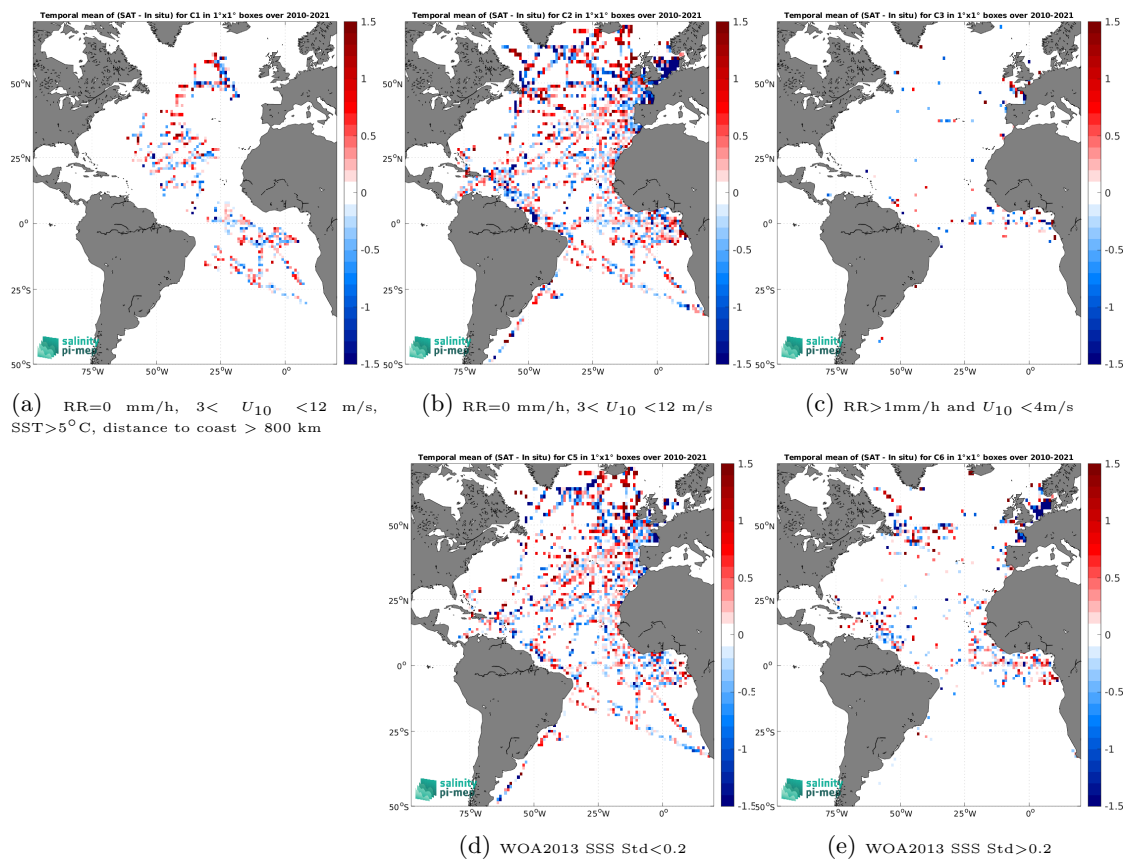
Figure 14: Temporal mean gridded over spatial boxes of size 1^\circ \times 1^\circ of \Delta SSS (SMOS SSS L2Q v331 - No FLAG (CMEMS-CATDS-CPDC) - TSG (GOSUD-Research-vessel)) for 5 different subdatasets corresponding to:RR=0 mm/h, 3 < U_{10} < 12 m/s, SST >5^\circ\text{C} , distance to coast > 800 km (a), RR=0 mm/h, 3 < U_{10} < 12 m/s (b), RR >1 mm/h and U_{10} < 4 m/s (c), WOA2013 SSS Std <0.2 (d), WOA2013 SSS Std >0.2 (e).
