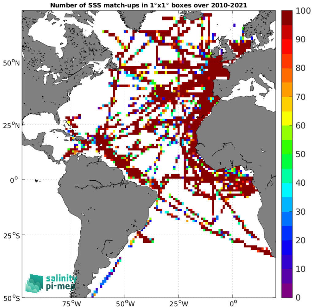
Figure 5: Number of SSS match-ups between TSG (GOSUD-Research-vessel) SSS and the SMOS SSS L2Q v331 - No FLAG (CMEMS-CATDS-CPDC) SSS product for the Atlantic Ocean Pi-MEP region over 1^\circ \times 1^\circ boxes and for the full satellite product period.
