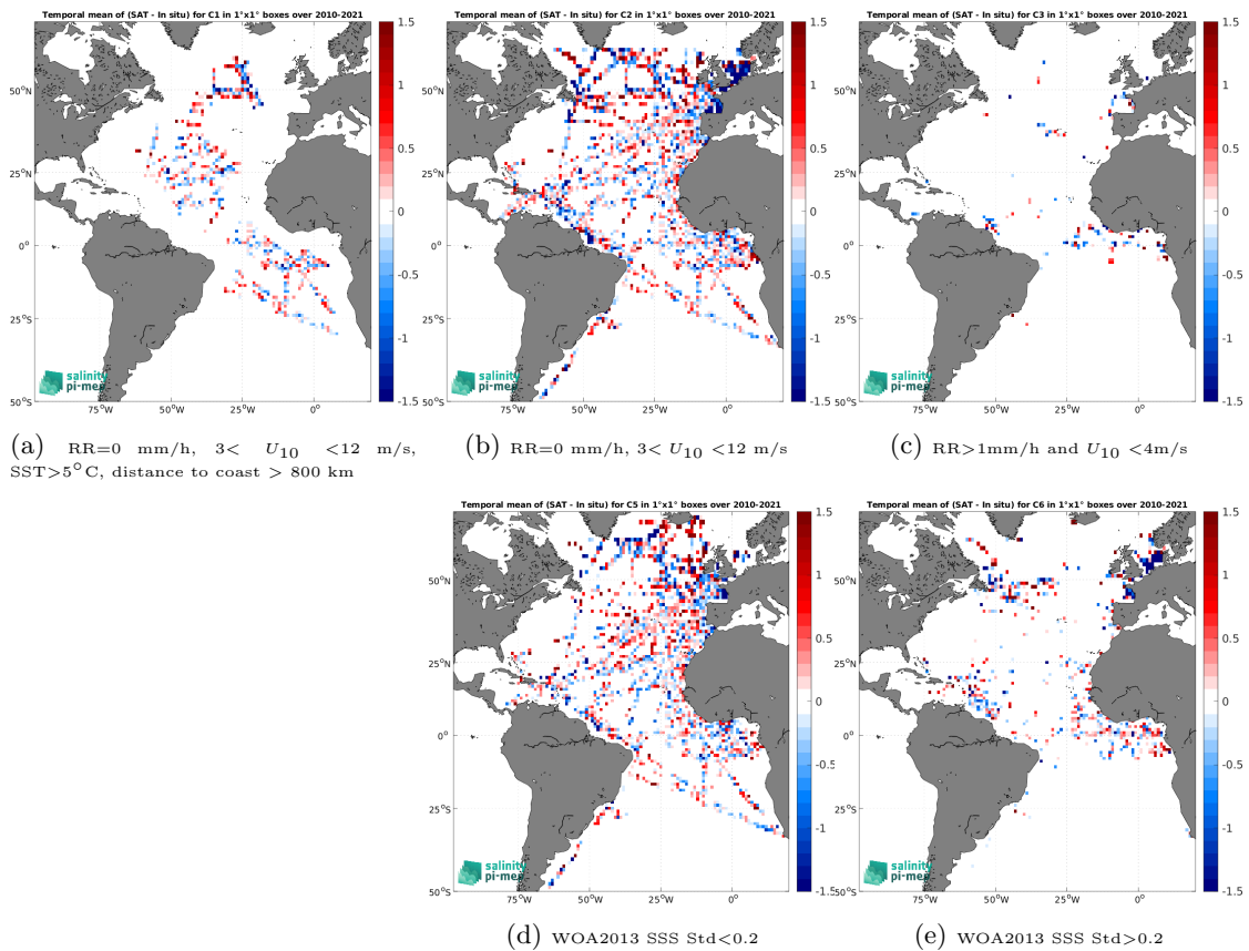
Figure 12: Temporal mean gridded over spatial boxes of size 1^\circ \times 1^\circ of \Delta\text{SSS} (SMOS SSS L2Q v331 - No FLAG (CMEMS-CATDS-CPDC) - TSG (GOSUD-Research-vessel)) for 5 different subdatasets corresponding to:RR=0 mm/h, 3 < U_{10} < 12 m/s, SST >5^\circ\text{C} , distance to coast > 800 km (a), RR=0 mm/h, 3 < U_{10} < 12 m/s (b), RR >1 mm/h and U_{10} < 4 m/s (c), WOA2013 SSS Std <0.2 (d), WOA2013 SSS Std >0.2 (e).
