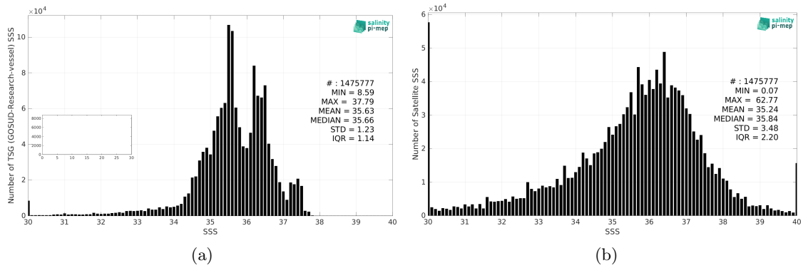
Figure 2: Histograms of SSS from TSG (GOSUD-Research-vessel) (a) and SMOS SSS L2Q v331 - No FLAG (CMEMS-CATDS-CPDC) (b) considering all match-up pairs per bins of 0.1 over the Atlantic Ocean Pi-MEP region and for the full satellite product period.
