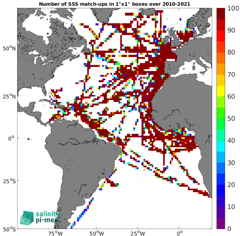
Figure 4: Number of SSS match-ups between TSG (GOSUD-Research-vessel) SSS and the SMOS SSS L2Q v331 - No FLAG (CMEMS-CATDS-CPDC) SSS product for the Atlantic Ocean Pi-MEP region over 1^\circ \times 1^\circ boxes and for the full satellite product period.
