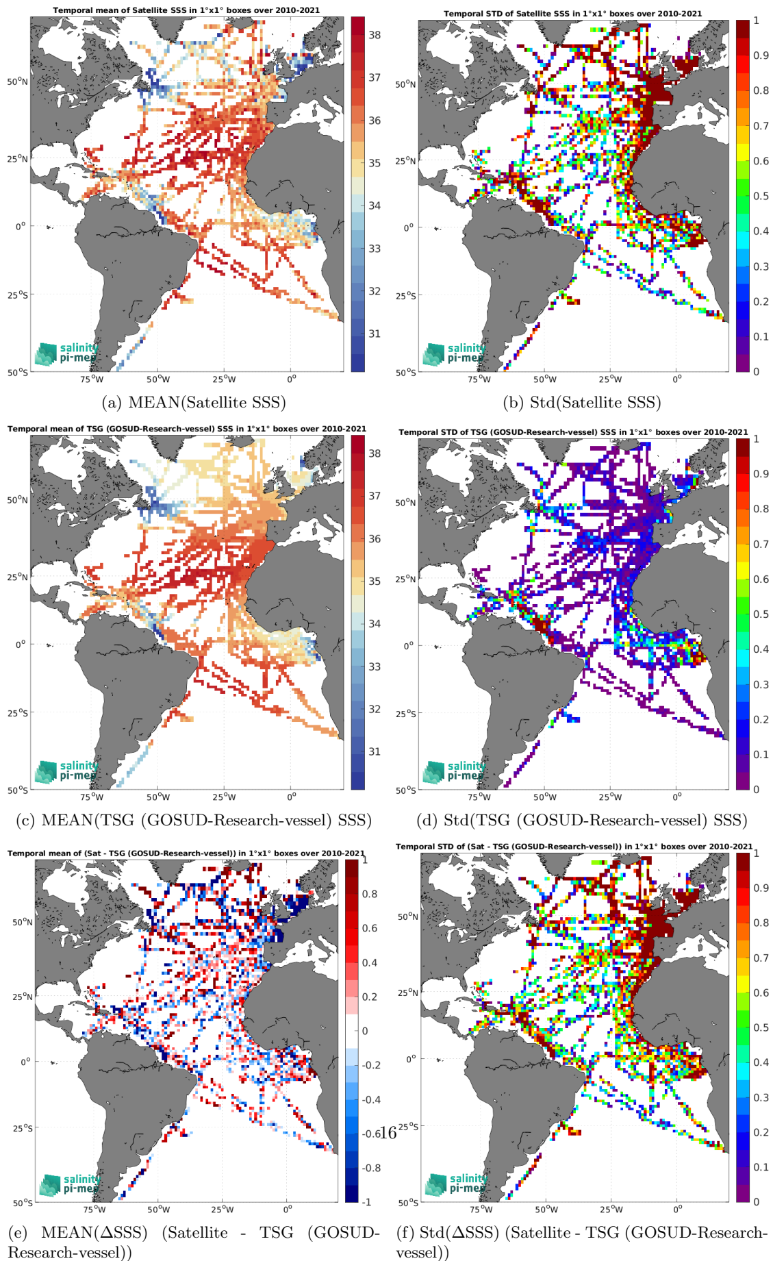
Figure 6: Temporal mean (left) and Std (right) of SSS from SMOS SSS L2Q v331 - No FLAG (CMEMS-CATDS-CPDC) (top), TSG (GOSUD-Research-vessel) (middle), and of \Delta SSS (Satellite - TSG (GOSUD-Research-vessel)). Only match-up pairs are used to generate these maps.
