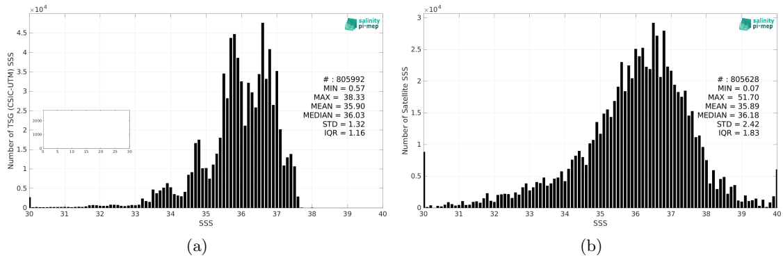
Figure 2: Histograms of SSS from TSG (CSIC-UTM) (a) and SMOS SSS L2Q v331 - No FLAG (CMEMS-CATDS-CPDC) (b) considering all match-up pairs per bins of 0.1 over the Atlantic Ocean Pi-MEP region and for the full satellite product period.
