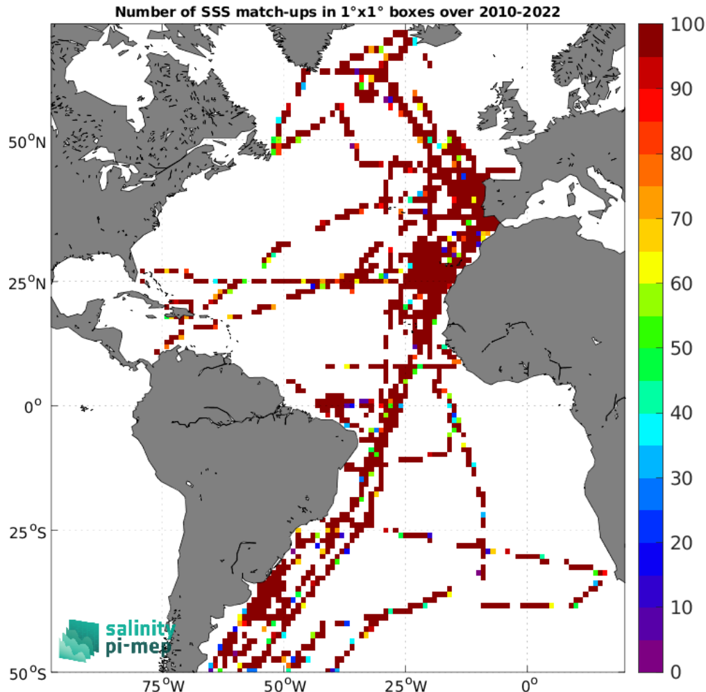
Figure 4: Number of SSS match-ups between TSG (CSIC-UTM) SSS and the SMOS SSS L2Q v331 - No FLAG (CMEMS-CATDS-CPDC) SSS product for the Atlantic Ocean Pi-MEP region over 1^\circ \times 1^\circ boxes and for the full satellite product period.
