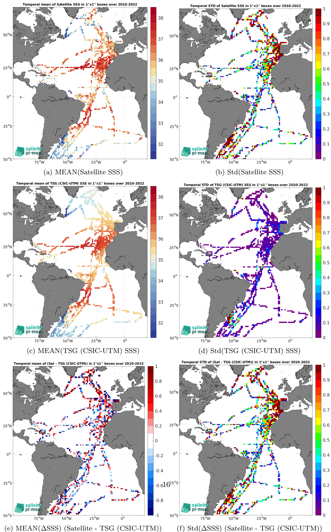
Figure 6: Temporal mean (left) and Std (right) of SSS from SMOS SSS L2Q v331 - No FLAG (CMEMS-CATDS-CPDC) (top), TSG (CSIC-UTM) (middle), and of \Delta SSS (Satellite - TSG (CSIC-UTM)). Only match-up pairs are used to generate these maps.
