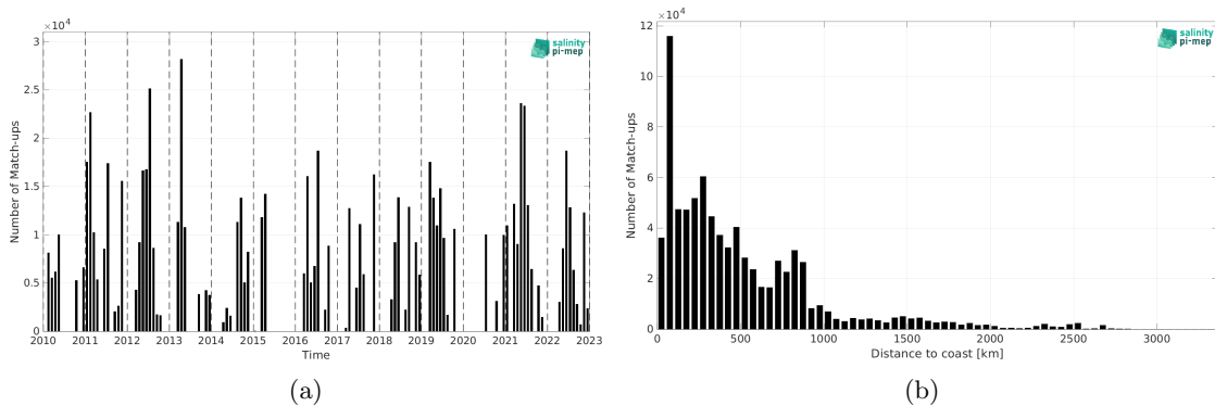
Figure 1: Number of match-ups between TSG (CSIC-UTM) and SMOS SSS L2Q v331 - No FLAG (CMEMS-CATDS-CPDC) SSS as a function of time (a) and as function of the distance to coast (b) over the Atlantic Ocean Pi-MEP region and for the full satellite product period.
