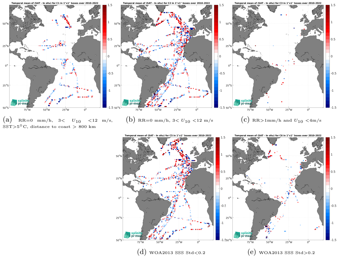
Figure 12: Temporal mean gridded over spatial boxes of size 1^\circ \times 1^\circ of \Delta SSS (SMOS SSS L2Q v331 - No FLAG (CMEMS-CATDS-CPDC) - TSG (CSIC-UTM)) for 5 different subdatasets corresponding to:RR=0 mm/h, 3 < U_{10} < 12 m/s, SST >5^\circ\text{C} , distance to coast > 800 km (a), RR=0 mm/h, 3 < U_{10} < 12 m/s (b), RR >1 mm/h and U_{10} < 4 m/s (c), WOA2013 SSS Std <0.2 (d), WOA2013 SSS Std >0.2 (e).
