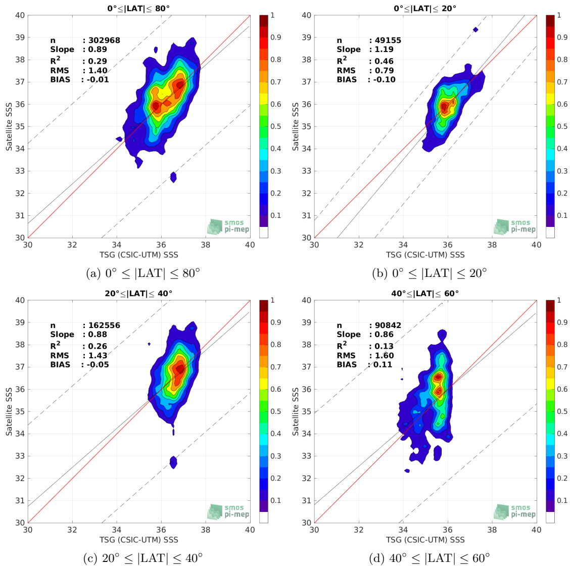
Figure 9: Contour maps of the concentration of SMOS SSS L2Q v331 - No FLAG (CMEMS-CATDS-CPDC) SSS ( y -axis) versus TSG (CSIC-UTM) SSS ( x -axis) at match-up pairs for different latitude bands. For each plot, the red line shows x=y . The black thin and dashed lines indicate a linear fit through the data cloud and the \pm 95\% confidence levels, respectively. The number match-up pairs n , the slope and R^2 coefficient of the linear fit, the root mean square (RMS) and the mean bias between satellite and in situ data are indicated for each latitude band in each plots.
