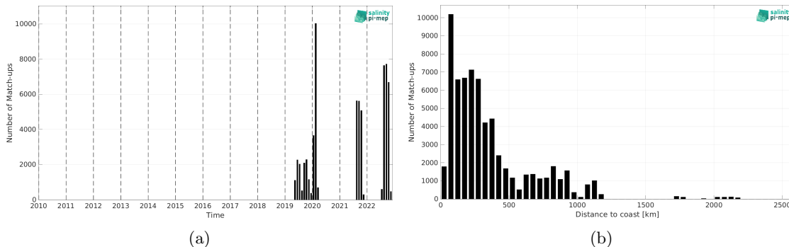
Figure 2: Number of match-ups between Saildrone and SMOS SSS L2Q v331 - No FLAG (CMEMS-CATDS-CPDC) SSS as a function of time (a) and as function of the distance to coast (b) over the Atlantic Ocean Pi-MEP region and for the full satellite product period.
