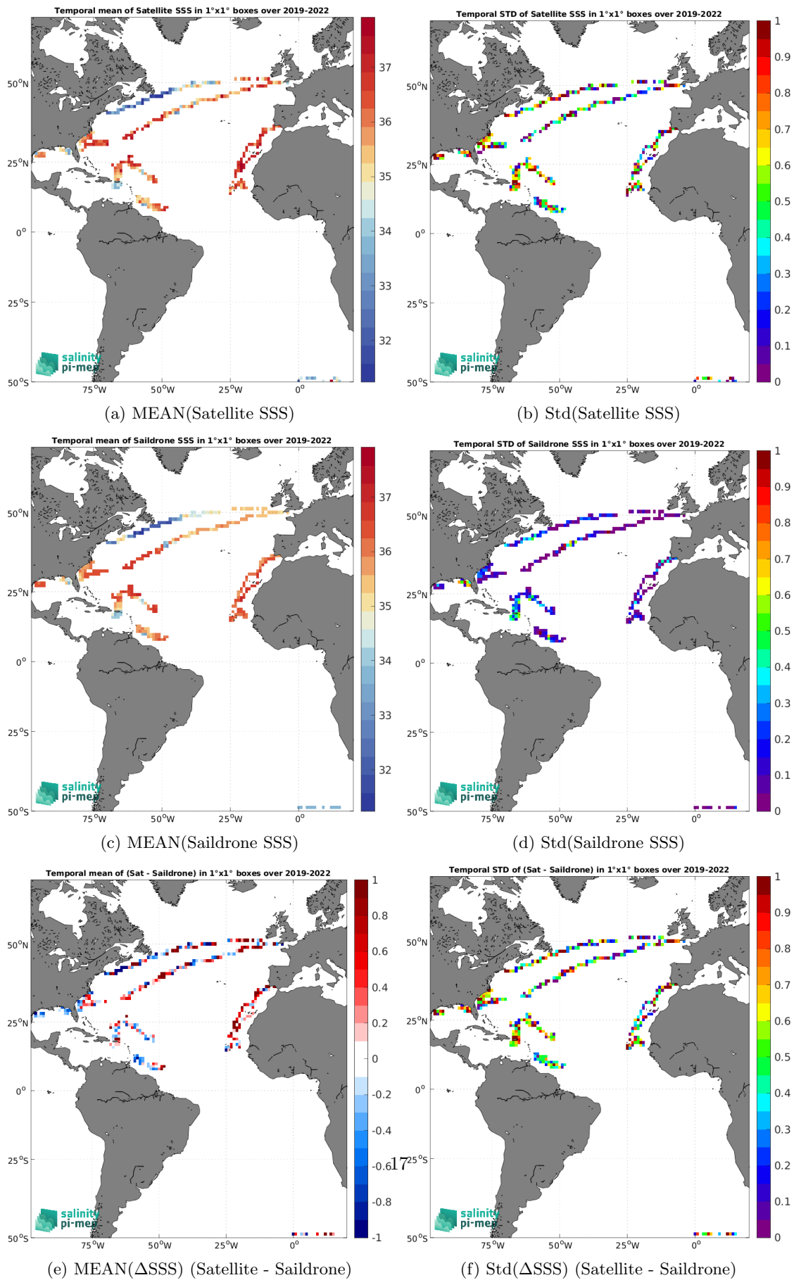
Figure 7: Temporal mean (left) and Std (right) of SSS from SMOS SSS L2Q v331 - No FLAG (CMEMS-CATDS-CPDC) (top), Saildrone (middle), and of \Delta\text{SSS} (Satellite - Saildrone). Only match-up pairs are used to generate these maps.
