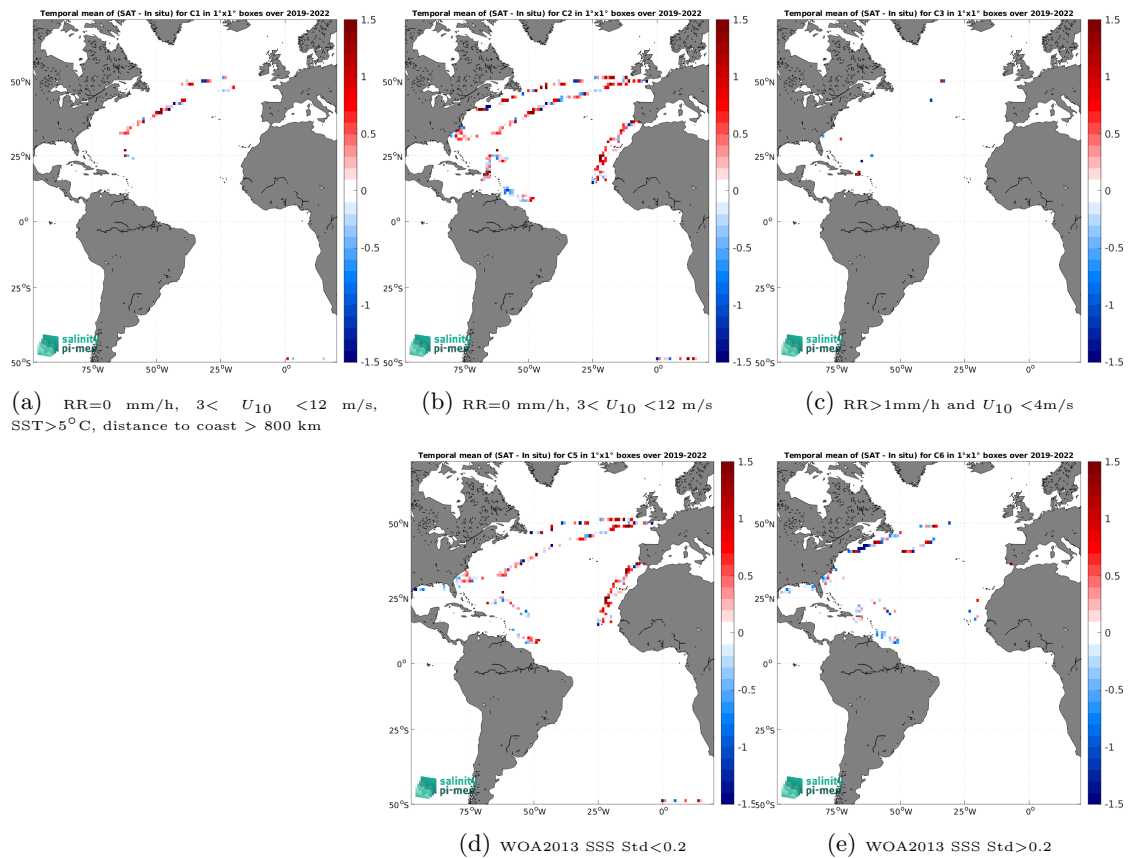
Figure 14: Temporal mean gridded over spatial boxes of size 1^\circ \times 1^\circ of \Delta SSS (SMOS SSS L2Q v331 - No FLAG (CMEMS-CATDS-CPDC) - Sailability) for 5 different subdatasets corresponding to:RR=0 mm/h, 3 < U_{10} < 12 m/s, SST >5^\circ\text{C} , distance to coast > 800 km (a), RR=0 mm/h, 3 < U_{10} < 12 m/s (b), RR >1 mm/h and U_{10} < 4 m/s (c), WOA2013 SSS Std <0.2 (d), WOA2013 SSS Std >0.2 (e).
