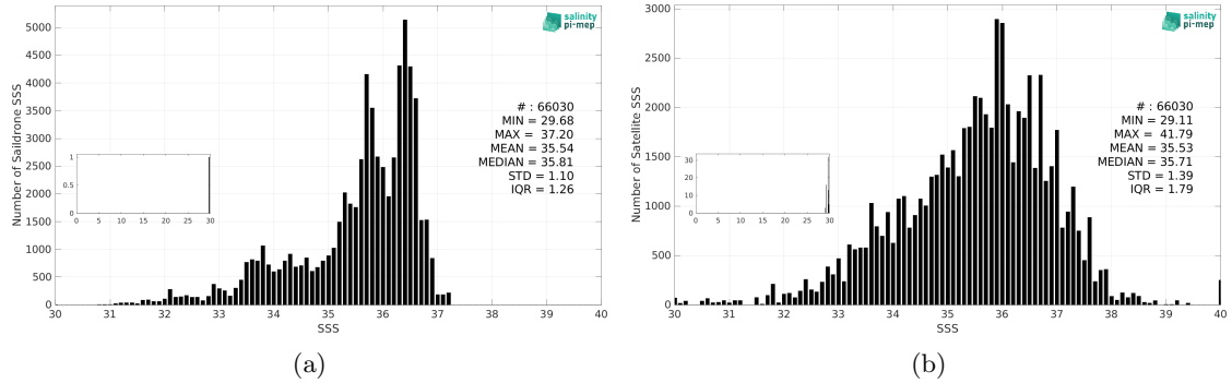
Figure 3: Histograms of SSS from Saildrone (a) and SMOS SSS L2Q v331 - No FLAG (CMEMS-CATDS-CPDC) (b) considering all match-up pairs per bins of 0.1 over the Atlantic Ocean Pi-MEP region and for the full satellite product period.
