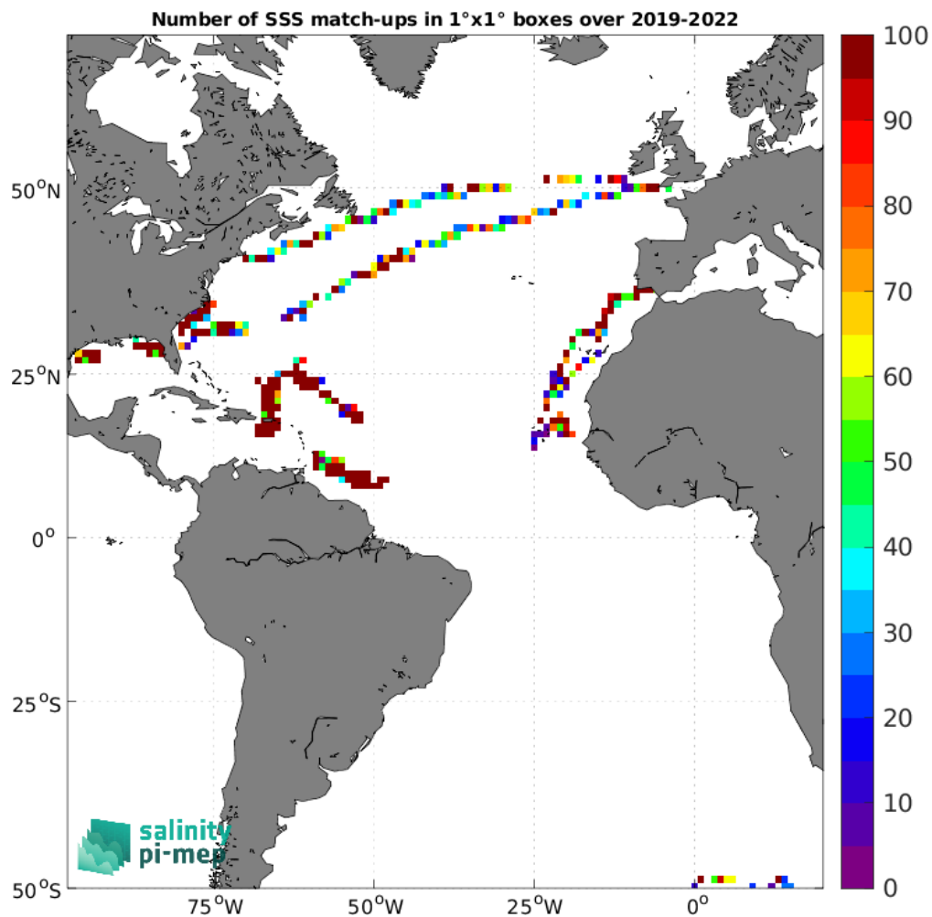
Figure 5: Number of SSS match-ups between Saildrone SSS and the SMOS SSS L2Q v331 - No FLAG (CMEMS-CATDS-CPDC) SSS product for the Atlantic Ocean Pi-MEP region over 1^\circ \times 1^\circ boxes and for the full satellite product period.
