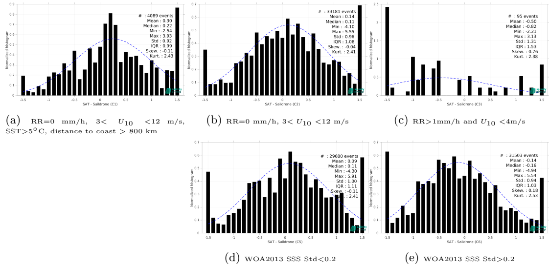
Figure 15: Normalized histogram of \Delta SSS (SMOS SSS L2Q v331 - No FLAG (CMEMS-CATDS-CPDC) - Salldrone) for 5 different subdatasets corresponding to: RR=0 mm/h, 3 < U_{10} < 12 m/s, SST > 5°C, distance to coast > 800 km (a), RR=0 mm/h, 3 < U_{10} < 12 m/s (b), RR > 1mm/h and U_{10} < 4 m/s (c), WOA2013 SSS Std < 0.2 (d), WOA2013 SSS Std > 0.2 (e).
