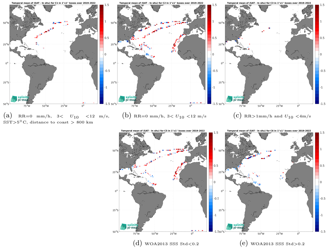
Figure 12: Temporal mean gridded over spatial boxes of size 1^\circ \times 1^\circ of \Delta\text{SSS} (SMOS SSS L2Q v331 - No FLAG (CMEMS-CATDS-CPDC) - Saildrone) for 5 different subdatasets corresponding to:RR=0 mm/h, 3 < U_{10} < 12 m/s, SST >5^\circ\text{C} , distance to coast > 800 km (a), RR=0 mm/h, 3 < U_{10} < 12 m/s (b), RR >1 mm/h and U_{10} < 4 m/s (c), WOA2013 SSS Std <0.2 (d), WOA2013 SSS Std >0.2 (e).
