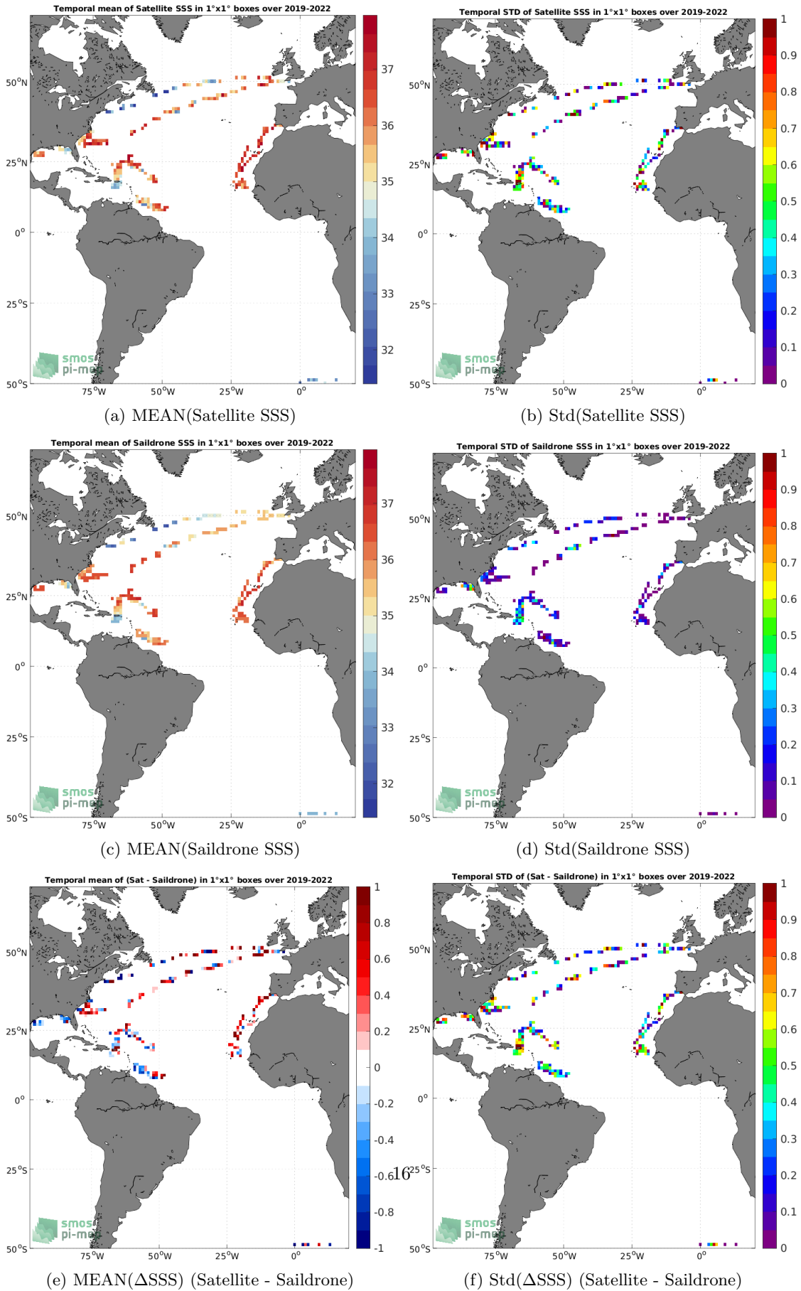
Figure 6: Temporal mean (left) and Std (right) of SSS from SMOS SSS L2Q v331 - No FLAG (CMEMS-CATDS-CPDC) (top), Saildrone (middle), and of \Delta SSS (Satellite - Saildrone). Only match-up pairs are used to generate these maps.
