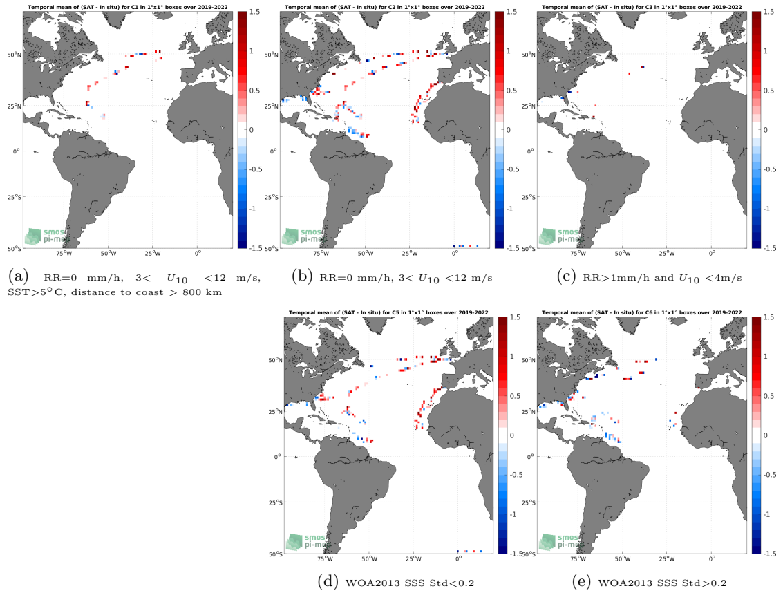
Figure 12: Temporal mean gridded over spatial boxes of size 1^\circ \times 1^\circ of \Delta SSS (SMOS SSS L2Q v331 - No FLAG (CMEMS-CATDS-CPDC) - Saildrone) for 5 different subdatasets corresponding to:RR=0 mm/h, 3 < U_{10} < 12 m/s, SST >5^\circ\text{C} , distance to coast > 800 km (a), RR=0 mm/h, 3 < U_{10} < 12 m/s (b), RR >1 mm/h and U_{10} < 4 m/s (c), WOA2013 SSS Std <0.2 (d), WOA2013 SSS Std >0.2 (e).
