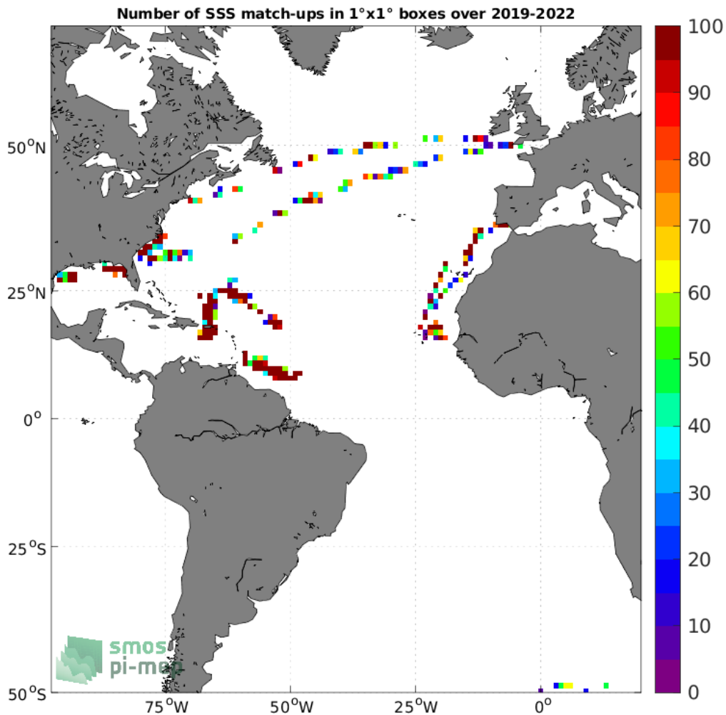
Figure 4: Number of SSS match-ups between Saildrone SSS and the SMOS SSS L2Q v331 - No FLAG (CMEMS-CATDS-CPDC) SSS product for the Atlantic Ocean Pi-MEP region over 1°×1° boxes and for the full satellite product period.
