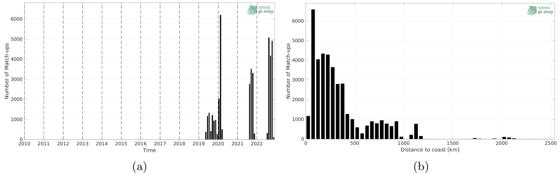
Figure 1: Number of match-ups between Saildrone and SMOS SSS L2Q v331 - No FLAG (CMEMS-CATDS-CPDC) SSS as a function of time (a) and as function of the distance to coast (b) over the Atlantic Ocean Pi-MEP region and for the full satellite product period.
