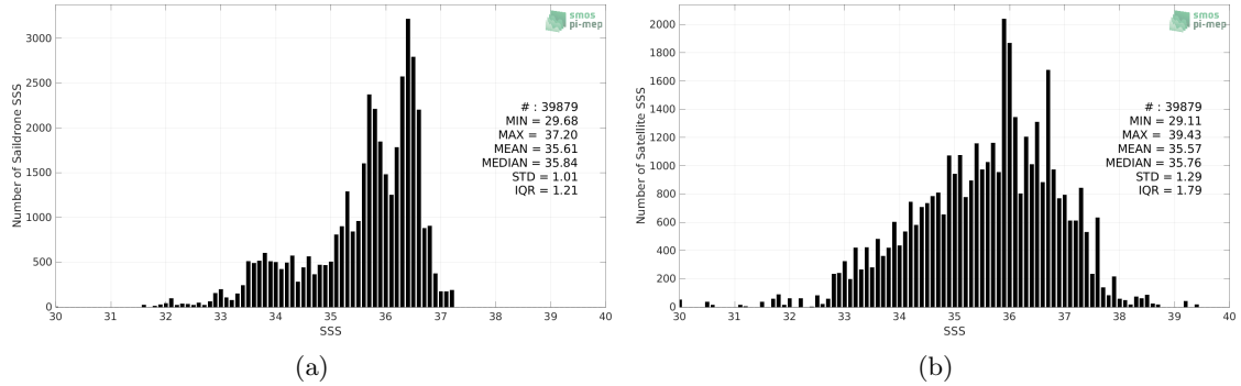
Figure 2: Histograms of SSS from Saildrone (a) and SMOS SSS L2Q v331 - No FLAG (CMEMS-CATDS-CPDC) (b) considering all match-up pairs per bins of 0.1 over the Atlantic Ocean Pi-MEP region and for the full satellite product period.
