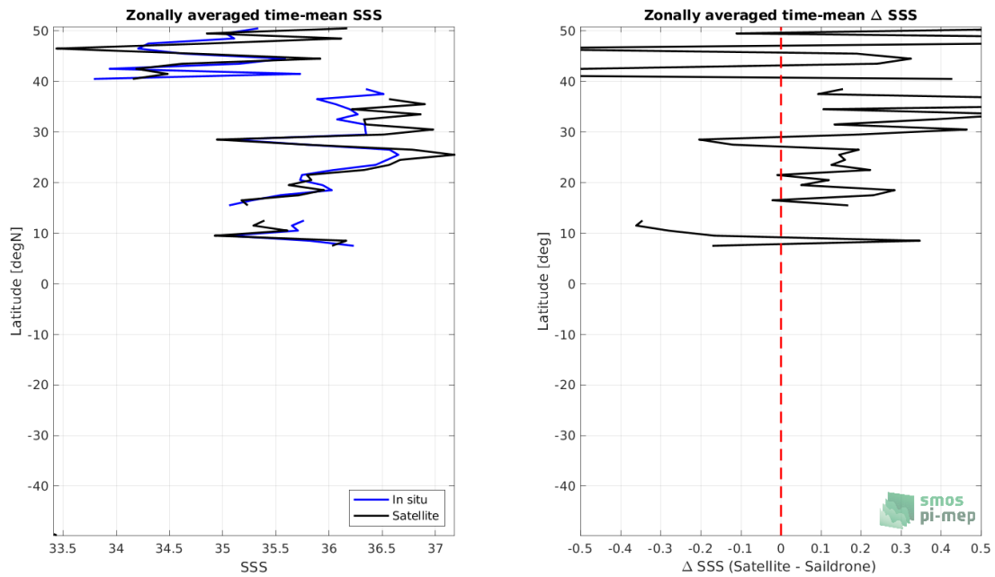
Figure 8: Left panel: Zonal mean SSS from SMOS SSS L2Q v331 - No FLAG (CMEMS-CATDS-CPDC) satellite product (black) and from Saiddrone (blue). Right panel: Zonal mean of \Delta SSS (Satellite - Saiddrone) for all the collected Pi-MEP match-up pairs estimated over the full satellite product period.
