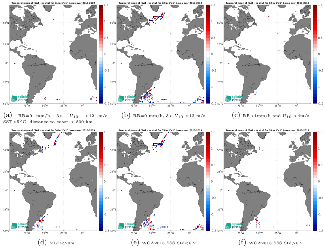
Figure 12: Temporal mean gridded over spatial boxes of size 1^{\circ} \times 1^{\circ} of \Delta SSS (SMOS SSS L2Q v331 - No FLAG (CMEMS-CATDS-CPDC) - Marine mammals) for 6 different subdatasets corresponding to: RR=0 mm/h, 3 < U_{10} < 12 m/s, SST > 5^{\circ}C , distance to coast > 800 km (a), RR=0 mm/h, 3 < U_{10} < 12 m/s (b), RR > 1 mm/h and U_{10} < 4 m/s (c), MLD < 20 m (d), WOA2013 SSS Std < 0.2 (e), WOA2013 SSS Std > 0.2 (f).
