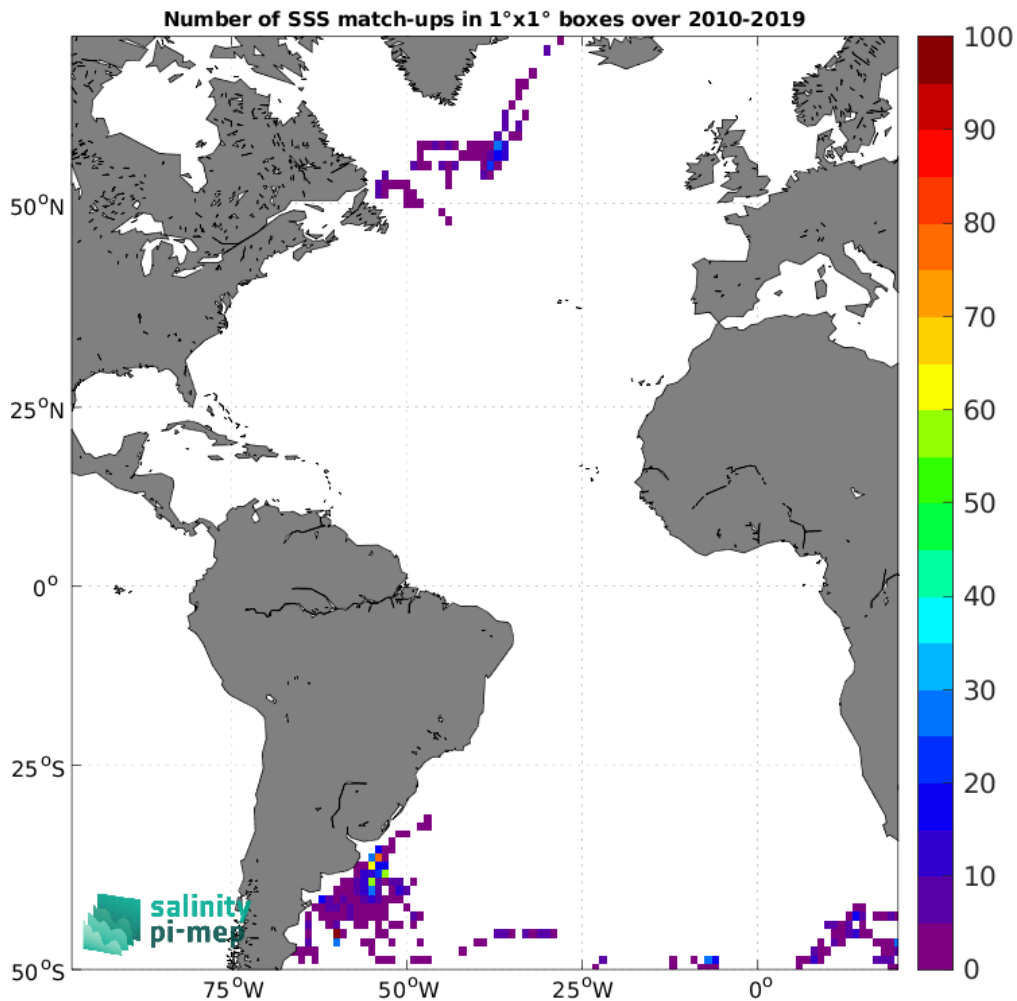
Figure 4: Number of SSS match-ups between Marine mammals SSS and the SMOS SSS L2Q v331 - No FLAG (CMEMS-CATDS-CPDC) SSS product for the Atlantic Ocean Pi-MEP region over 1°x1° boxes and for the full satellite product period.
