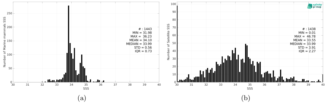
Figure 2: Histograms of SSS from Marine mammals (a) and SMOS SSS L2Q v331 - No FLAG (CMEMS-CATDS-CPDC) (b) considering all match-up pairs per bins of 0.1 over the Atlantic Ocean Pi-MEP region and for the full satellite product period.
