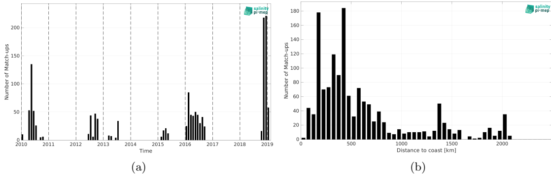
Figure 1: Number of match-ups between Marine mammals and SMOS SSS L2Q v331 - No FLAG (CMEMS-CATDS-CPDC) SSS as a function of time (a) and as function of the distance to coast (b) over the Atlantic Ocean Pi-MEP region and for the full satellite product period.
