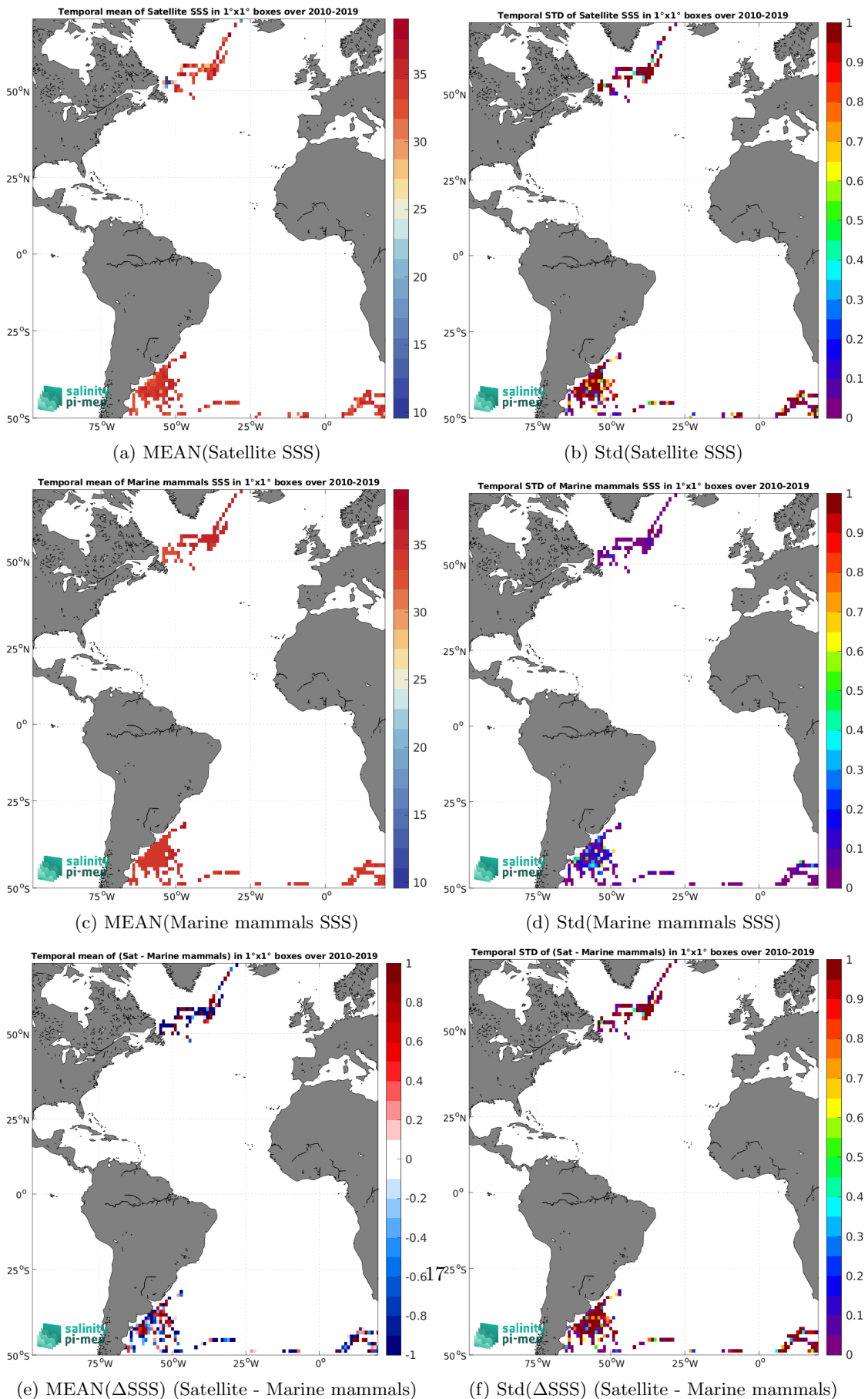
Figure 6: Temporal mean (left) and Std (right) of SSS from SMOS SSS L2Q v331 - No FLAG (CMEMS-CATDS-CPDC) (top), Marine mammals (middle), and of \Delta SSS (Satellite - Marine mammals). Only match-up pairs are used to generate these maps.
