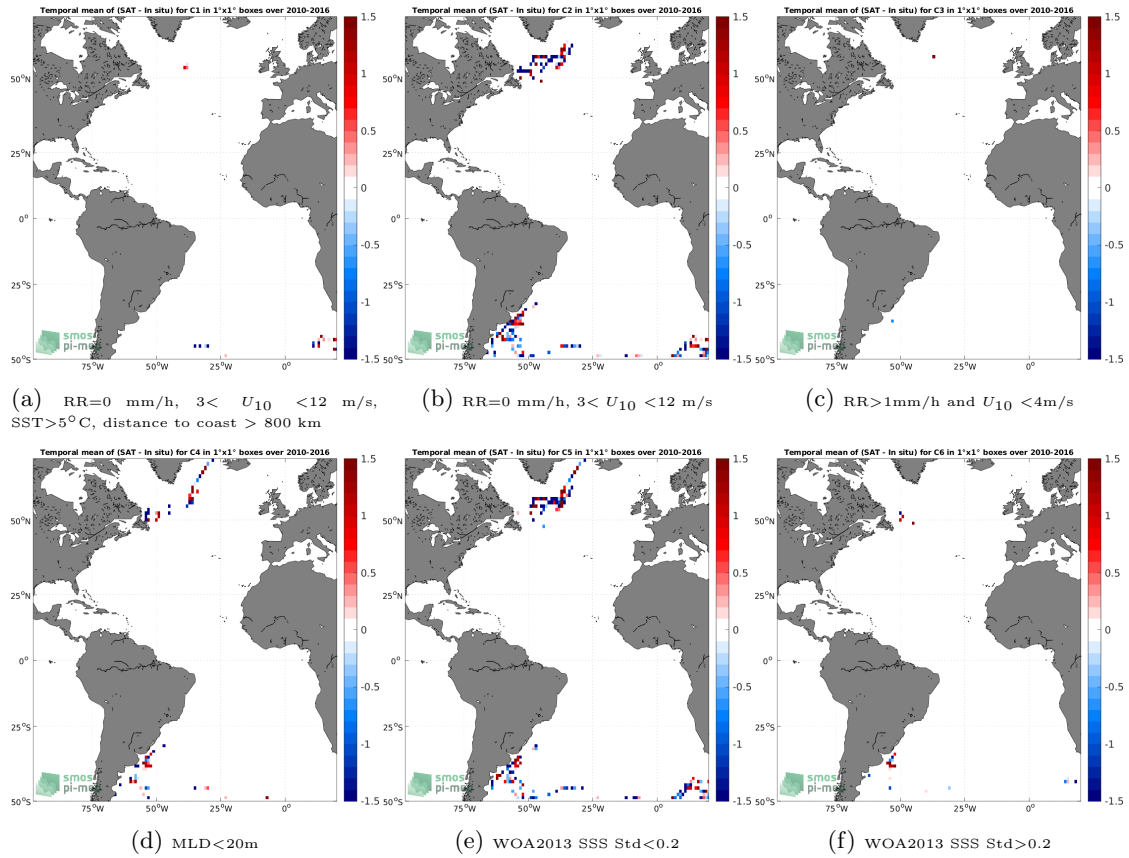
Figure 12: Temporal mean gridded over spatial boxes of size 1^\circ \times 1^\circ of \Delta SSS (SMOS SSS L2Q v331 - No FLAG (CMEMS-CATDS-CPDC) - Marine mammals) for 6 different subdatasets corresponding to: RR=0 mm/h, 3 < U_{10} < 12 m/s, SST > 5°C, distance to coast > 800 km (a), RR=0 mm/h, 3 < U_{10} < 12 m/s (b), RR > 1mm/h and U_{10} < 4 m/s (c), MLD < 20m (d), WOA2013 SSS Std < 0.2 (e), WOA2013 SSS Std > 0.2 (f).
