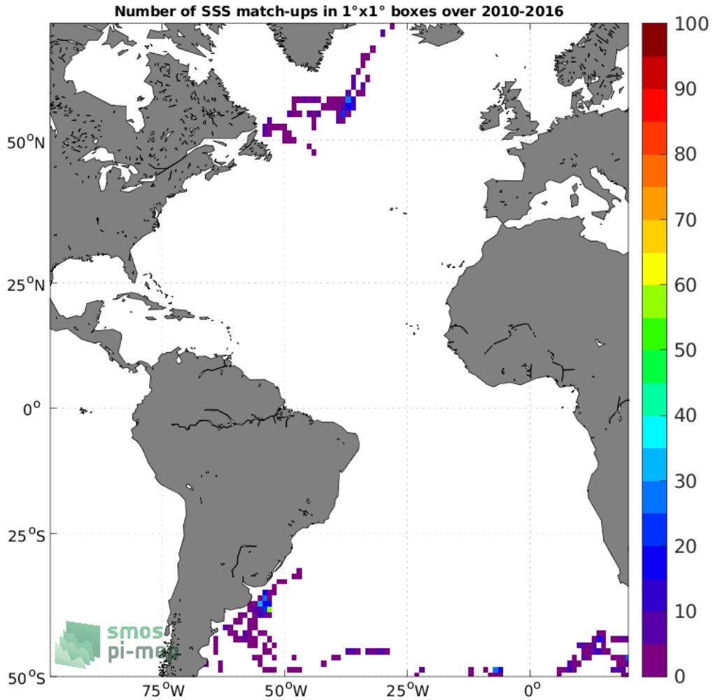
Figure 4: Number of SSS match-ups between Marine mammals SSS and the SMOS SSS L2Q v331 - No FLAG (CMEMS-CATDS-CPDC) SSS product for the Atlantic Ocean Pi-MEP region over 1^\circ \times 1^\circ boxes and for the full satellite product period.
