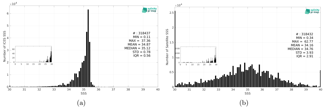
Figure 3: Histograms of SSS from ICES (a) and SMOS SSS L2Q v331 - No FLAG (CMEMS-CATDS-CPDC) (b) considering all match-up pairs per bins of 0.1 over the Atlantic Ocean Pi-MEP region and for the full satellite product period.
