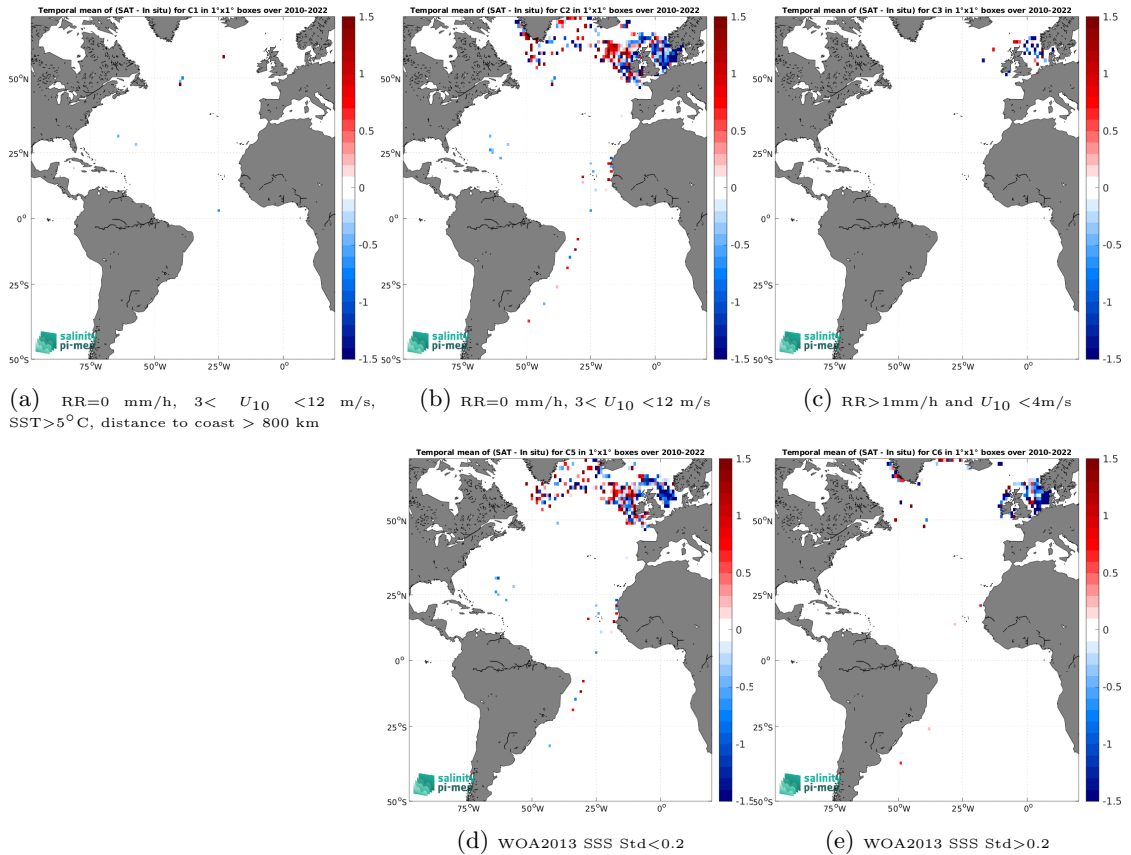
Figure 14: Temporal mean gridded over spatial boxes of size 1^\circ \times 1^\circ of \Delta\text{SSS} (SMOS SSS L2Q v331 - No FLAG (CMEMS-CATDS-CPDC) - ICES) for 5 different subdatasets corresponding to:RR=0 mm/h, 3 < U_{10} < 12 m/s, SST>5°C, distance to coast > 800 km (a), RR=0 mm/h, 3 < U_{10} < 12 m/s (b), RR>1mm/h and U_{10} < 4 m/s (c), WOA2013 SSS Std<0.2 (d), WOA2013 SSS Std>0.2 (e).
