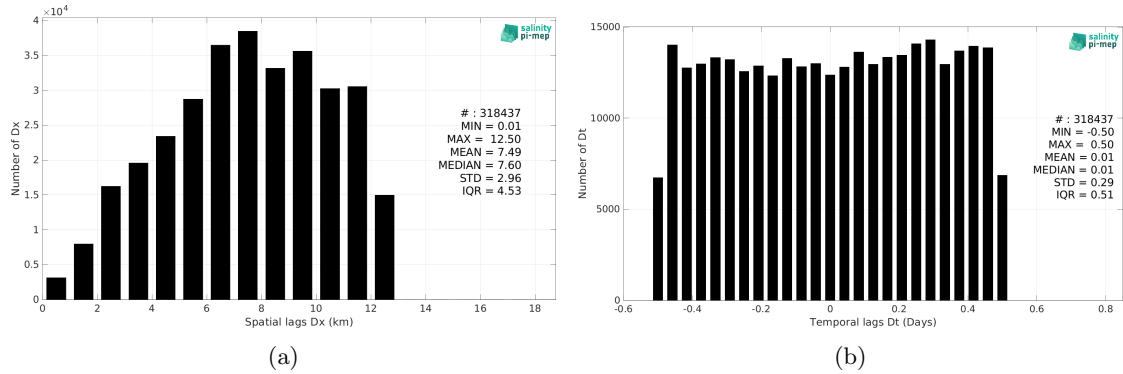
Figure 6: Histograms of the spatial (a) and temporal (b) lags between the location/time of the ICES measurement and the date of the corresponding SMOS SSS L2Q v331 - No FLAG (CMEMS-CATDS-CPDC) SSS pixel.
