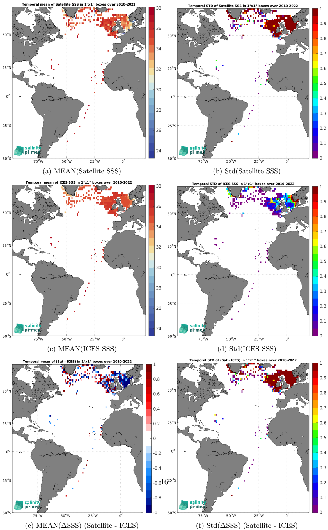
Figure 7: Temporal mean (left) and Std (right) of SSS from SMOS SSS L2Q v331 - No FLAG (CMEMS-CATDS-CPDC) (top), ICES (middle), and of \Delta SSS (Satellite - ICES). Only match-up pairs are used to generate these maps.
