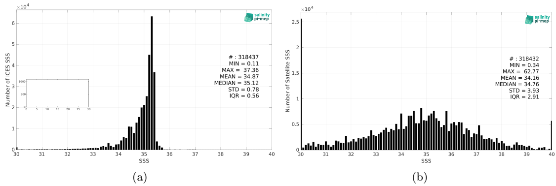
Figure 2: Histograms of SSS from ICES (a) and SMOS SSS L2Q v331 - No FLAG (CMEMS-CATDS-CPDC) (b) considering all match-up pairs per bins of 0.1 over the Atlantic Ocean Pi-MEP region and for the full satellite product period.
