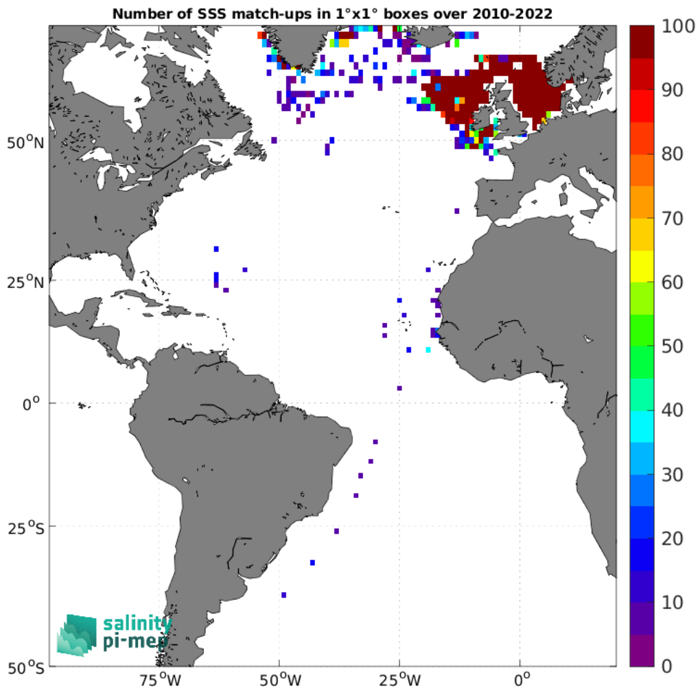
Figure 4: Number of SSS match-ups between ICES SSS and the SMOS SSS L2Q v331 - No FLAG (CMEMS-CATDS-CPDC) SSS product for the Atlantic Ocean Pi-MEP region over 1^\circ \times 1^\circ boxes and for the full satellite product period.
