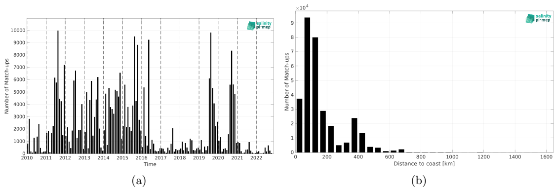
Figure 1: Number of match-ups between ICES and SMOS SSS L2Q v331 - No FLAG (CMEMS-CATDS-CPDC) SSS as a function of time (a) and as function of the distance to coast (b) over the Atlantic Ocean Pi-MEP region and for the full satellite product period.
