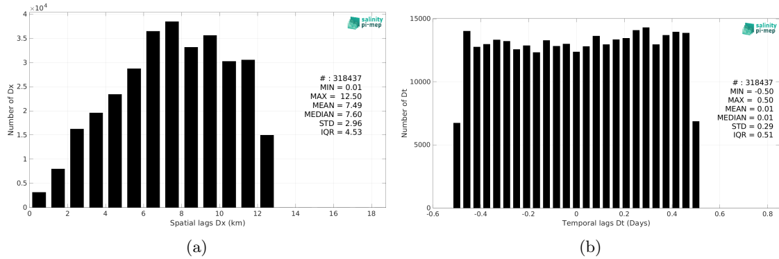
Figure 5: Histograms of the spatial (a) and temporal (b) lags between the location/time of the ICES measurement and the date of the corresponding SMOS SSS L2Q v331 - No FLAG (CMEMS-CATDS-CPDC) SSS pixel.
