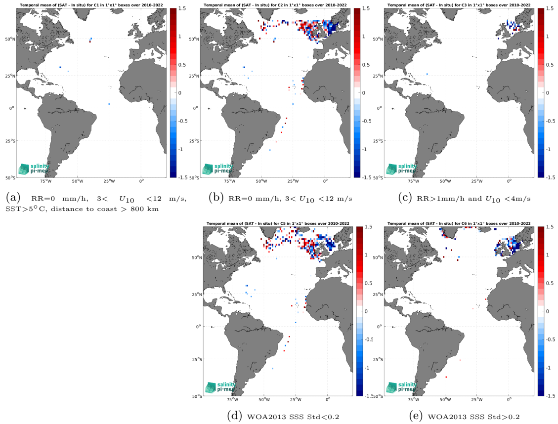
Figure 12: Temporal mean gridded over spatial boxes of size 1^\circ \times 1^\circ of \Delta\text{SSS} (SMOS SSS L2Q v331 - No FLAG (CMEMS-CATDS-CPDC) - ICES) for 5 different subdatasets corresponding to:RR=0 mm/h, 3 < U_{10} < 12 m/s, SST >5^\circ\text{C} , distance to coast > 800 km (a), RR=0 mm/h, 3 < U_{10} < 12 m/s (b), RR >1 mm/h and U_{10} < 4 m/s (c), WOA2013 SSS Std <0.2 (d), WOA2013 SSS Std >0.2 (e).
