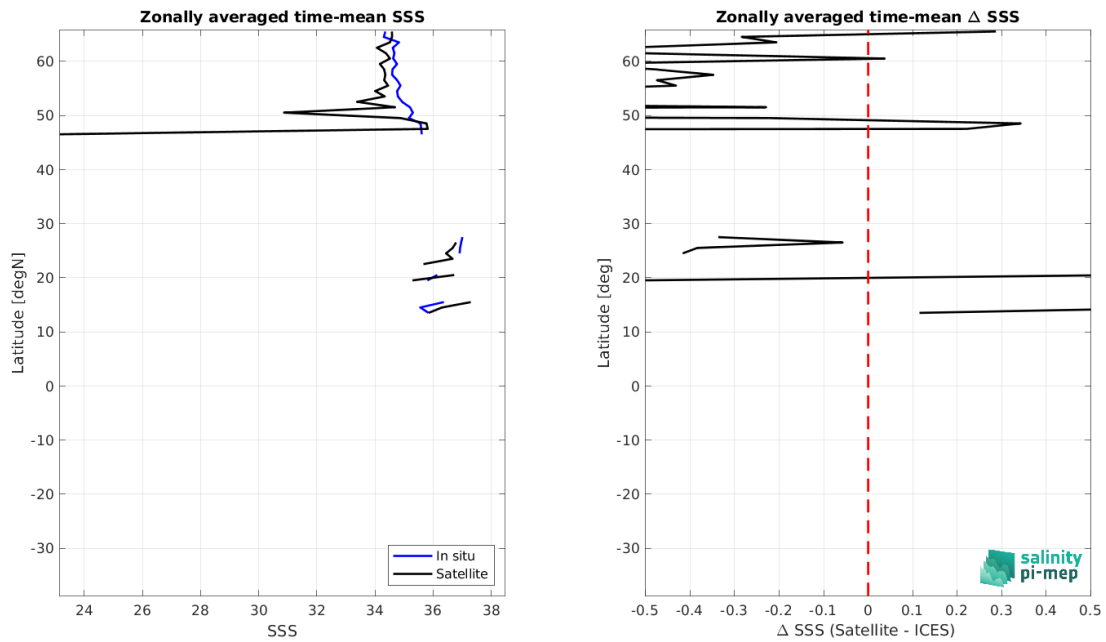
Figure 8: Left panel: Zonal mean SSS from SMOS SSS L2Q v331 - No FLAG (CMEMS-CATDS-CPDC) satellite product (black) and from ICES (blue). Right panel: Zonal mean of \Delta SSS (Satellite - ICES) for all the collected Pi-MEP match-up pairs estimated over the full satellite product period.
