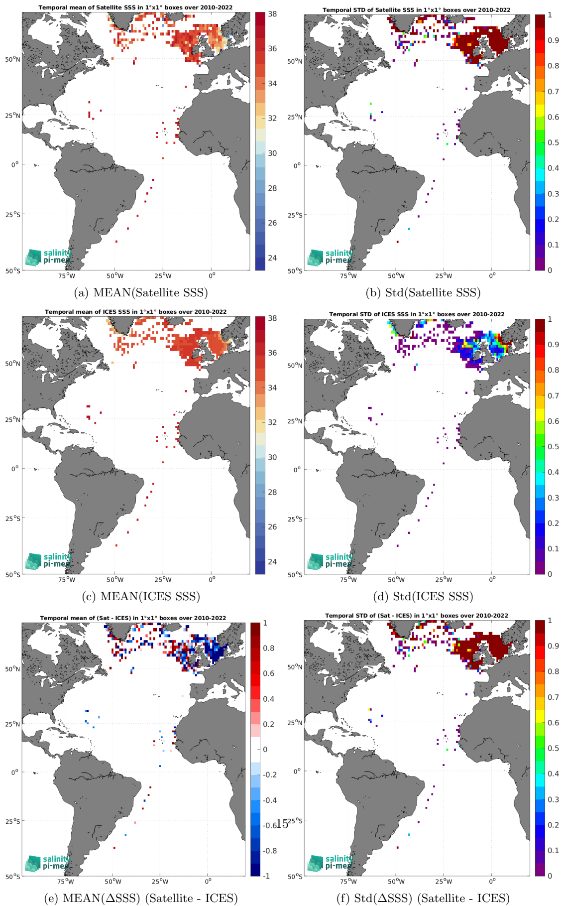
Figure 6: Temporal mean (left) and Std (right) of SSS from SMOS SSS L2Q v331 - No FLAG (CMEMS-CATDS-CPDC) (top), ICES (middle), and of \Delta SSS (Satellite - ICES). Only match-up pairs are used to generate these maps.
