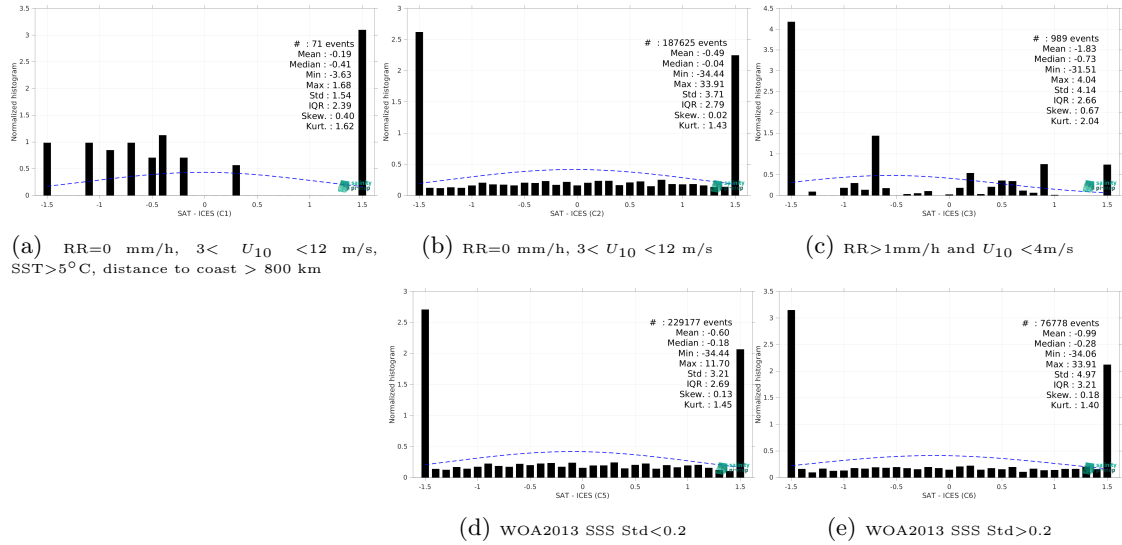
Figure 13: Normalized histogram of \Delta SSS (SMOS SSS L2Q v331 - No FLAG (CMEMS-CATDS-CPDC) - ICES) for 5 different subdatasets corresponding to: RR=0 mm/h, 3 < U_{10} < 12 m/s, SST > 5°C, distance to coast > 800 km (a), RR=0 mm/h, 3 < U_{10} < 12 m/s (b), RR > 1mm/h and U_{10} < 4 m/s (c), WOA2013 SSS Std < 0.2 (d), WOA2013 SSS Std > 0.2 (e).
