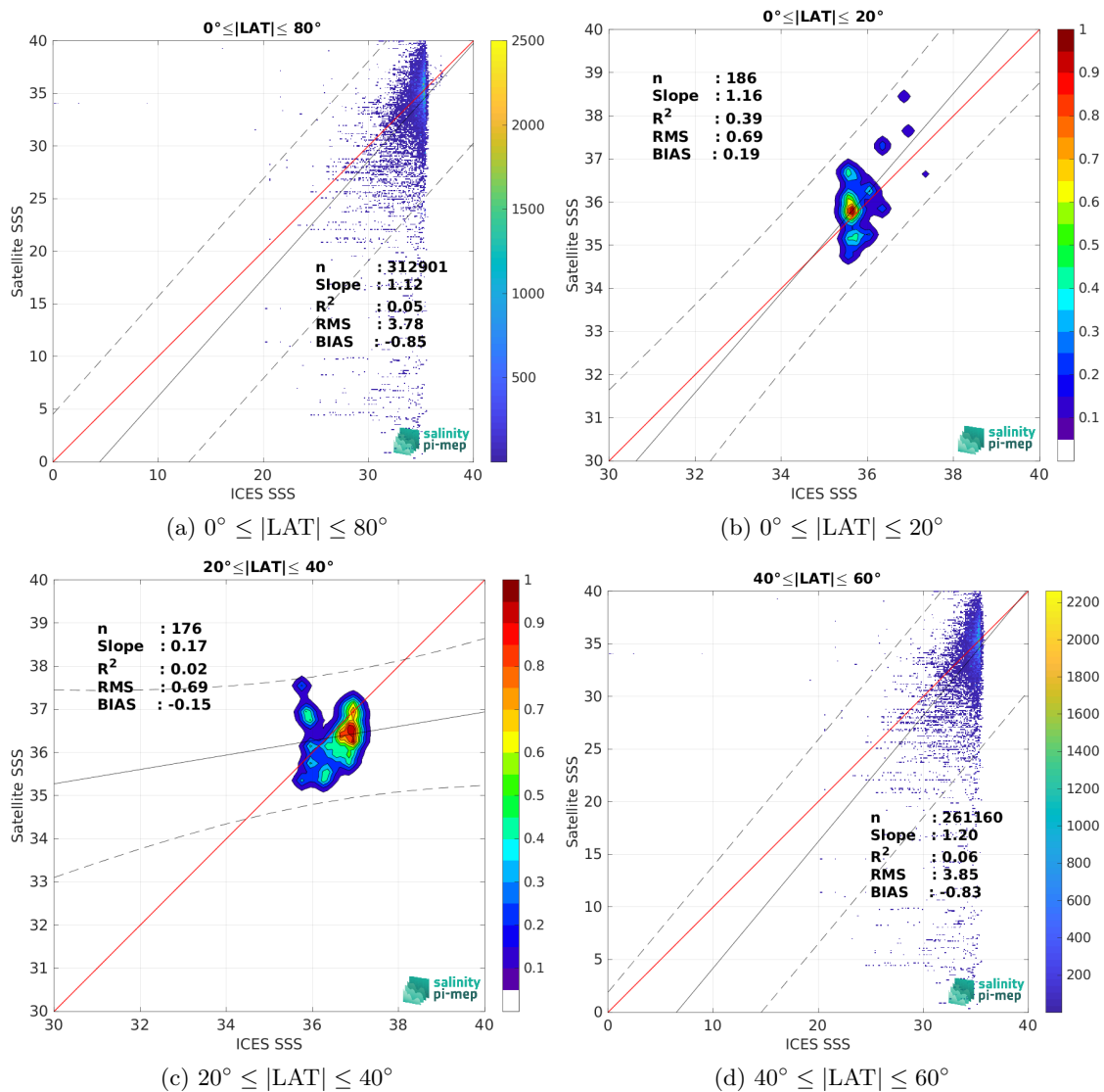
Figure 9: Contour maps of the concentration of SMOS SSS L2Q v331 - No FLAG (CMEMS-CATDS-CPDC) SSS (y-axis) versus ICES SSS (x-axis) at match-up pairs for different latitude bands. For each plot, the red line shows x=y . The black thin and dashed lines indicate a linear fit through the data cloud and the \pm 95\% confidence levels, respectively. The number match-up pairs n , the slope and R^2 coefficient of the linear fit, the root mean square (RMS) and the mean bias between satellite and in situ data are indicated for each latitude band in each plots.
