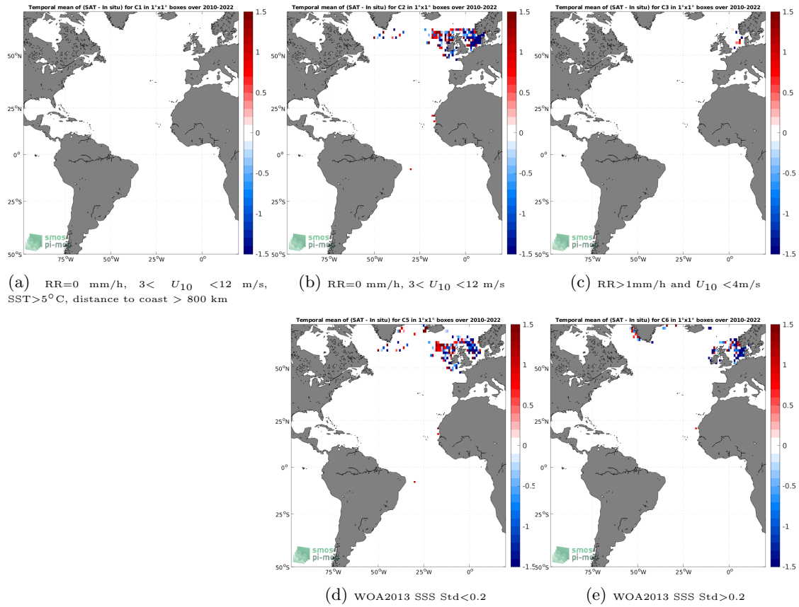
Figure 12: Temporal mean gridded over spatial boxes of size 1^\circ \times 1^\circ of \Delta SSS (SMOS SSS L2Q v331 - No FLAG (CMEMS-CATDS-CPDC) - ICES) for 5 different subdatasets corresponding to:RR=0 mm/h, 3 < U_{10} < 12 m/s, SST >5^\circ\text{C} , distance to coast > 800 km (a), RR=0 mm/h, 3 < U_{10} < 12 m/s (b), RR >1 mm/h and U_{10} < 4 m/s (c), WOA2013 SSS Std <0.2 (d), WOA2013 SSS Std >0.2 (e).
