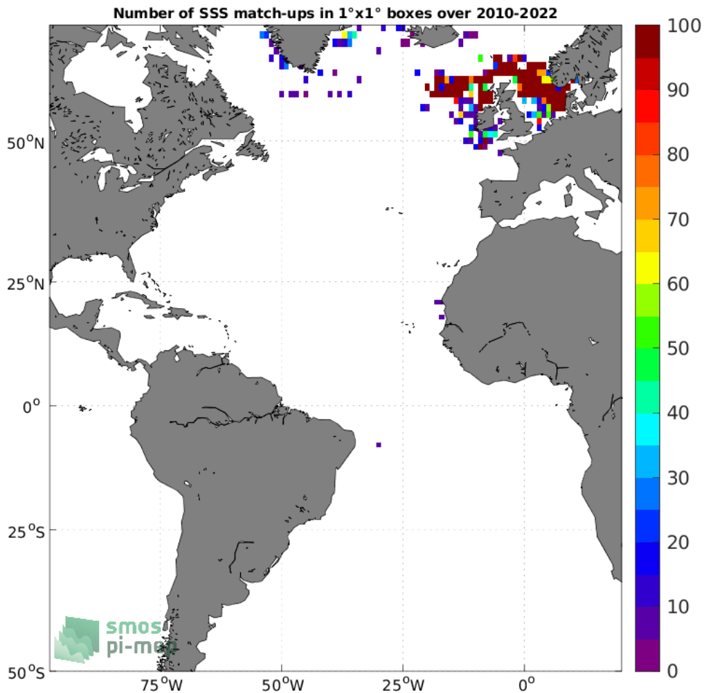
Figure 4: Number of SSS match-ups between ICES SSS and the SMOS SSS L2Q v331 - No FLAG (CMEMS-CATDS-CPDC) SSS product for the Atlantic Ocean Pi-MEP region over 1°x1° boxes and for the full satellite product period.
