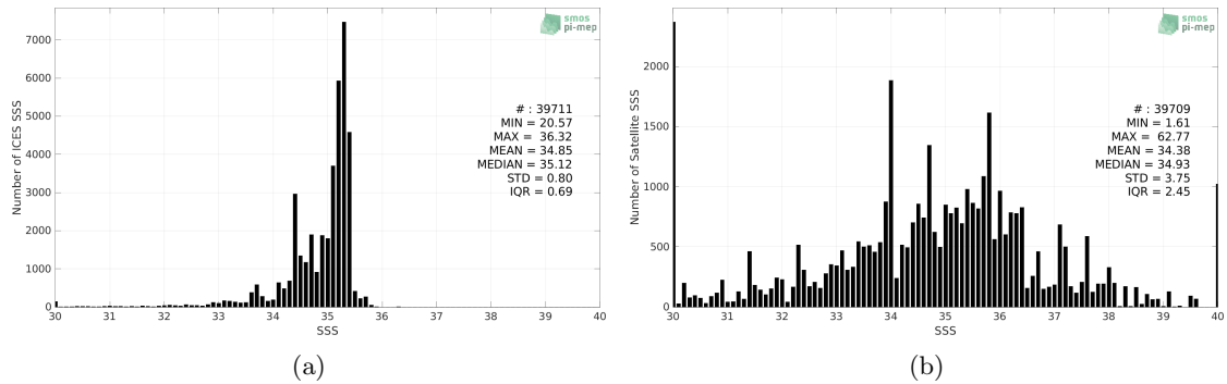
Figure 2: Histograms of SSS from ICES (a) and SMOS SSS L2Q v331 - No FLAG (CMEMS-CATDS-CPDC) (b) considering all match-up pairs per bins of 0.1 over the Atlantic Ocean Pi-MEP region and for the full satellite product period.
