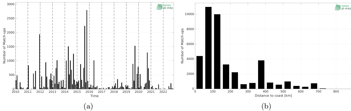
Figure 1: Number of match-ups between ICES and SMOS SSS L2Q v331 - No FLAG (CMEMS-CATDS-CPDC) SSS as a function of time (a) and as function of the distance to coast (b) over the Atlantic Ocean Pi-MEP region and for the full satellite product period.
