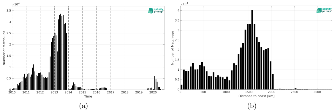
Figure 2: Number of match-ups between Surface drifters and SMOS SSS L2Q v331 - No FLAG (CMEMS-CATDS-CPDC) SSS as a function of time (a) and as function of the distance to coast (b) over the Atlantic Ocean Pi-MEP region and for the full satellite product period.
