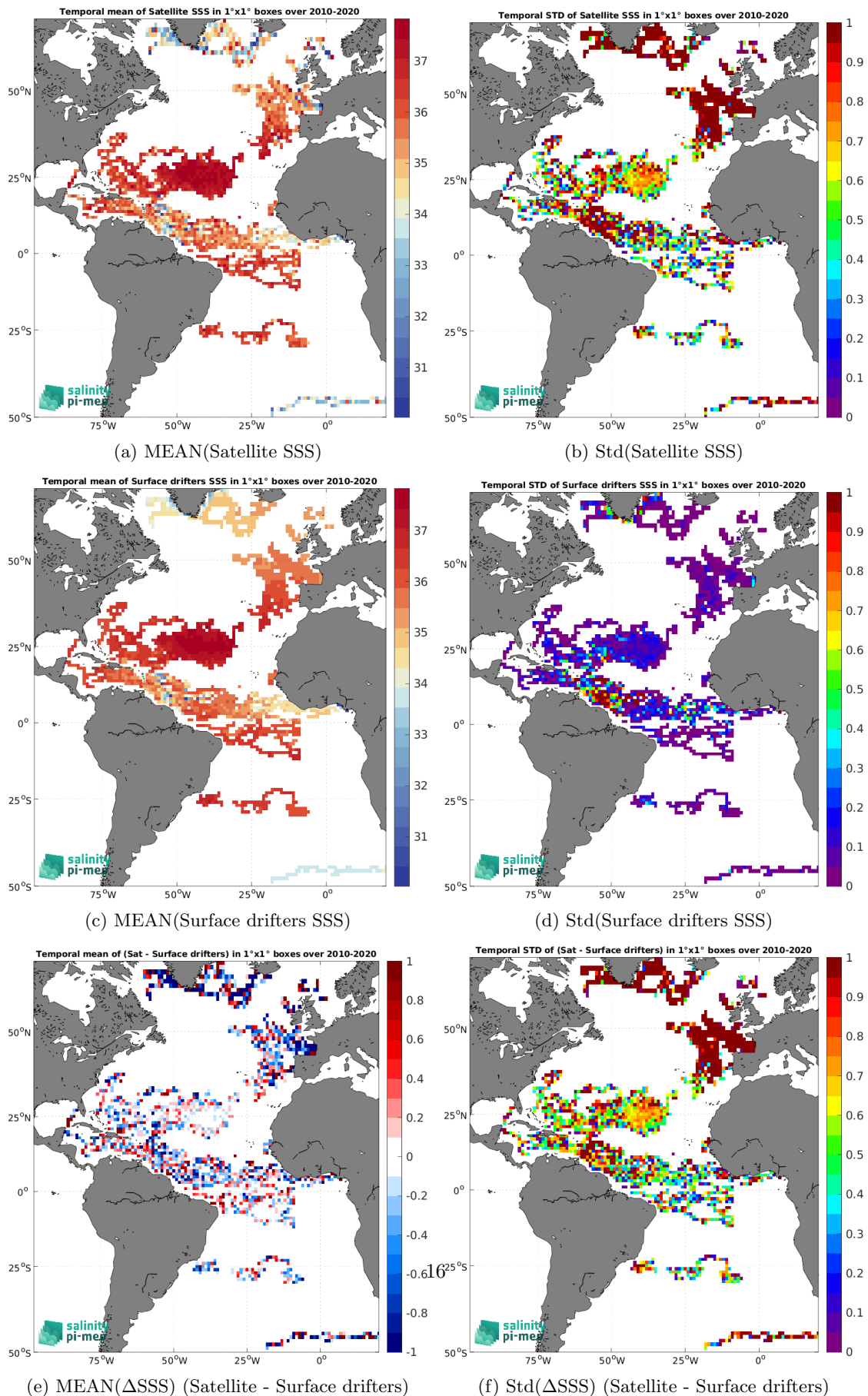
Figure 6: Temporal mean (left) and Std (right) of SSS from SMOS SSS L2Q v331 - No FLAG (CMEMS-CATDS-CPDC) (top), Surface drifters (middle), and of \Delta SSS (Satellite - Surface drifters). Only match-up pairs are used to generate these maps.
