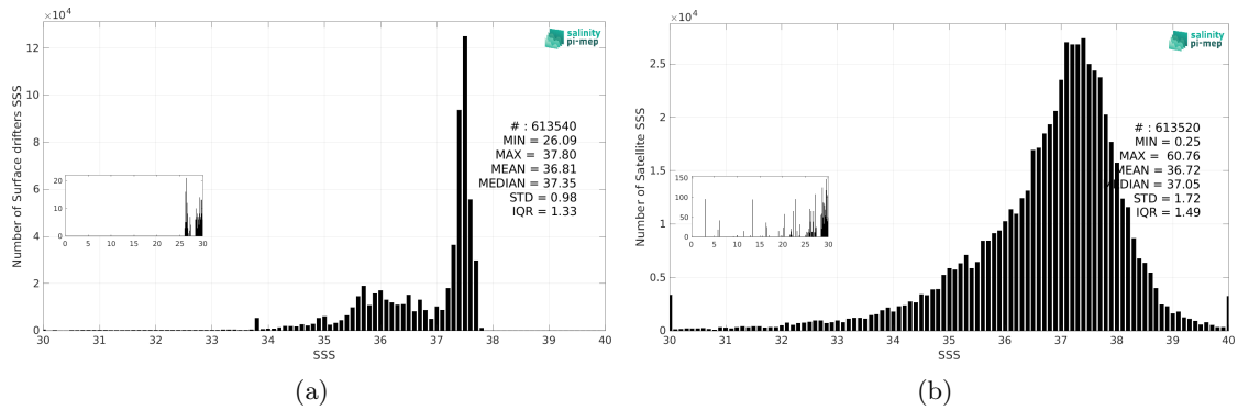
Figure 3: Histograms of SSS from Surface drifters (a) and SMOS SSS L2Q v331 - No FLAG (CMEMS-CATDS-CPDC) (b) considering all match-up pairs per bins of 0.1 over the Atlantic Ocean Pi-MEP region and for the full satellite product period.
