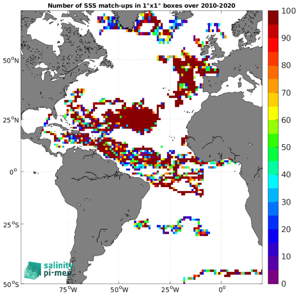
Figure 4: Number of SSS match-ups between Surface drifters SSS and the SMOS SSS L2Q v331 - No FLAG (CMEMS-CATDS-CPDC) SSS product for the Atlantic Ocean Pi-MEP region over 1^\circ \times 1^\circ boxes and for the full satellite product period.
