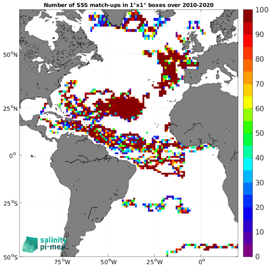
Figure 3: Number of SSS match-ups between Surface drifters SSS and the SMOS SSS L2Q v331 - No FLAG (CMEMS-CATDS-CPDC) SSS product for the Atlantic Ocean Pi-MEP region over 1°×1° boxes and for the full satellite product period.
