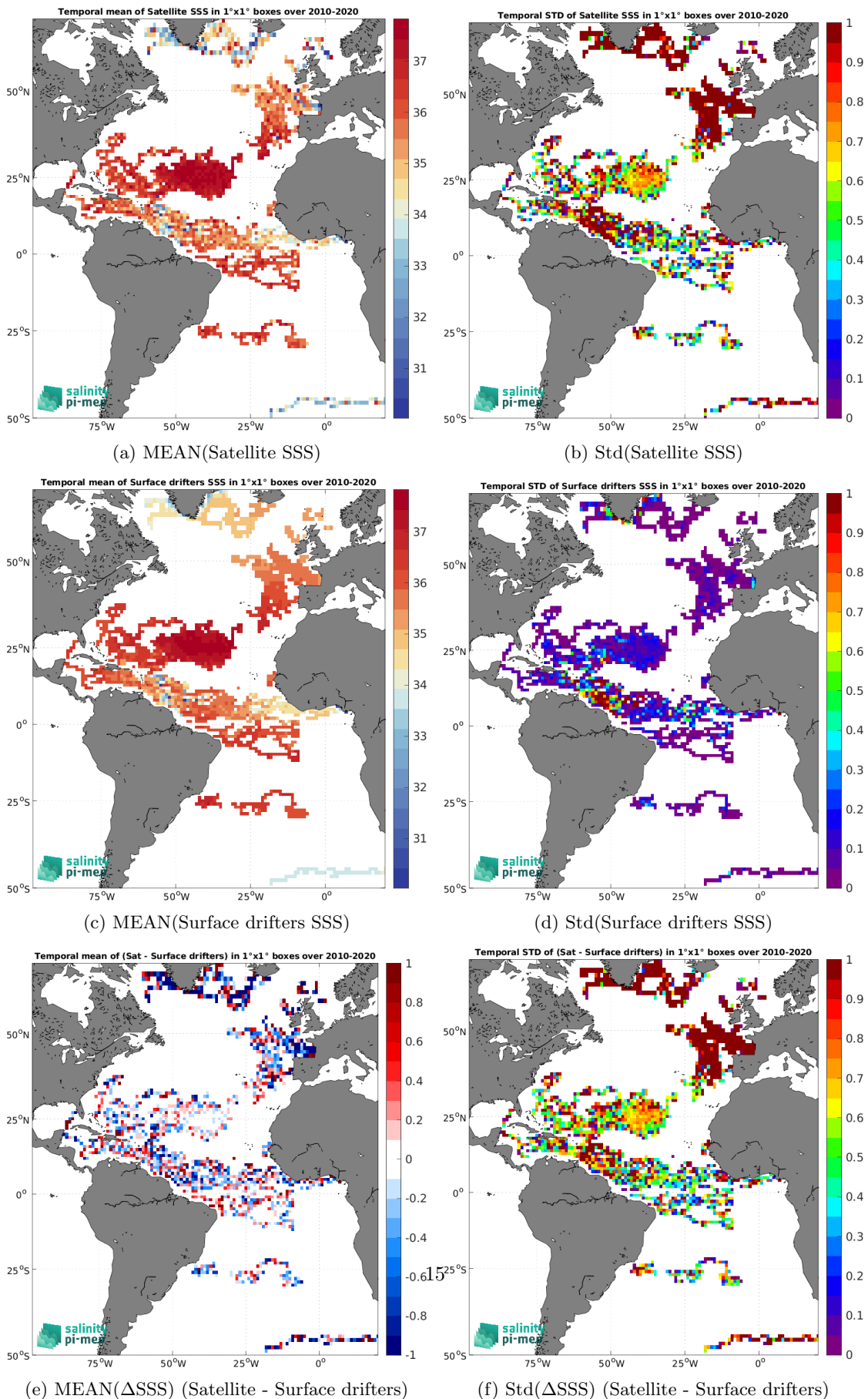
Figure 5: Temporal mean (left) and Std (right) of SSS from SMOS SSS L2Q v331 - No FLAG (CMEMS-CATDS-CPDC) (top), Surface drifters (middle), and of \Delta SSS (Satellite - Surface drifters). Only match-up pairs are used to generate these maps.
