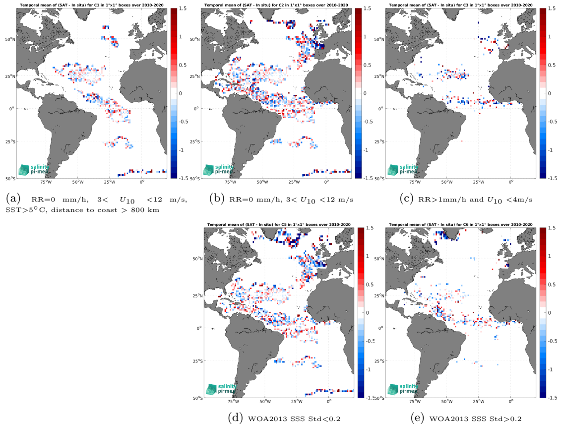
Figure 11: Temporal mean gridded over spatial boxes of size 1^\circ \times 1^\circ of \Delta\text{SSS} (SMOS SSS L2Q v331 - No FLAG (CMEMS-CATDS-CPDC) - Surface drifters) for 5 different subdatasets corresponding to:RR=0 mm/h, 3 < U_{10} < 12 m/s, SST >5^\circ\text{C} , distance to coast > 800 km (a), RR=0 mm/h, 3 < U_{10} < 12 m/s (b), RR >1 mm/h and U_{10} < 4 m/s (c), WOA2013 SSS Std <0.2 (d), WOA2013 SSS Std >0.2 (e).
