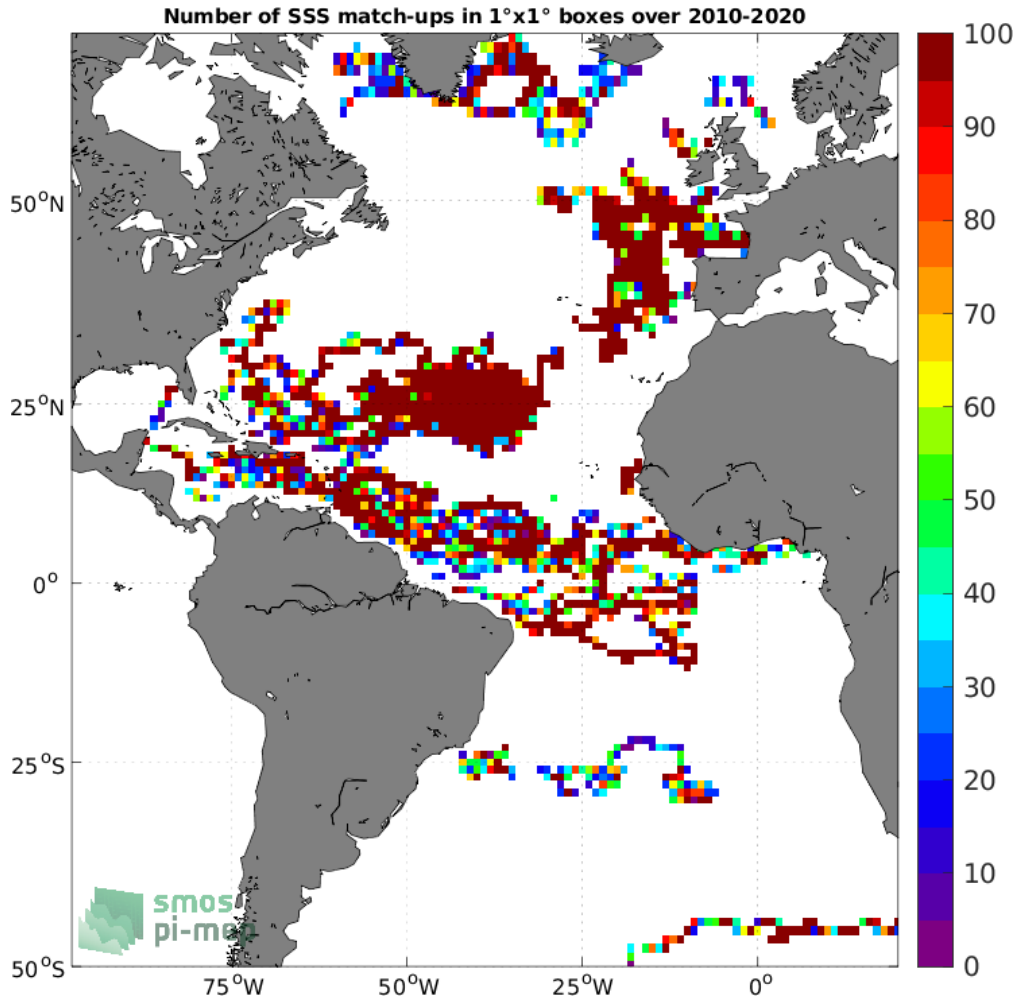
Figure 3: Number of SSS match-ups between Surface drifters SSS and the SMOS SSS L2Q v331 - No FLAG (CMEMS-CATDS-CPDC) SSS product for the Atlantic Ocean Pi-MEP region over 1^\circ \times 1^\circ boxes and for the full satellite product period.
