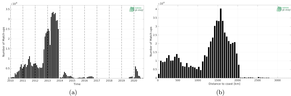
Figure 1: Number of match-ups between Surface drifters and SMOS SSS L2Q v331 - No FLAG (CMEMS-CATDS-CPDC) SSS as a function of time (a) and as function of the distance to coast (b) over the Atlantic Ocean Pi-MEP region and for the full satellite product period.
