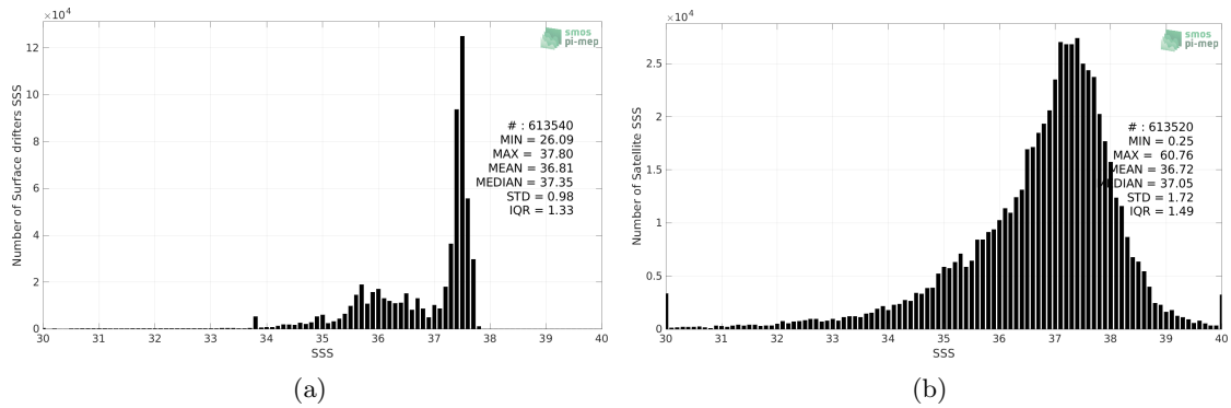
Figure 2: Histograms of SSS from Surface drifters (a) and SMOS SSS L2Q v331 - No FLAG (CMEMS-CATDS-CPDC) (b) considering all match-up pairs per bins of 0.1 over the Atlantic Ocean Pi-MEP region and for the full satellite product period.
