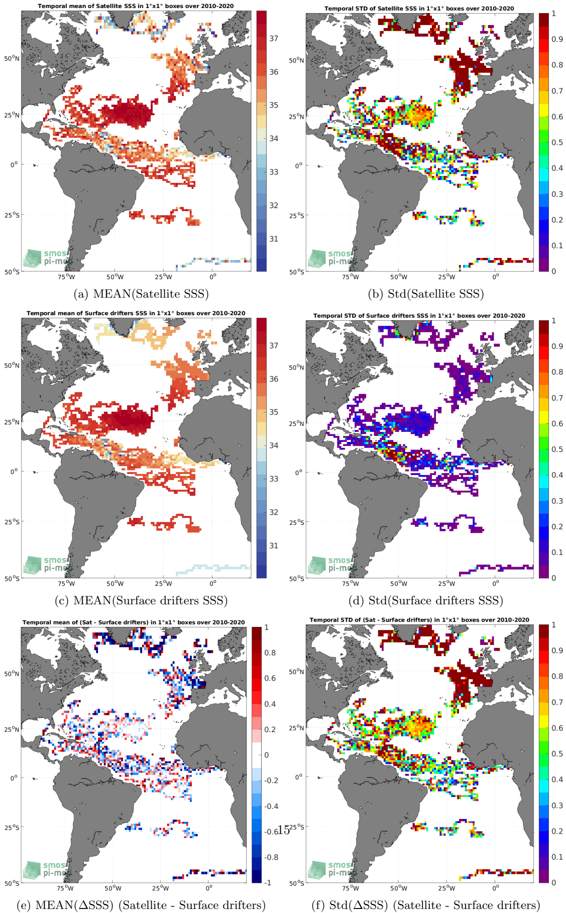
(e) MEAN( \Delta SSS) (Satellite - Surface drifters) (f) Std( \Delta SSS) (Satellite - Surface drifters) Figure 5: Temporal mean (left) and Std (right) of SSS from SMOS SSS L2Q v331 - No FLAG (CMEMS-CATDS-CPDC) (top), Surface drifters (middle), and of \Delta SSS (Satellite - Surface drifters). Only match-up pairs are used to generate these maps.
