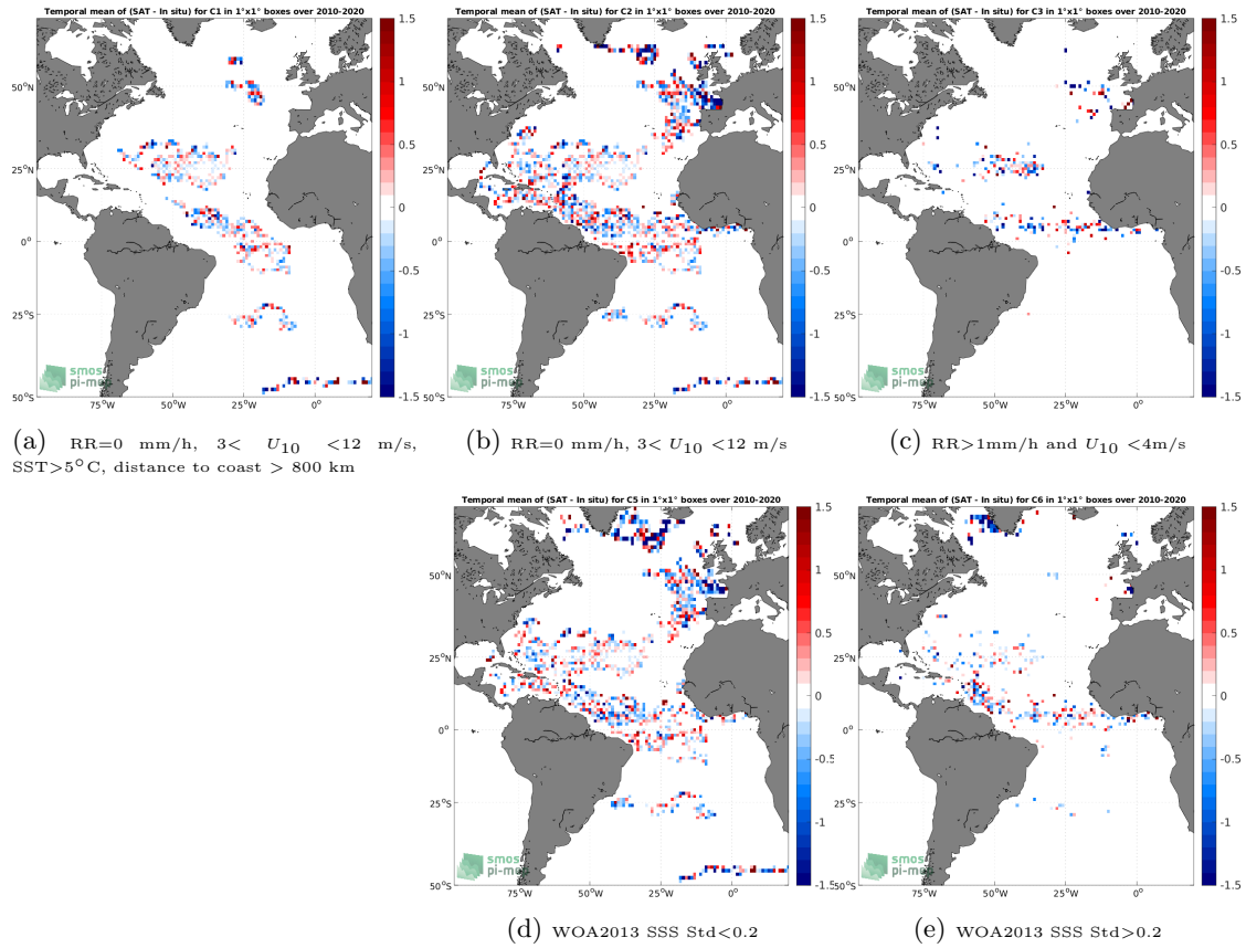
Figure 11: Temporal mean gridded over spatial boxes of size 1^\circ \times 1^\circ of \Delta\text{SSS} (SMOS SSS L2Q v331 - No FLAG (CMEMS-CATDS-CPDC) - Surface drifters) for 5 different subdatasets corresponding to:RR=0 mm/h, 3 < U_{10} < 12 m/s, SST >5^\circ\text{C} , distance to coast > 800 km (a), RR=0 mm/h, 3 < U_{10} < 12 m/s (b), RR >1 mm/h and U_{10} < 4 m/s (c), WOA2013 SSS Std <0.2 (d), WOA2013 SSS Std >0.2 (e).
