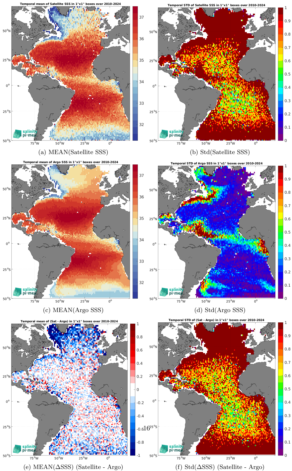
Figure 7: Temporal mean (left) and Std (right) of SSS from SMOS SSS L2Q v331 - No FLAG (CMEMS-CATDS-CPDC) (top), Argo (middle), and of \Delta SSS (Satellite - Argo). Only match-up pairs are used to generate these maps.
