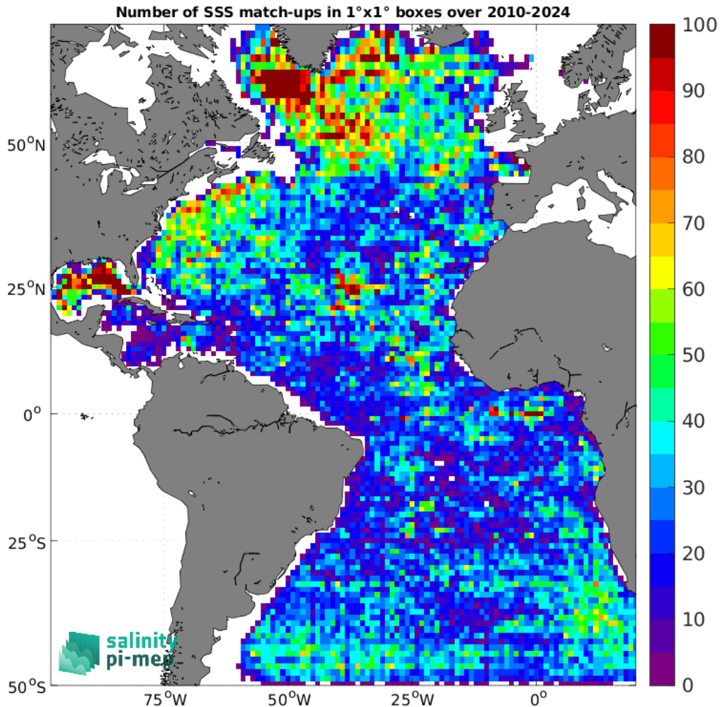
Figure 5: Number of SSS match-ups between Argo SSS and the SMOS SSS L2Q v331 - No FLAG (CMEMS-CATDS-CPDC) SSS product for the Atlantic Ocean Pi-MEP region over 1^\circ \times 1^\circ boxes and for the full satellite product period.
