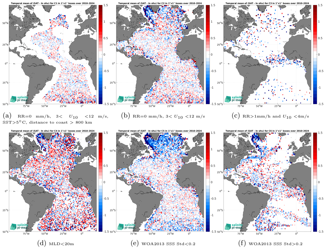
Figure 14: Temporal mean gridded over spatial boxes of size 1^\circ \times 1^\circ of \Delta SSS (SMOS SSS L2Q v331 - No FLAG (CMEMS-CATDS-CPDC) - Argo) for 6 different subdatasets corresponding to:RR=0 mm/h, 3 < U_{10} < 12 m/s, SST>5°C, distance to coast > 800 km (a), RR=0 mm/h, 3 < U_{10} < 12 m/s (b), RR>1mm/h and U_{10} < 4 m/s (c),MLD<20m (d),WOA2013 SSS Std<0.2 (e),WOA2013 SSS Std>0.2 (f).
