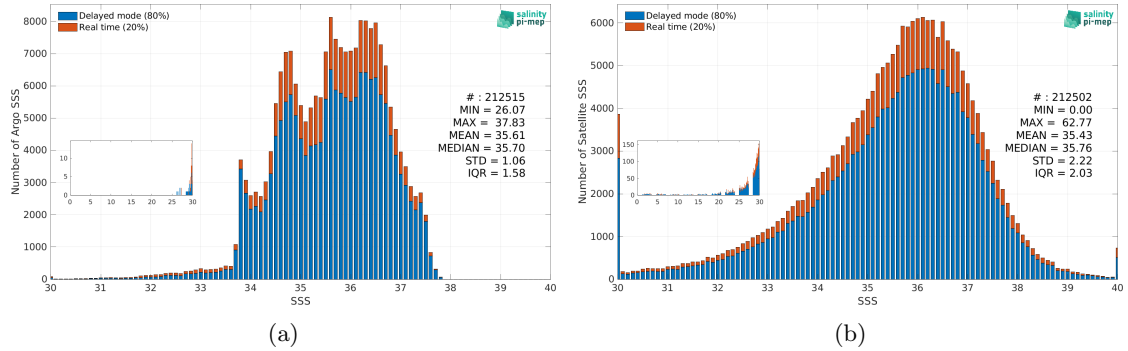
Figure 3: Histograms of SSS from Argo (a) and SMOS SSS L2Q v331 - No FLAG (CMEMS-CATDS-CPDC) (b) considering all match-up pairs per bins of 0.1 over the Atlantic Ocean Pi-MEP region and for the full satellite product period.
