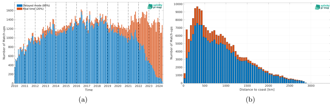
Figure 2: Number of match-ups between Argo and SMOS SSS L2Q v331 - No FLAG (CMEMS-CATDS-CPDC) SSS as a function of time (a) and as function of the distance to coast (b) over the Atlantic Ocean Pi-MEP region and for the full satellite product period.
