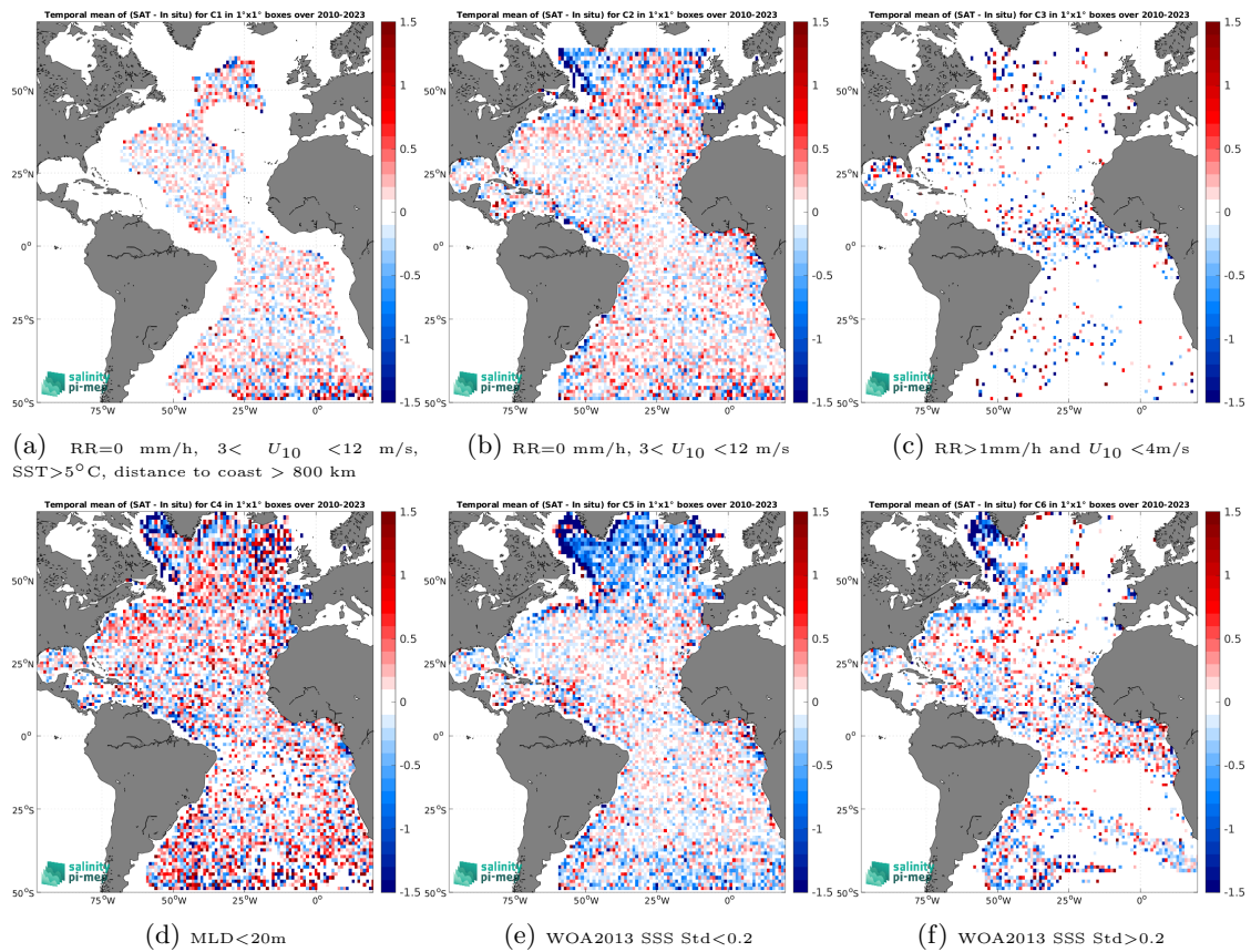
Figure 12: Temporal mean gridded over spatial boxes of size 1^\circ \times 1^\circ of \Delta SSS (SMOS SSS L2Q v331 - No FLAG (CMEMS-CATDS-CPDC) - Argo) for 6 different subdatasets corresponding to:RR=0 mm/h, 3 < U_{10} < 12 m/s, SST >5^\circ C, distance to coast > 800 km (a), RR=0 mm/h, 3 < U_{10} < 12 m/s (b), RR >1 mm/h and U_{10} < 4 m/s (c),MLD <20 m (d),WOA2013 SSS Std <0.2 (e),WOA2013 SSS Std >0.2 (f).
