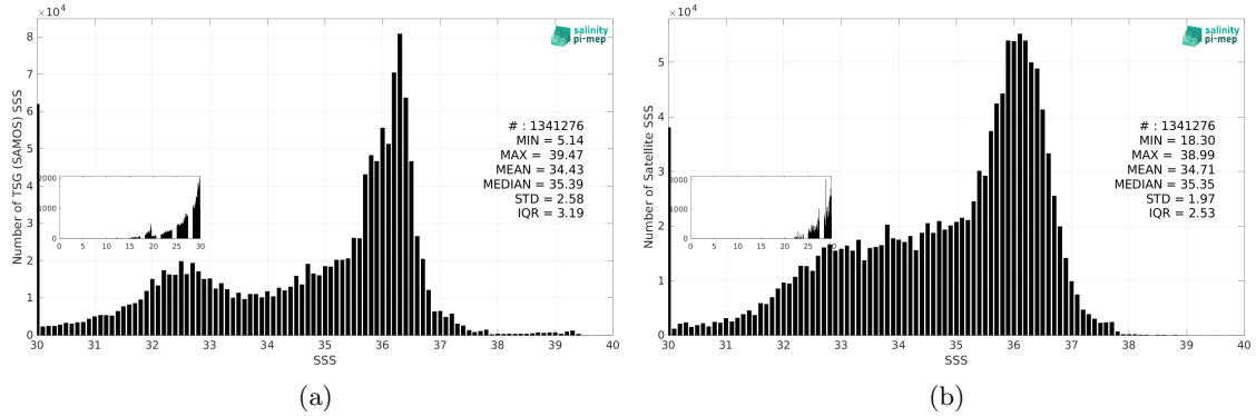
Figure 3: Histograms of SSS from TSG (SAMOS) (a) and SMOS SSS L3 v9 - 9 Days (CATDS-CEC-LOCEAN) (b) considering all match-up pairs per bins of 0.1 over the Atlantic Ocean Pi-MEP region and for the full satellite product period.
