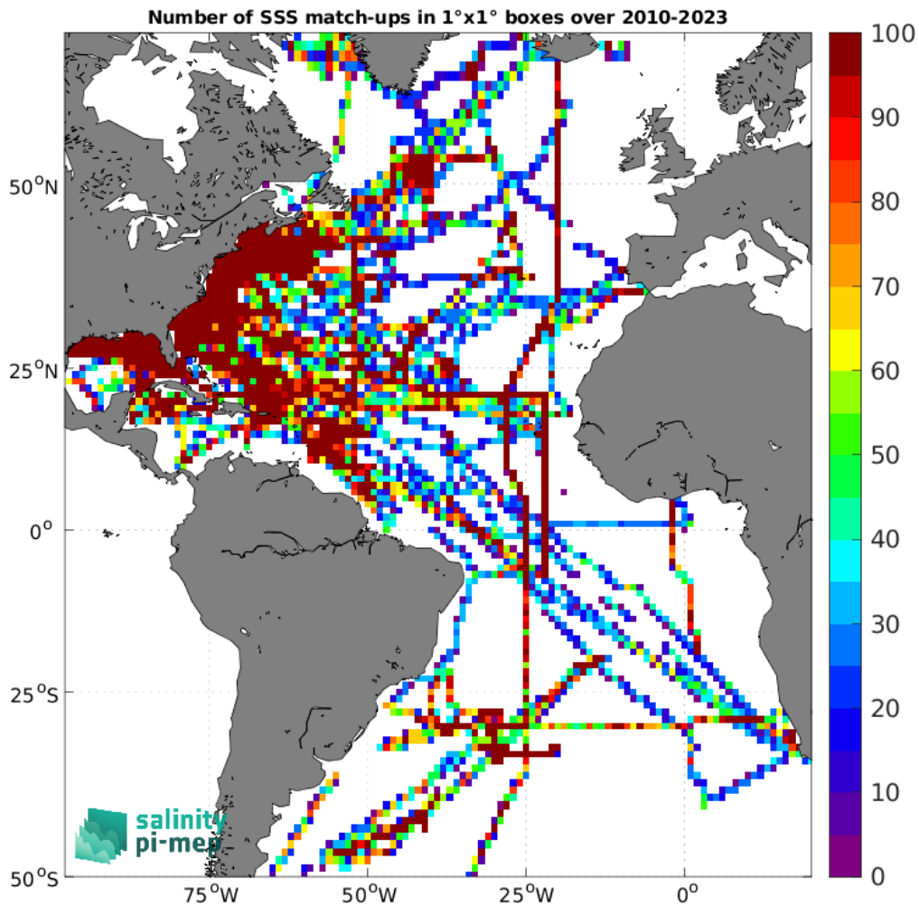
Figure 5: Number of SSS match-ups between TSG (SAMOS) SSS and the SMOS SSS L3 v9 - 9 Days (CATDS-CEC-LOCEAN) SSS product for the Atlantic Ocean Pi-MEP region over 1^\circ \times 1^\circ boxes and for the full satellite product period.
