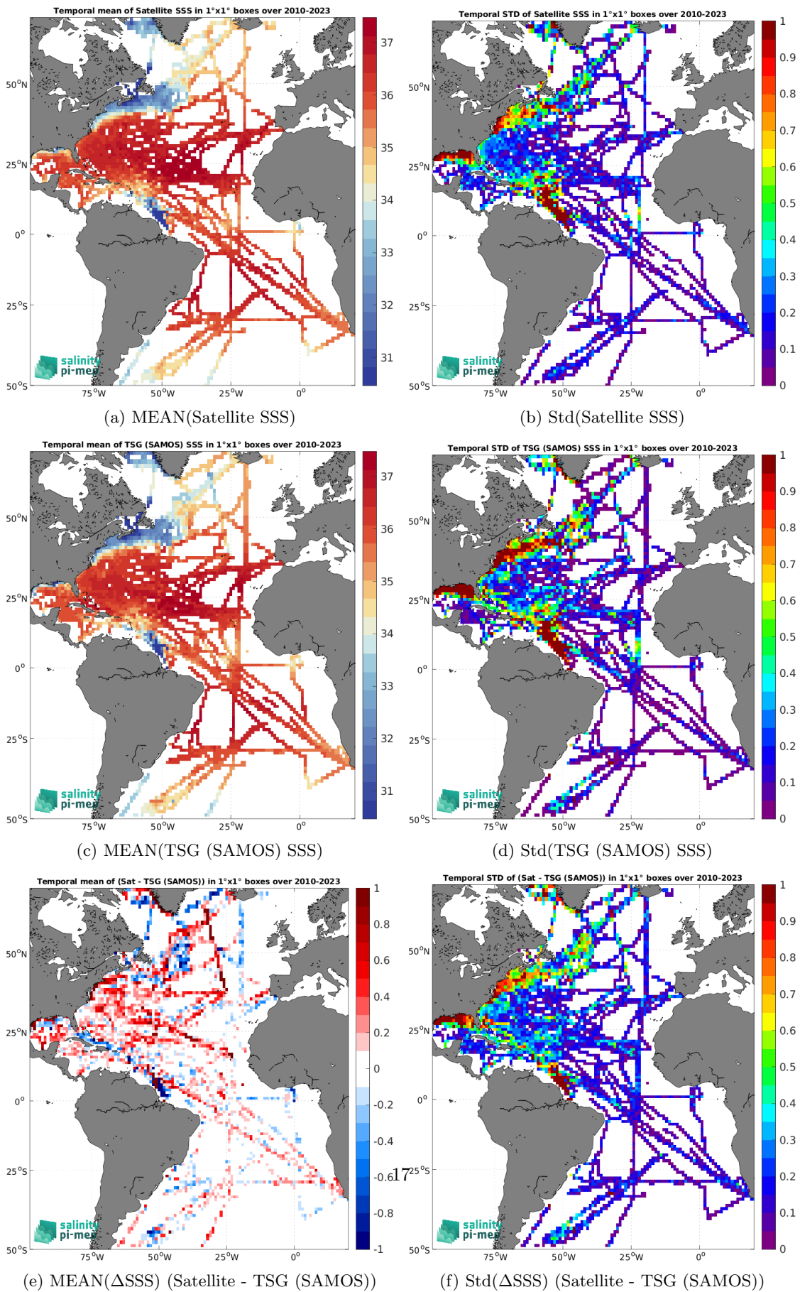
Figure 7: Temporal mean (left) and Std (right) of SSS from SMOS SSS L3 v9 - 9 Days (CATDS-CEC-LOCEAN) (top), TSG (SAMOS) (middle), and of \Delta SSS (Satellite - TSG (SAMOS)). Only match-up pairs are used to generate these maps.
