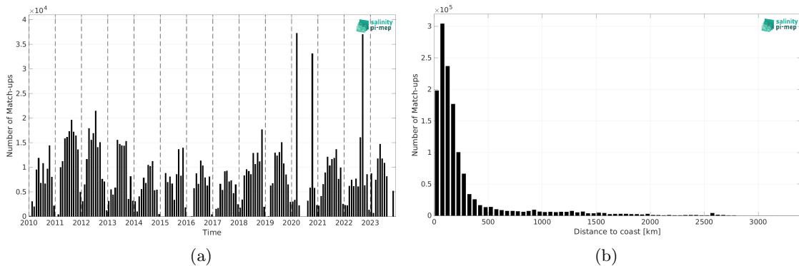
Figure 2: Number of match-ups between TSG (SAMOS) and SMOS SSS L3 v9 - 9 Days (CATDS-CEC-LOCEAN) SSS as a function of time (a) and as function of the distance to coast (b) over the Atlantic Ocean Pi-MEP region and for the full satellite product period.
