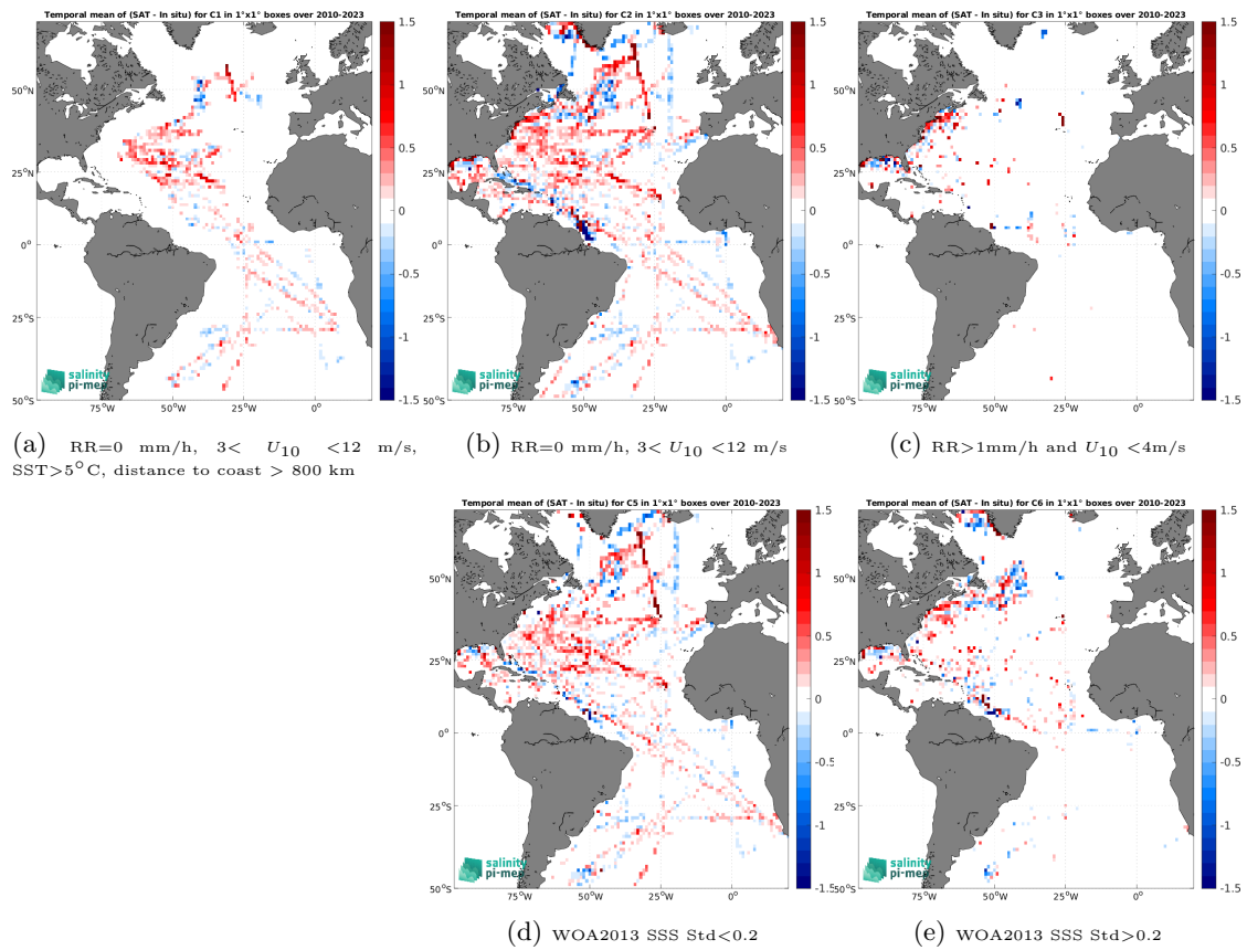
Figure 14: Temporal mean gridded over spatial boxes of size 1^\circ \times 1^\circ of \Delta\text{SSS} (SMOS SSS L3 v9 - 9 Days (CATDS-CEC-LOCEAN) - TSG (SAMOS)) for 5 different subdatasets corresponding to:RR=0 mm/h, 3 < U_{10} < 12 m/s, SST >5^\circ\text{C} , distance to coast > 800 km (a), RR=0 mm/h, 3 < U_{10} < 12 m/s (b), RR >1 mm/h and U_{10} < 4 m/s (c), WOA2013 SSS Std <0.2 (d), WOA2013 SSS Std >0.2 (e).
