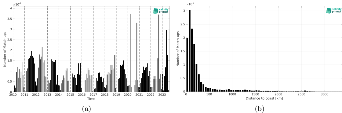
Figure 1: Number of match-ups between TSG (SAMOS) and SMOS SSS L3 v9 - 9 Days (CATDS-CEC-LOCEAN) SSS as a function of time (a) and as function of the distance to coast (b) over the Atlantic Ocean Pi-MEP region and for the full satellite product period.
