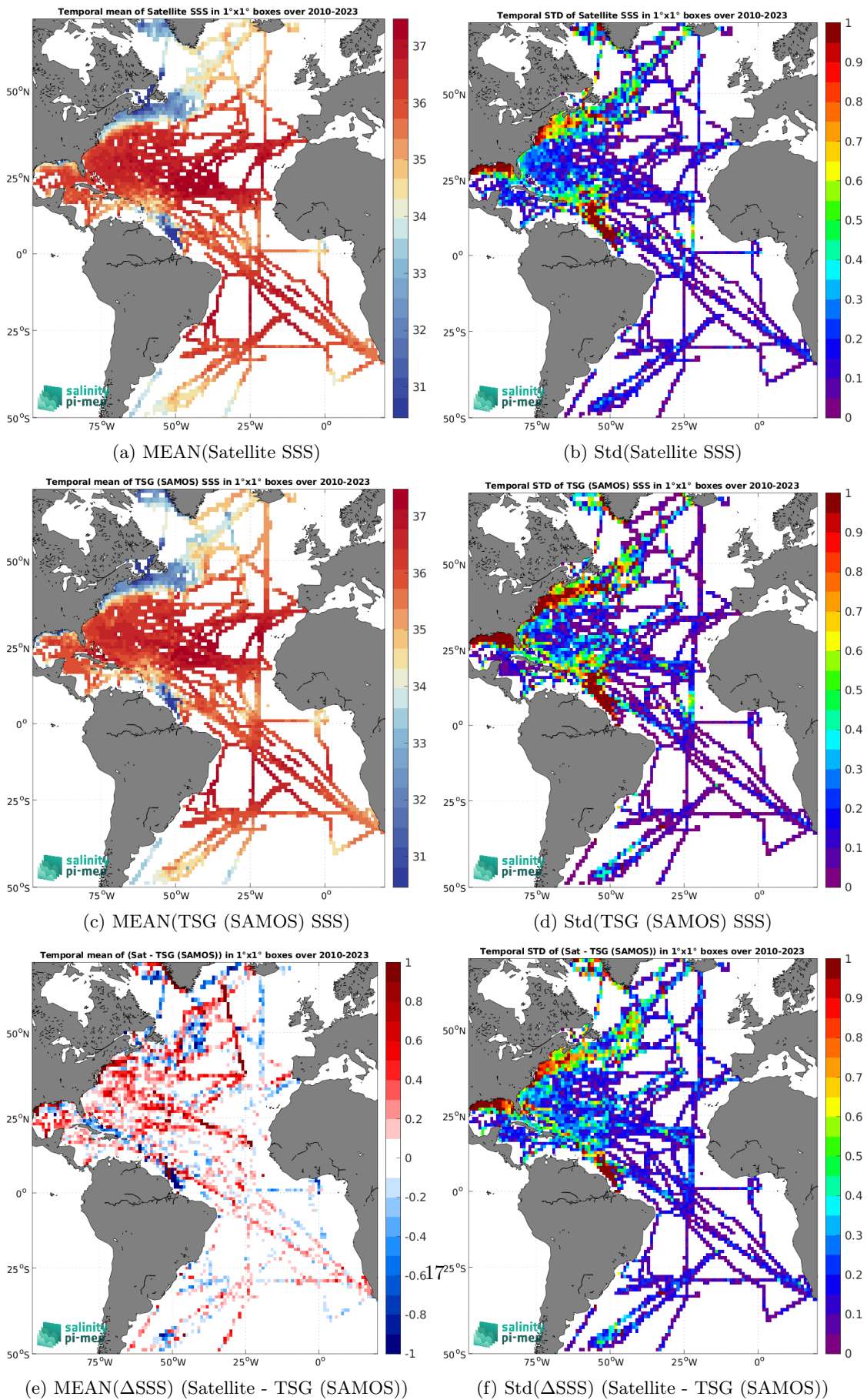
Figure 6: Temporal mean (left) and Std (right) of SSS from SMOS SSS L3 v9 - 9 Days (CATDS-CEC-LOCEAN) (top), TSG (SAMOS) (middle), and of \Delta SSS (Satellite - TSG (SAMOS)). Only match-up pairs are used to generate these maps.
