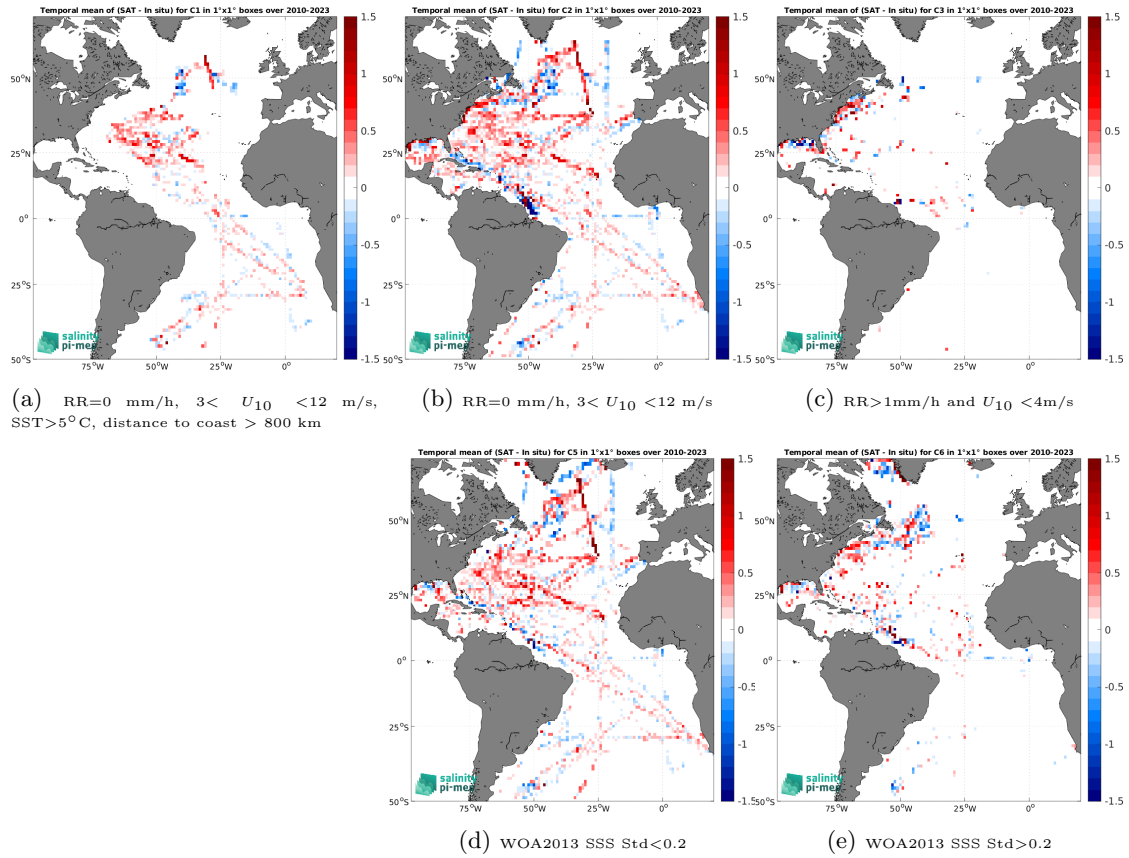
Figure 12: Temporal mean gridded over spatial boxes of size 1^\circ \times 1^\circ of \Delta SSS (SMOS SSS L3 v9 - 9 Days (CATDS-CEC-LOCEAN) - TSG (SAMOS)) for 5 different subdatasets corresponding to:RR=0 mm/h, 3 < U_{10} < 12 m/s, SST >5^\circ\text{C} , distance to coast > 800 km (a), RR=0 mm/h, 3 < U_{10} < 12 m/s (b), RR >1 mm/h and U_{10} < 4 m/s (c), WOA2013 SSS Std <0.2 (d), WOA2013 SSS Std >0.2 (e).
