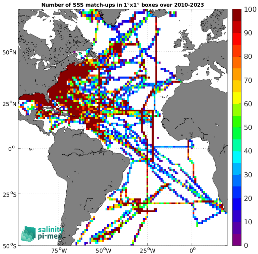
Figure 4: Number of SSS match-ups between TSG (SAMOS) SSS and the SMOS SSS L3 v9 - 9 Days (CATDS-CEC-LOCEAN) SSS product for the Atlantic Ocean Pi-MEP region over 1^\circ \times 1^\circ boxes and for the full satellite product period.
