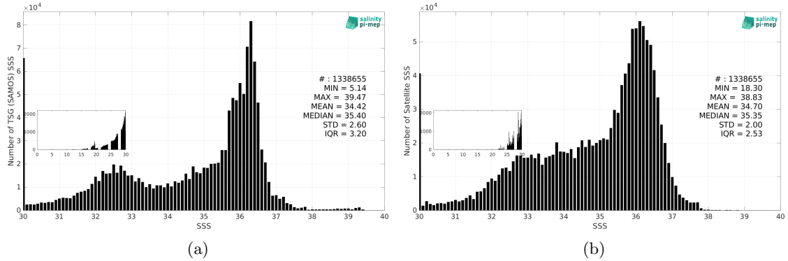
Figure 2: Histograms of SSS from TSG (SAMOS) (a) and SMOS SSS L3 v9 - 9 Days (CATDS-CEC-LOCEAN) (b) considering all match-up pairs per bins of 0.1 over the Atlantic Ocean Pi-MEP region and for the full satellite product period.
