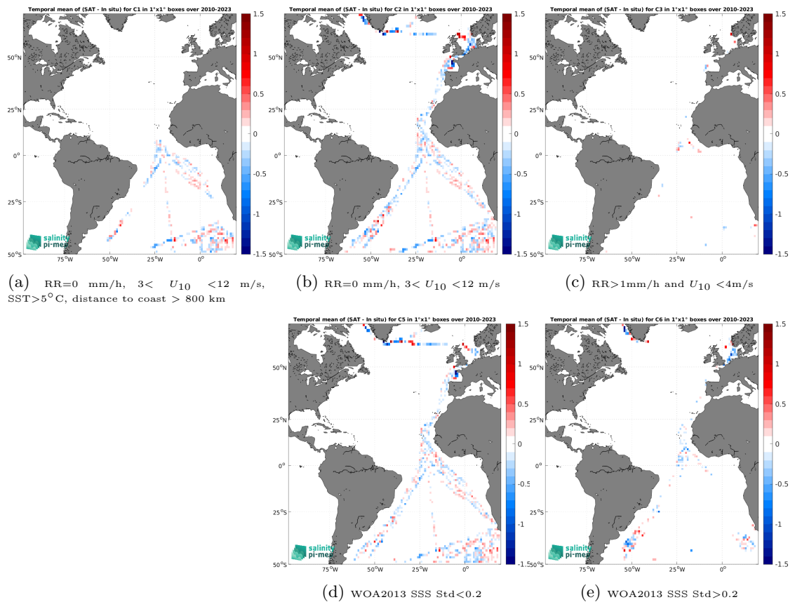
Figure 14: Temporal mean gridded over spatial boxes of size 1^\circ \times 1^\circ of \Delta\text{SSS} (SMOS SSS L3 v9 - 9 Days (CATDS-CEC-LOCEAN) - TSG (Polarstern)) for 5 different subdatasets corresponding to:RR=0 mm/h, 3 < U_{10} < 12 m/s, SST>5°C, distance to coast > 800 km (a), RR=0 mm/h, 3 < U_{10} < 12 m/s (b), RR>1mm/h and U_{10} < 4 m/s (c), WOA2013 SSS Std<0.2 (d), WOA2013 SSS Std>0.2 (e).
