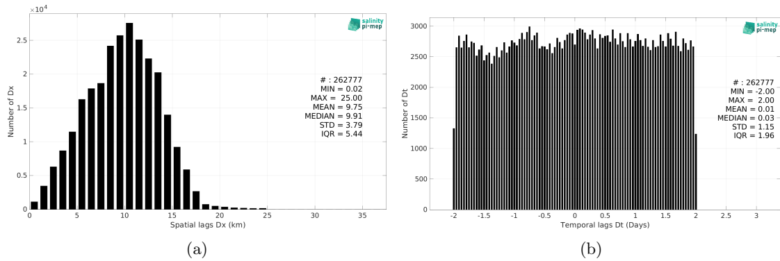
Figure 5: Histograms of the spatial (a) and temporal (b) lags between the location/time of the TSG (Polarstern) measurement and the date of the corresponding SMOS SSS L3 v9 - 9 Days (CATDS-CEC-LOCEAN) SSS pixel.
