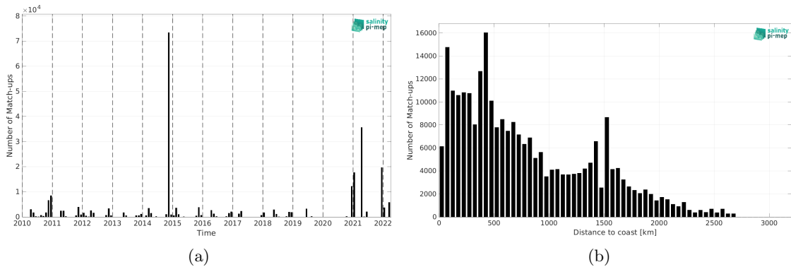
Figure 1: Number of match-ups between TSG (Polarstern) and SMOS SSS L3 v9 - 9 Days (CATDS-CEC-LOCEAN) SSS as a function of time (a) and as function of the distance to coast (b) over the Atlantic Ocean Pi-MEP region and for the full satellite product period.
