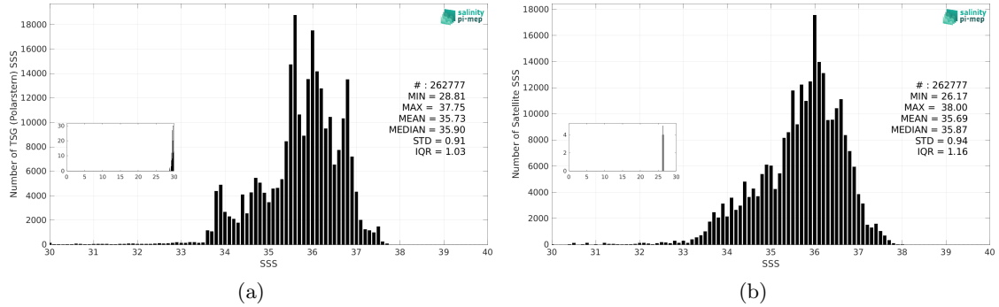
Figure 2: Histograms of SSS from TSG (Polarstern) (a) and SMOS SSS L3 v9 - 9 Days (CATDS-CEC-LOCEAN) (b) considering all match-up pairs per bins of 0.1 over the Atlantic Ocean Pi-MEP region and for the full satellite product period.
