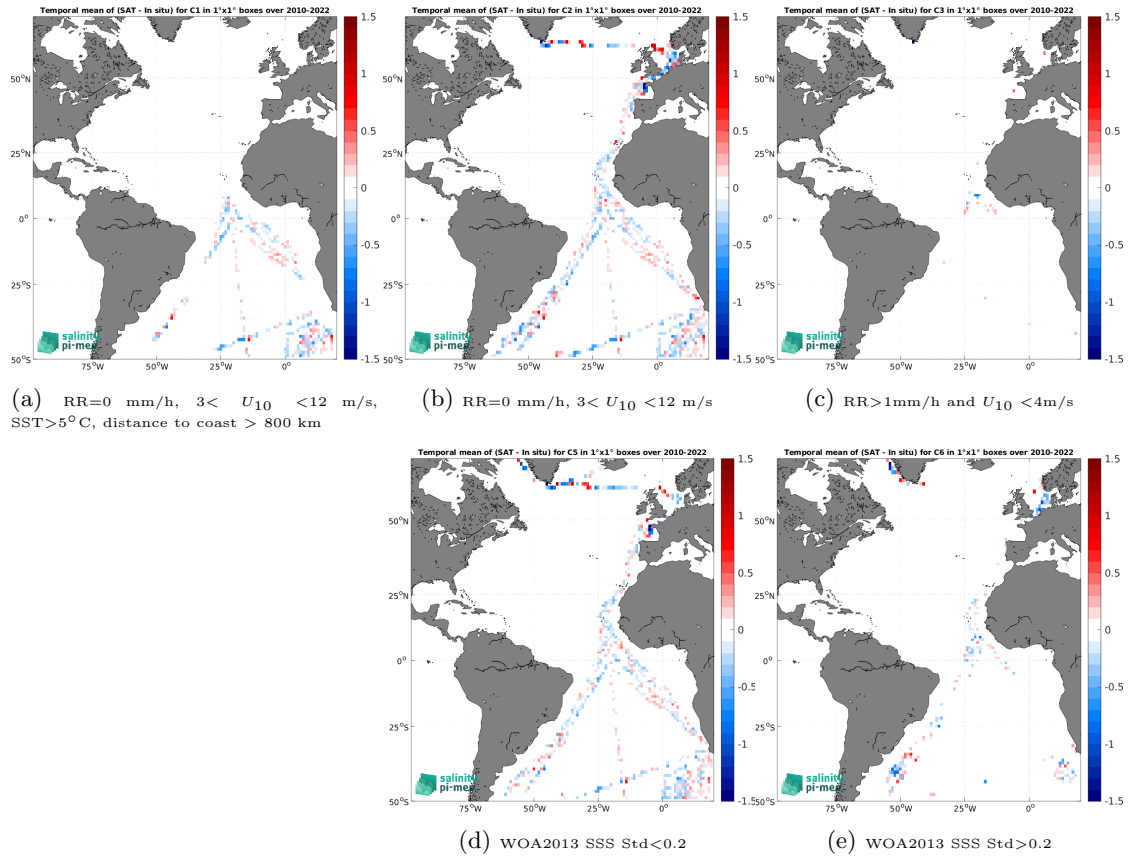
Figure 12: Temporal mean gridded over spatial boxes of size 1^\circ \times 1^\circ of \Delta SSS (SMOS SSS L3 v9 - 9 Days (CATDS-CEC-LOCEAN) - TSG (Polarstern)) for 5 different subdatasets corresponding to:RR=0 mm/h, 3 < U_{10} < 12 m/s, SST >5^\circ\text{C} , distance to coast > 800 km (a), RR=0 mm/h, 3 < U_{10} < 12 m/s (b), RR >1 mm/h and U_{10} < 4 m/s (c), WOA2013 SSS Std <0.2 (d), WOA2013 SSS Std >0.2 (e).
