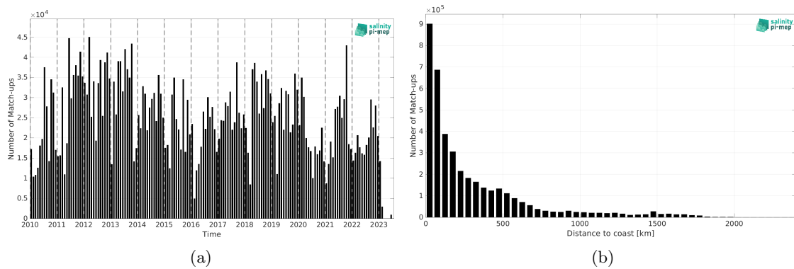
Figure 2: Number of match-ups between TSG (LEGOS-DM) and SMOS SSS L3 v9 - 9 Days (CATDS-CEC-LOCEAN) SSS as a function of time (a) and as function of the distance to coast (b) over the Atlantic Ocean Pi-MEP region and for the full satellite product period.
