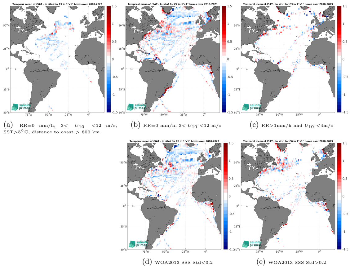
Figure 14: Temporal mean gridded over spatial boxes of size 1^\circ \times 1^\circ of \Delta SSS (SMOS SSS L3 v9 - 9 Days (CATDS-CEC-LOCEAN) - TSG (LEGOS-DM)) for 5 different subdatasets corresponding to:RR=0 mm/h, 3 < U_{10} < 12 m/s, SST >5^\circ\text{C} , distance to coast > 800 km (a), RR=0 mm/h, 3 < U_{10} < 12 m/s (b), RR >1 mm/h and U_{10} < 4 m/s (c), WOA2013 SSS Std <0.2 (d), WOA2013 SSS Std >0.2 (e).
