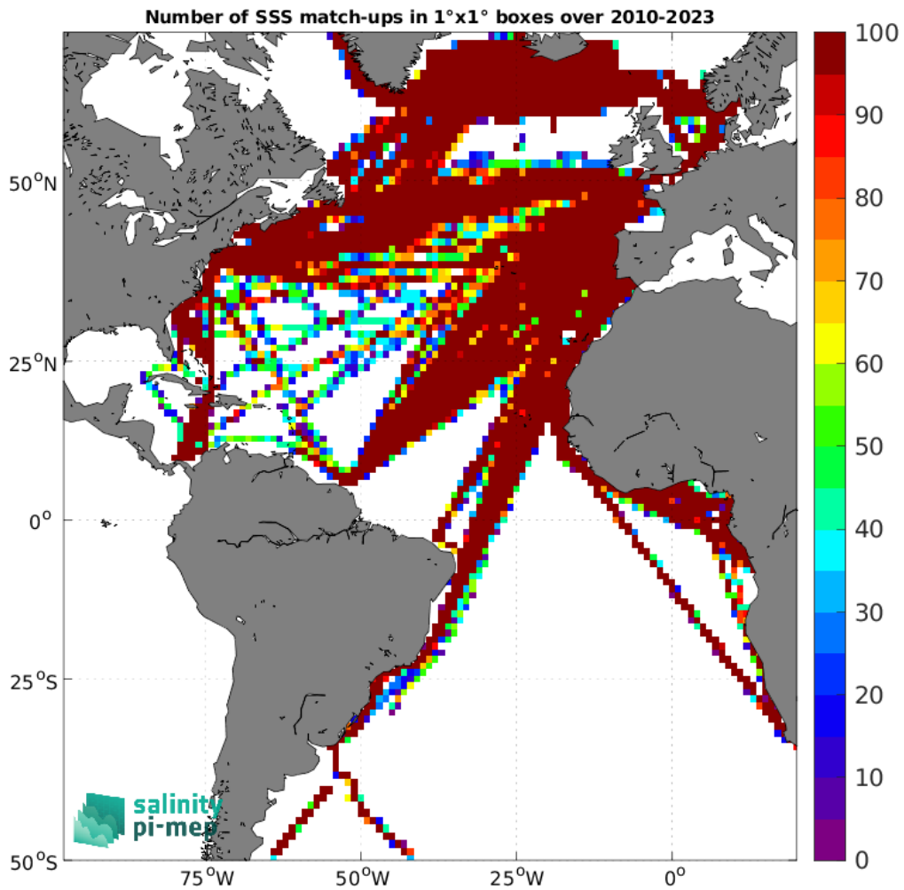
Figure 5: Number of SSS match-ups between TSG (LEGOS-DM) SSS and the SMOS SSS L3 v9 - 9 Days (CATDS-CEC-LOCEAN) SSS product for the Atlantic Ocean Pi-MEP region over 1^\circ \times 1^\circ boxes and for the full satellite product period.
