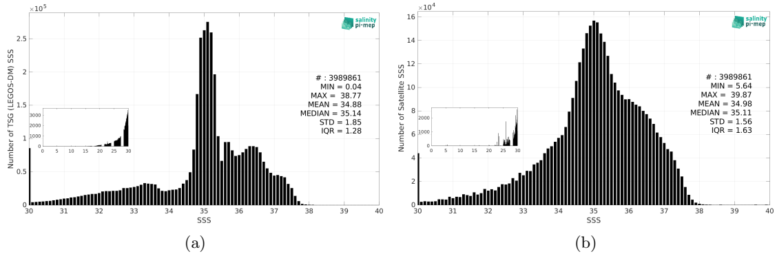
Figure 3: Histograms of SSS from TSG (LEGOS-DM) (a) and SMOS SSS L3 v9 - 9 Days (CATDS-CEC-LOCEAN) (b) considering all match-up pairs per bins of 0.1 over the Atlantic Ocean Pi-MEP region and for the full satellite product period.
