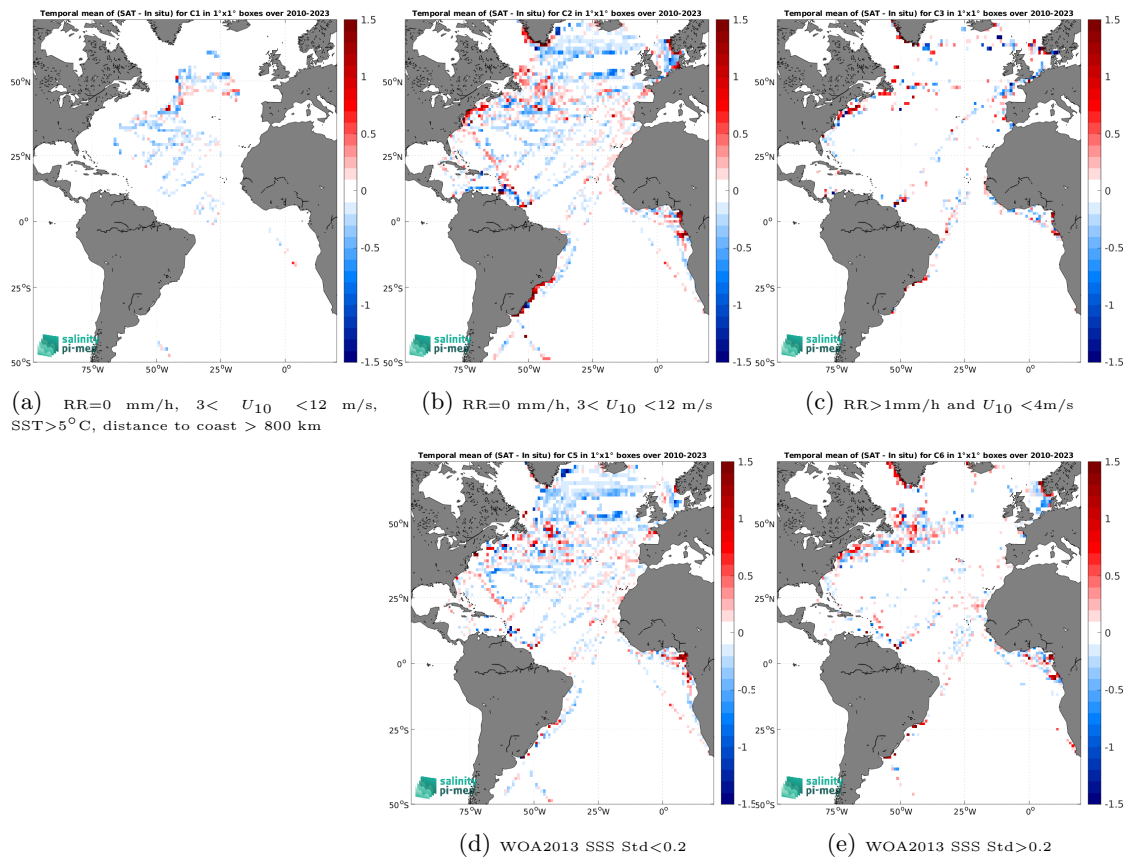
Figure 14: Temporal mean gridded over spatial boxes of size 1^\circ \times 1^\circ of \Delta\text{SSS} (SMOS SSS L3 v9 - 9 Days (CATDS-CEC-LOCEAN) - TSG (LEGOS-DM)) for 5 different subdatasets corresponding to:RR=0 mm/h, 3 < U_{10} < 12 m/s, SST >5^\circ\text{C} , distance to coast > 800 km (a), RR=0 mm/h, 3 < U_{10} < 12 m/s (b), RR >1 mm/h and U_{10} < 4 m/s (c), WOA2013 SSS Std <0.2 (d), WOA2013 SSS Std >0.2 (e).
