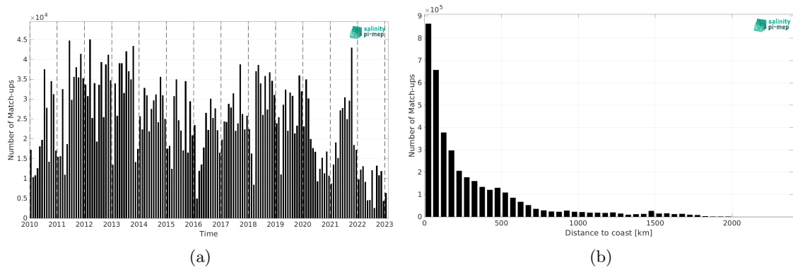
Figure 1: Number of match-ups between TSG (LEGOS-DM) and SMOS SSS L3 v9 - 9 Days (CATDS-CEC-LOCEAN) SSS as a function of time (a) and as function of the distance to coast (b) over the Atlantic Ocean Pi-MEP region and for the full satellite product period.
