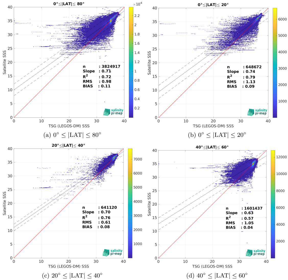
Figure 9: Contour maps of the concentration of SMOS SSS L3 v9 - 9 Days (CATDS-CEC-LOCEAN) SSS (y-axis) versus TSG (LEGOS-DM) SSS (x-axis) at match-up pairs for different latitude bands. For each plot, the red line shows x=y . The black thin and dashed lines indicate a linear fit through the data cloud and the \pm 95\% confidence levels, respectively. The number match-up pairs n , the slope and R^2 coefficient of the linear fit, the root mean square (RMS) and the mean bias between satellite and in situ data are indicated for each latitude band in each plots.
