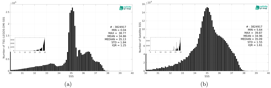
Figure 2: Histograms of SSS from TSG (LEGOS-DM) (a) and SMOS SSS L3 v9 - 9 Days (CATDS-CEC-LOCEAN) (b) considering all match-up pairs per bins of 0.1 over the Atlantic Ocean Pi-MEP region and for the full satellite product period.
