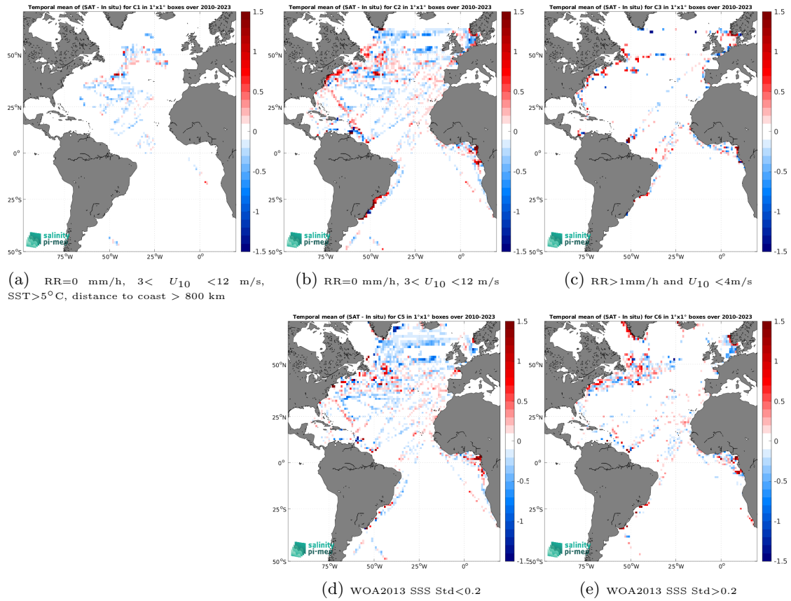
Figure 12: Temporal mean gridded over spatial boxes of size 1^\circ \times 1^\circ of \Delta SSS (SMOS SSS L3 v9 - 9 Days (CATDS-CEC-LOCEAN) - TSG (LEGOS-DM)) for 5 different subdatasets corresponding to:RR=0 mm/h, 3 < U_{10} < 12 m/s, SST >5^\circ\text{C} , distance to coast > 800 km (a), RR=0 mm/h, 3 < U_{10} < 12 m/s (b), RR >1 mm/h and U_{10} < 4 m/s (c), WOA2013 SSS Std <0.2 (d), WOA2013 SSS Std >0.2 (e).
