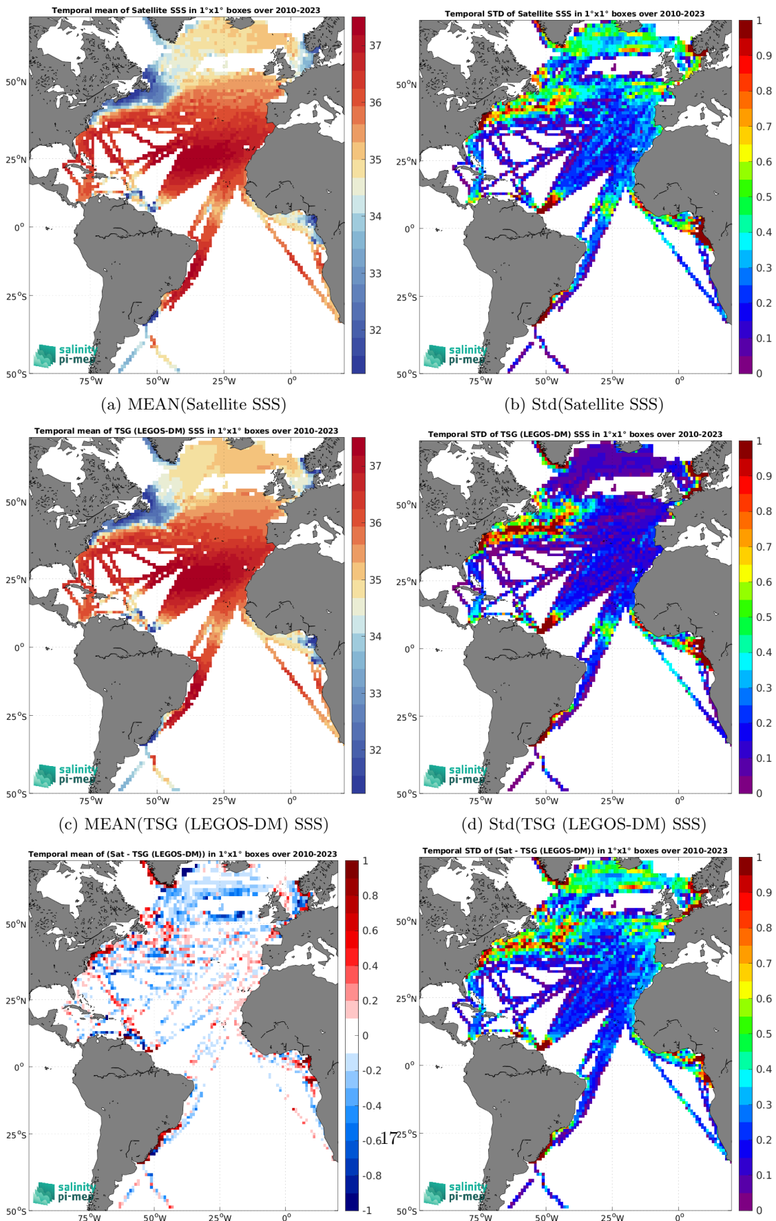
(e) MEAN( \Delta SSS) (Satellite - TSG (LEGOS-DM)) (f) Std( \Delta SSS) (Satellite - TSG (LEGOS-DM)) Figure 6: Temporal mean (left) and Std (right) of SSS from SMOS SSS L3 v9 - 9 Days (CATDS-CEC-LOCEAN) (top), TSG (LEGOS-DM) (middle), and of \Delta SSS (Satellite - TSG (LEGOS-DM)). Only match-up pairs are used to generate these maps.
